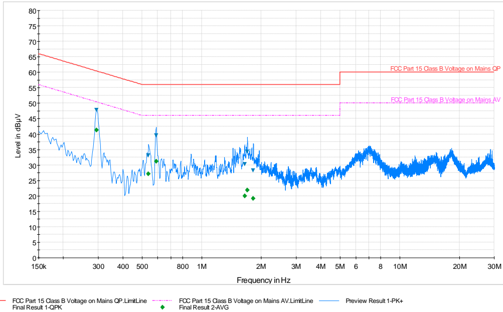
Plot 6-64. Line Conducted Plot with 802.11b (N)
