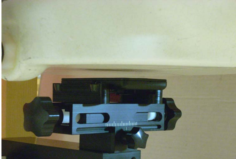
Figure 20-1 SAR Test Setup Photo 1: Front
