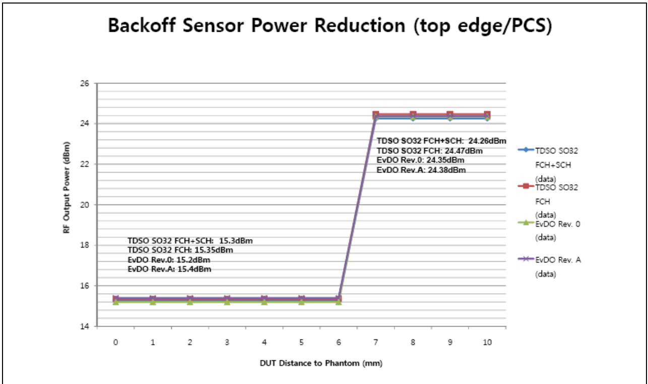
Figure 11-5 PCS Back off Power Reduction Graph – Top at 0° Angle
