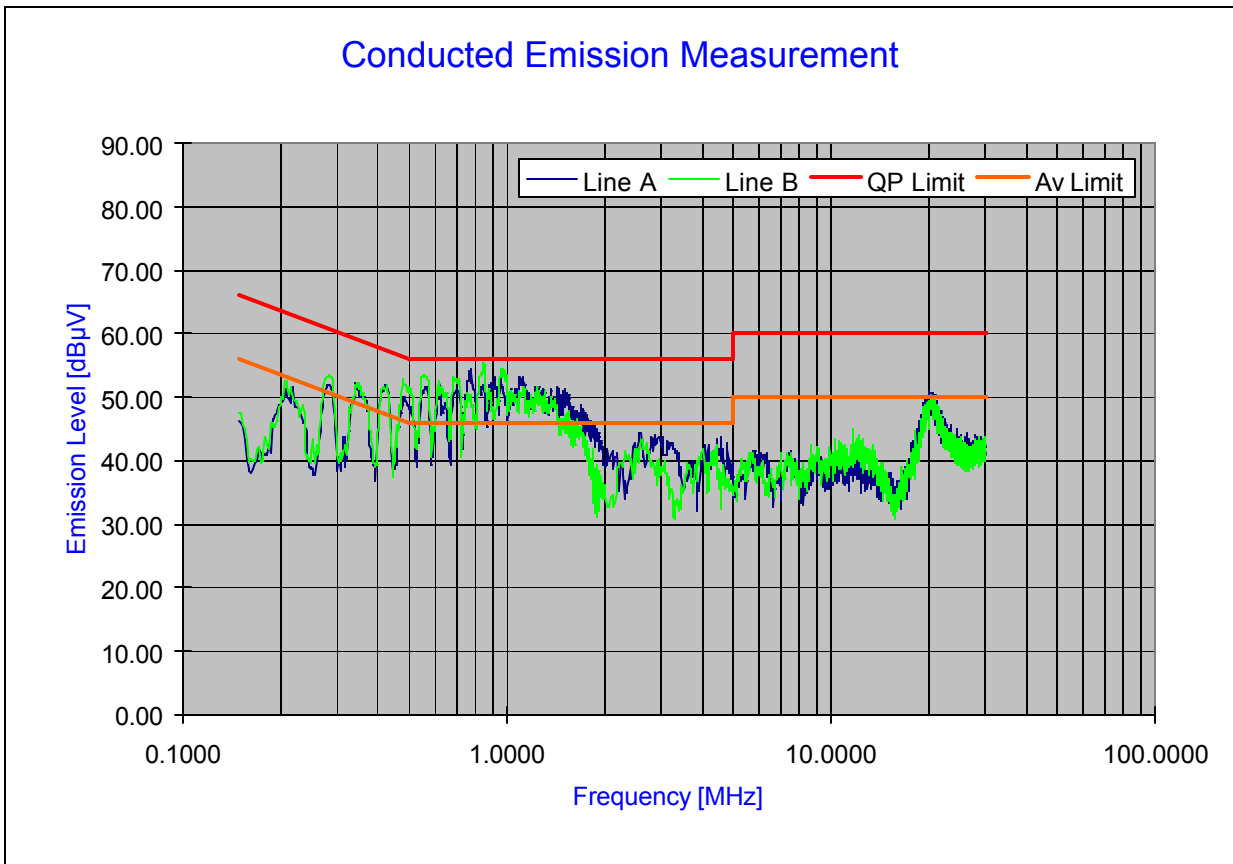
Plot 6-55. Line Conducted Plot with 802.11a (UNII-I Band)
