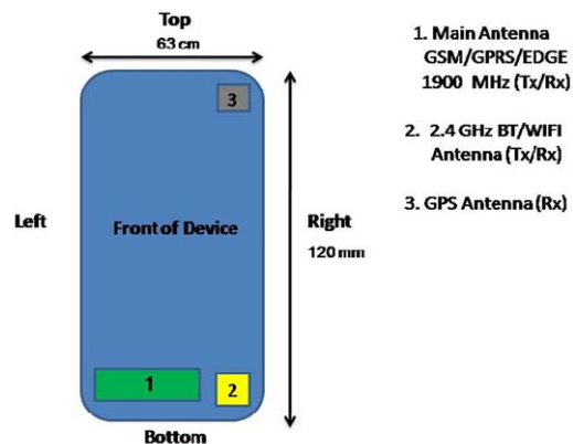
Figure 1-1 DUT Antenna Locations
