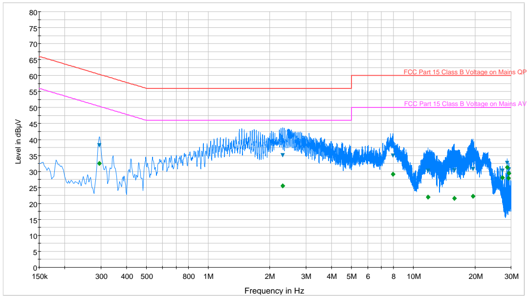
Plot 6-33. Line-Conducted Test Plot (L1)
