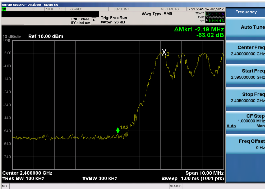
Plot 6-21. Band Edge Plot (Bluetooth with Hopping Enabled, 1Mbps)
