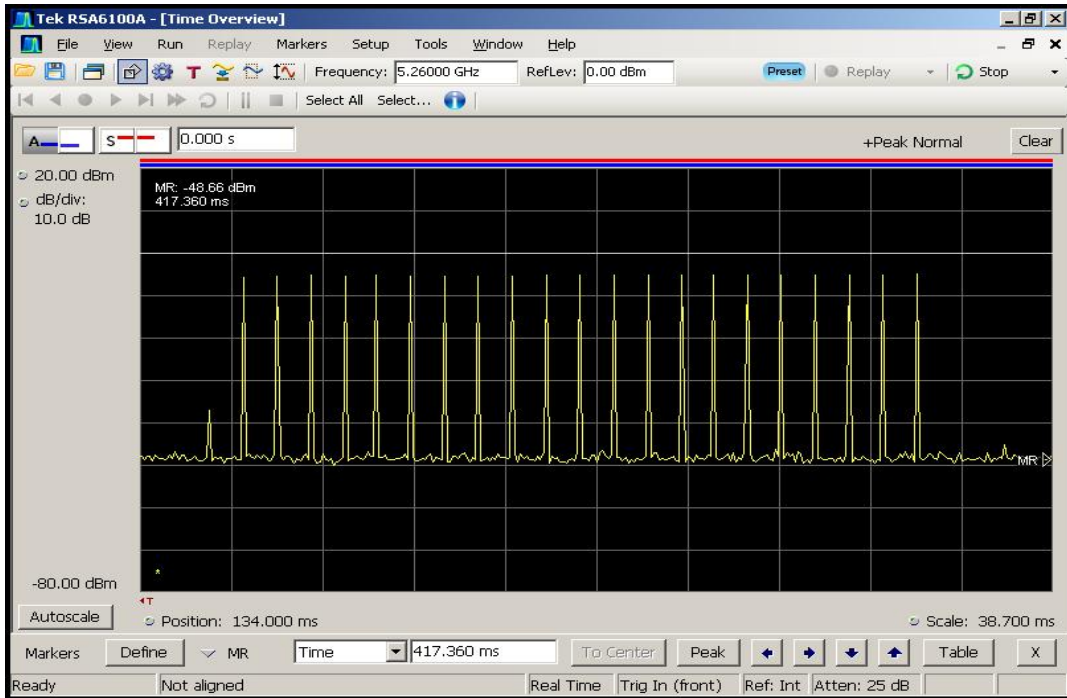
Figure 5-1. Type 1 Radar Pulse
