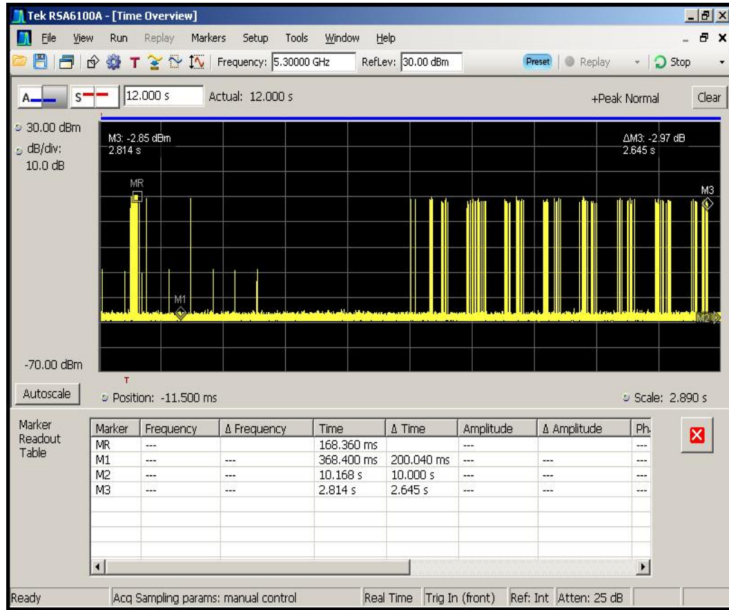
Figure 5-6. Channel Closing Transmission Time, Aggregate Time After 200ms
