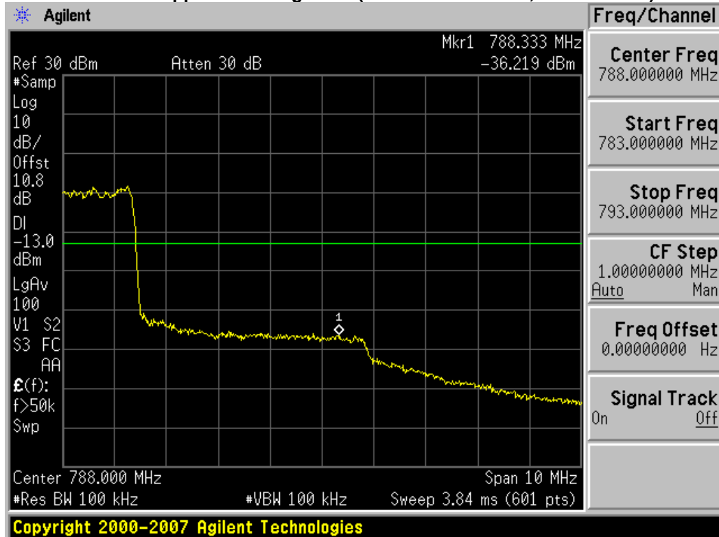
Plot 7-12. Upper Band Edge Plot (16-QAM – RB Size 25, RB Offset 12)
