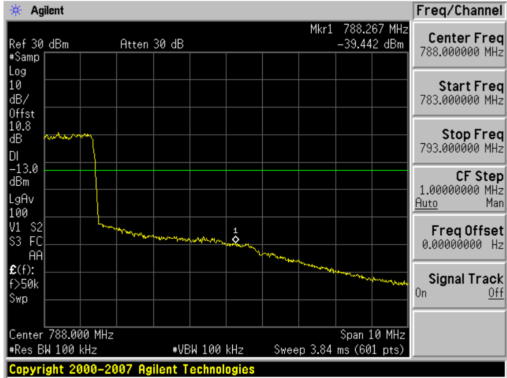
Plot 7-11. Upper Band Edge Plot (QPSK – RB Size 25, RB Offset 12)
