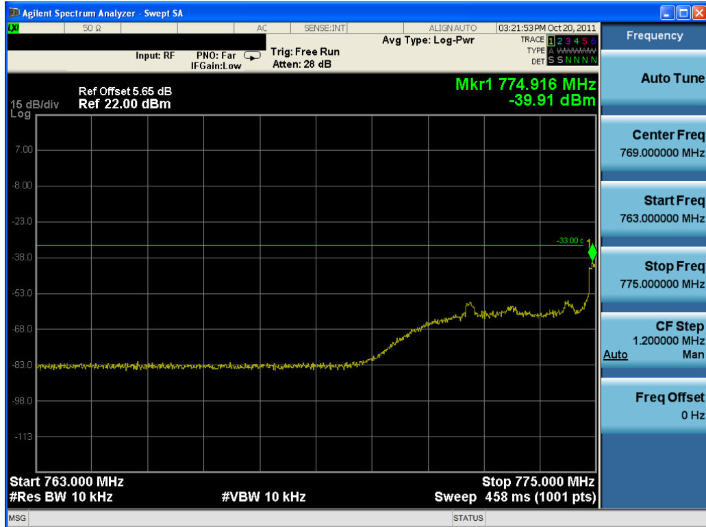
Plot 7-4. Lower Emission Mask (763 – 775MHz) Plot (16-QAM – RB Size 1, Offset 0)
