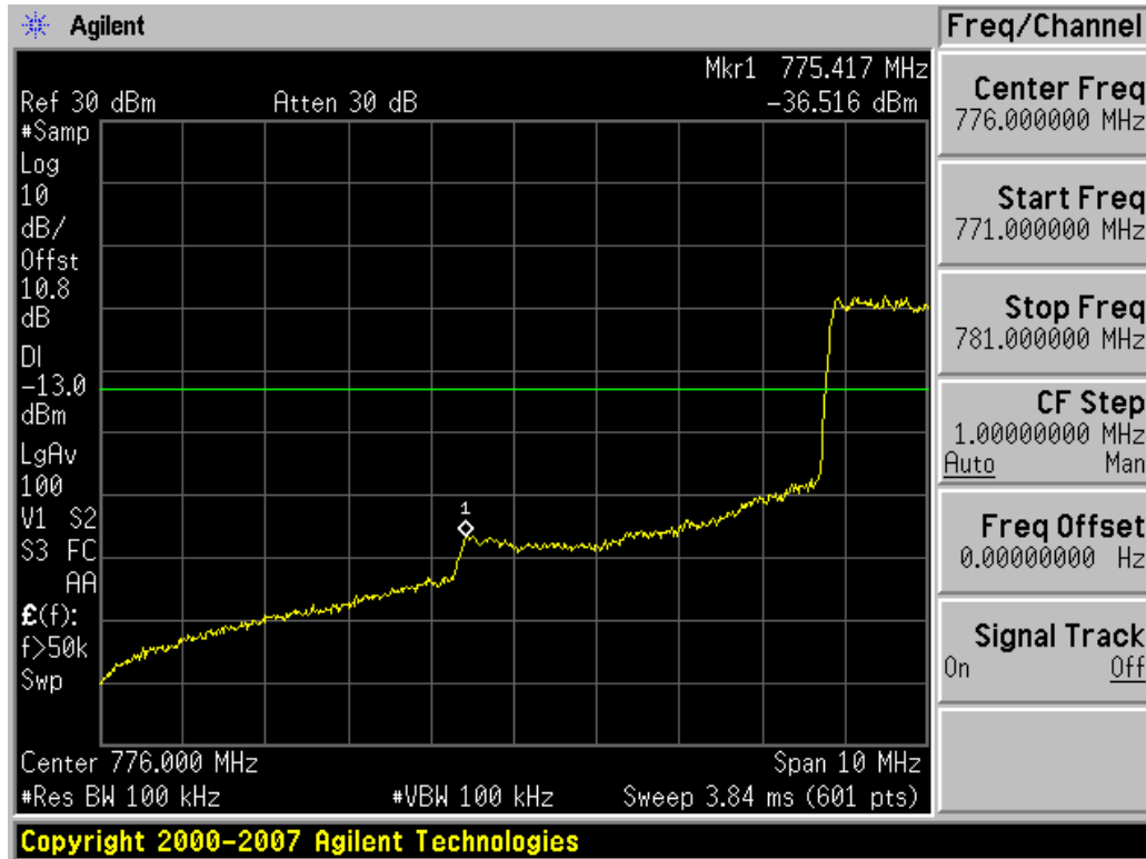
Plot 7-1. Lower Band Edge Plot (QPSK – RB Size 25, RB Offset 12)
