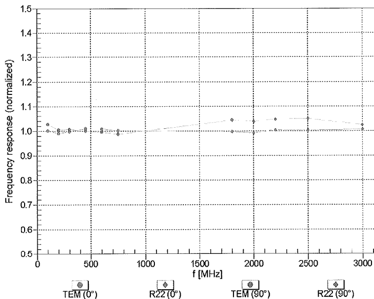
Uncertainty of Frequency Response of H-field: ± 6.3% (k=2)
