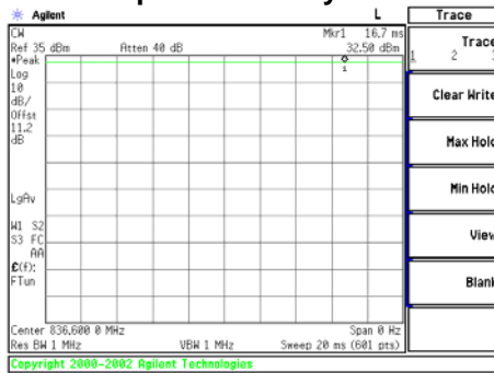
Figure 8-6 GSM850 CW Signal
