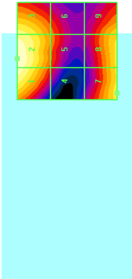
Figure 10-1 Sample E-field Scan Overlay
