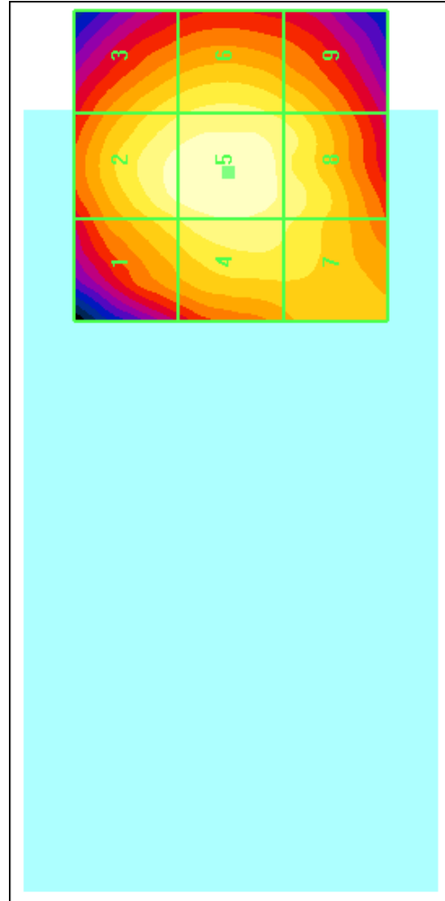
Figure 10-2 Sample H-field Scan Overlay
