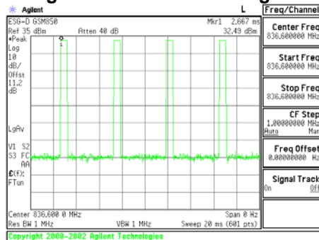
Figure 8-8 GSM850 Signal
