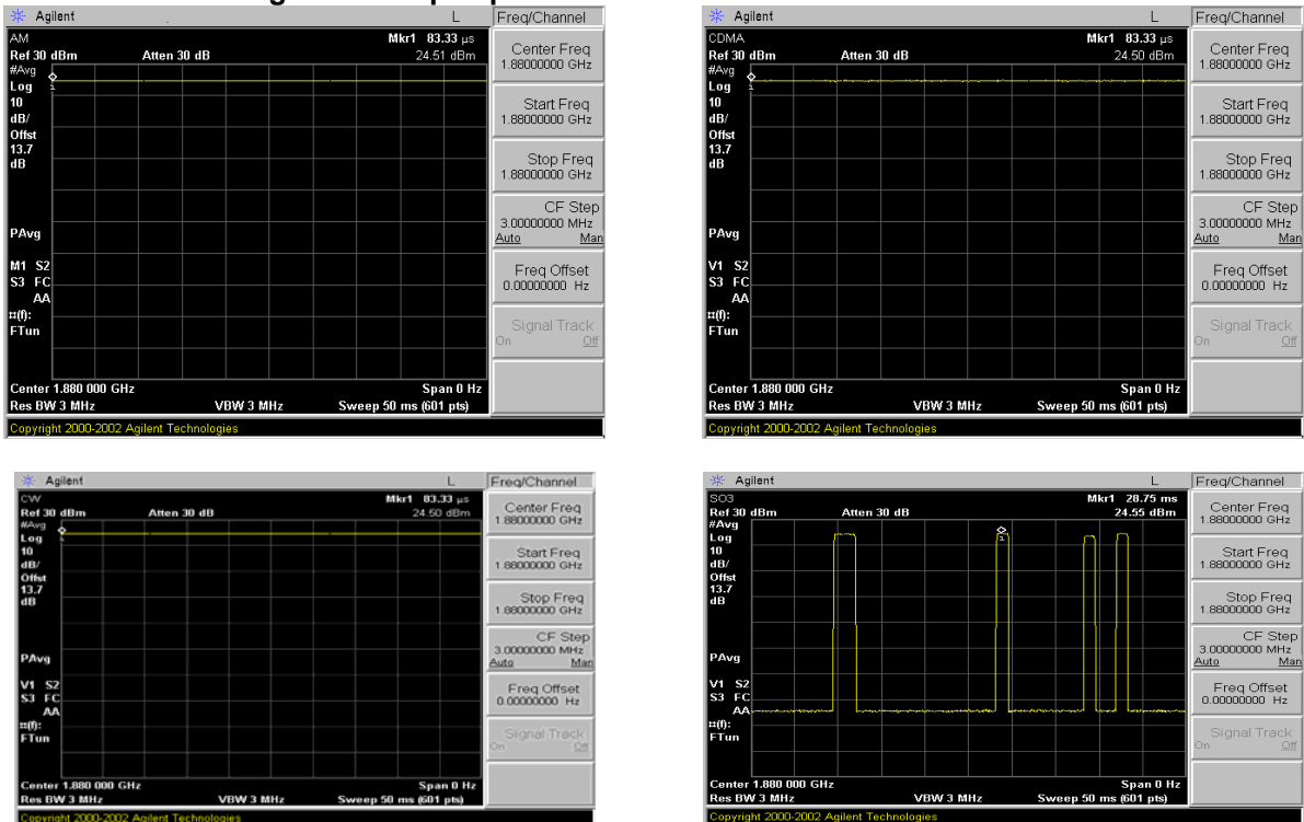
Figure 8-4 Zero-Span Plots
