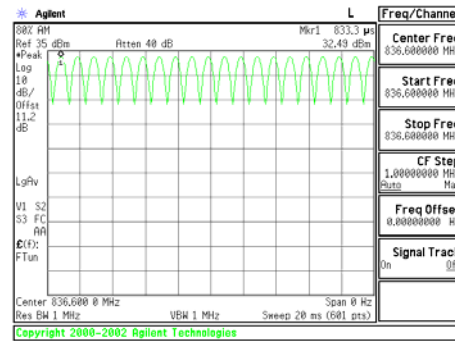
Figure 8-7 GSM850 80% AM Signal
