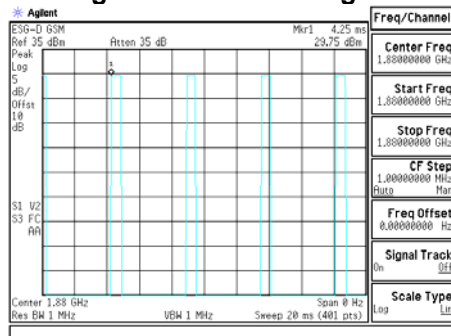
Figure 8-10 GSM1900 Signal
