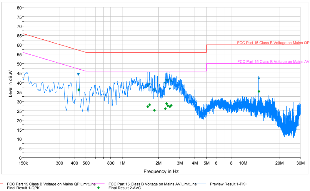
Plot 8-1. Line-Conducted Test Plot (L1)
