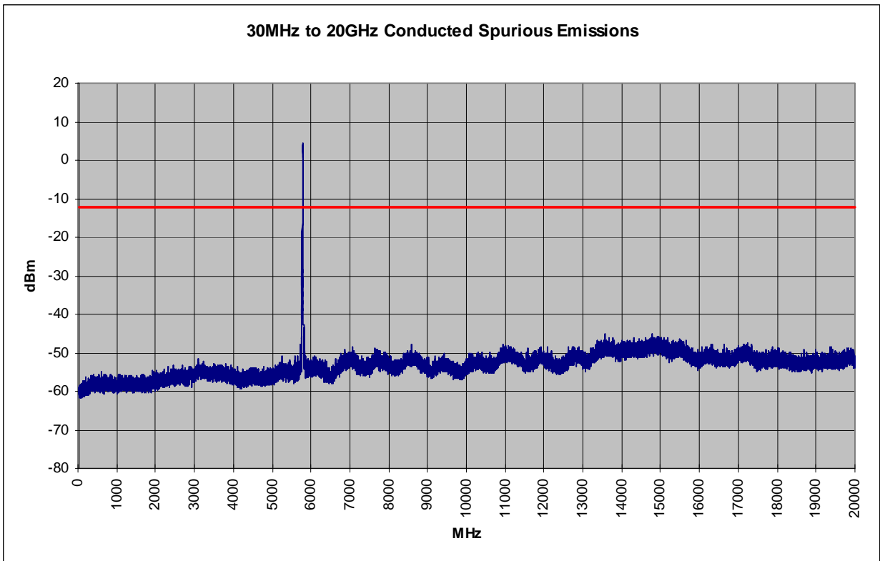
Plot 6-57. Conducted Spurious Plot (802.11a – Ch. 157)
