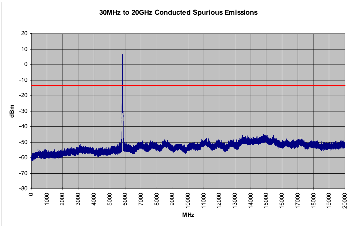
Plot 6-59. Conducted Spurious Plot (802.11a – Ch. 165)
