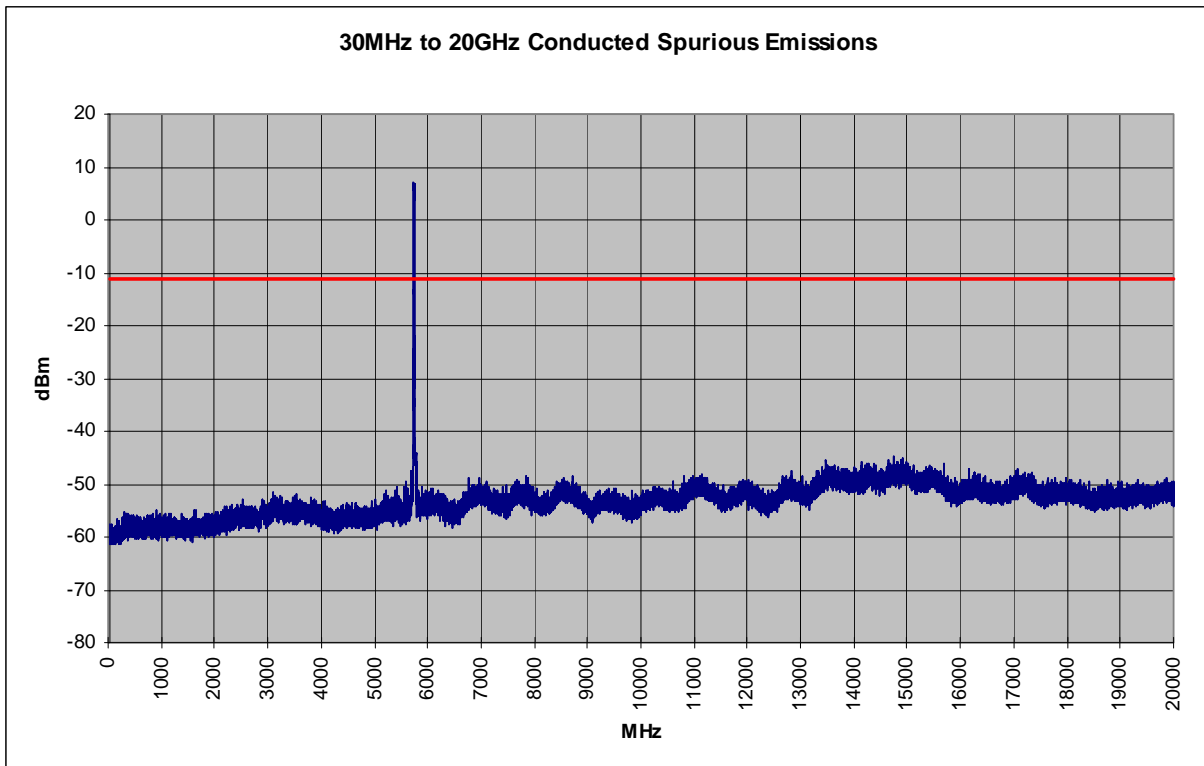
Plot 6-55. Conducted Spurious Plot (802.11a – Ch. 149)
