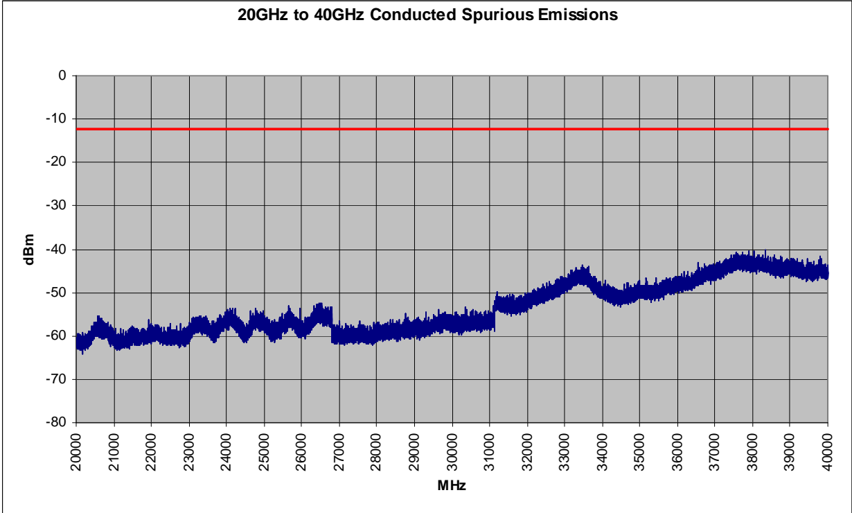
Plot 6-58. Conducted Spurious Plot (802.11a – Ch. 157)
