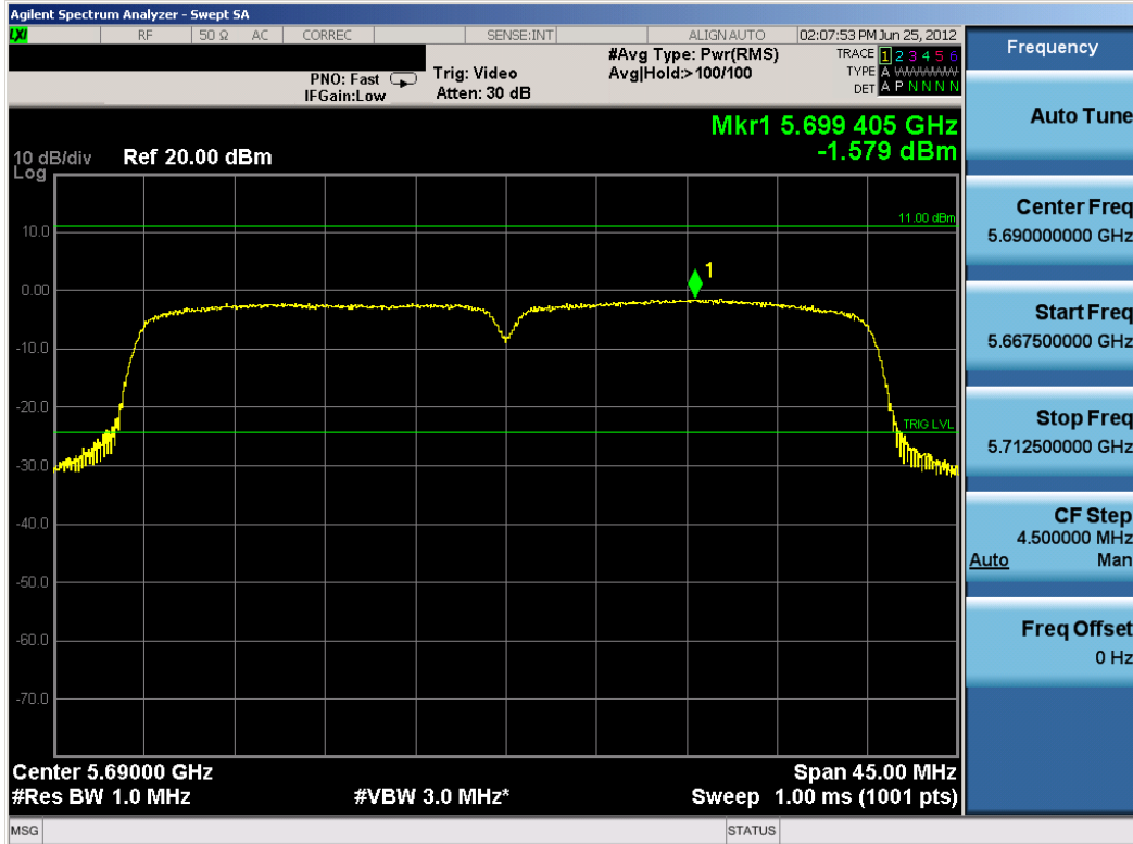
Plot 6-50. Peak Power Spectral Density Plot (40MHz BW 802.11n (UNII Band 3) – Ch. 138)
