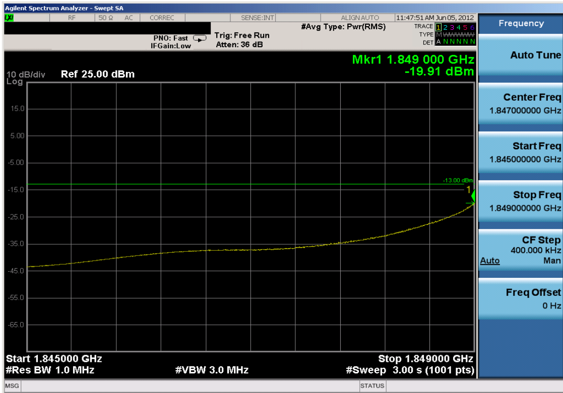
Plot 7-40. 4MHz Span Plot (PCS CDMA Mode – Ch. 25)
