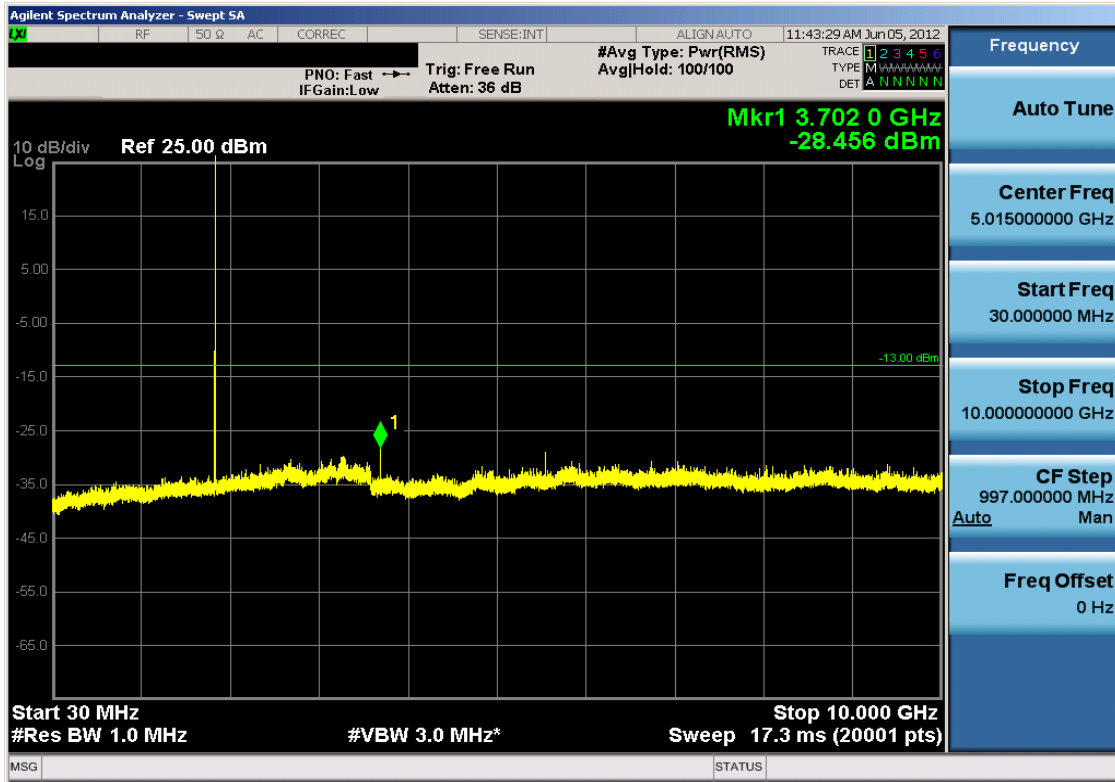
Plot 7-37. Conducted Spurious Plot (PCS CDMA Mode – Ch. 25)
