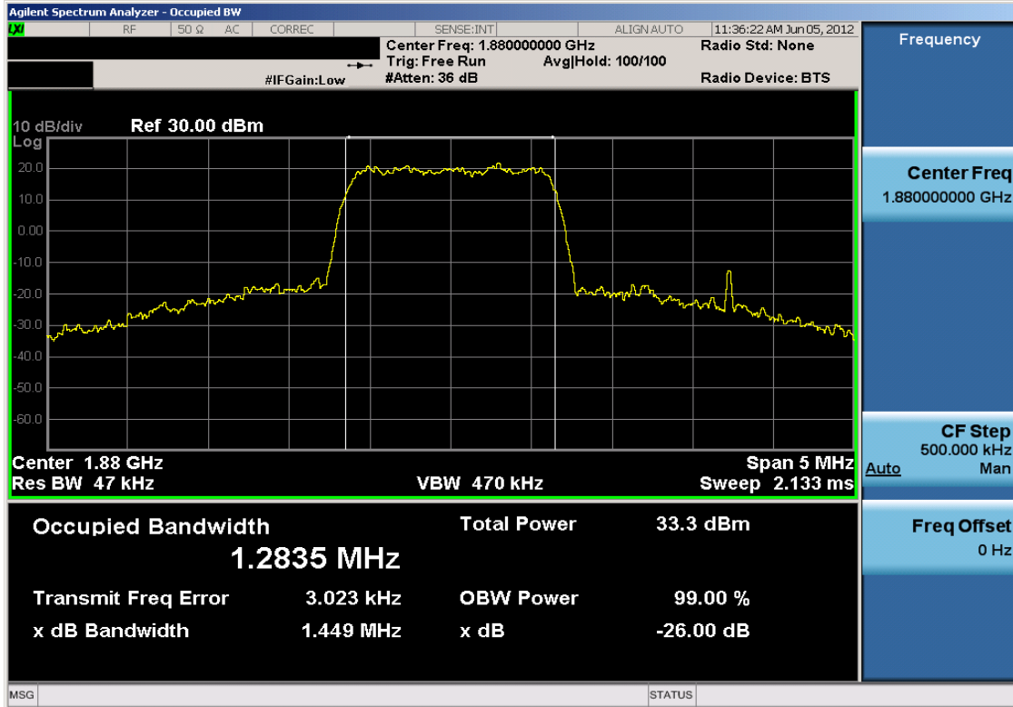
Plot 7-43. Occupied Bandwidth Plot (PCS CDMA Mode – Ch. 600)
