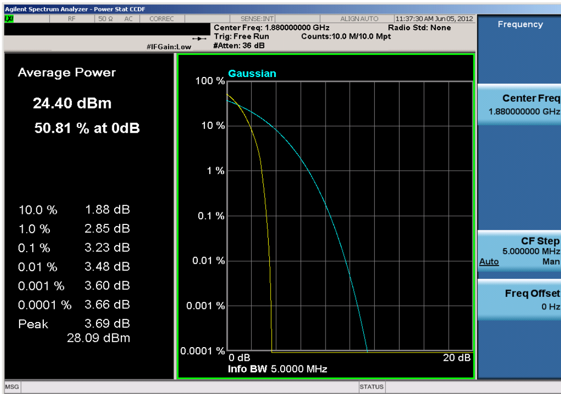
Plot 7-44. Peak-Average Ratio Plot (PCS CDMA Mode – Ch. 600)
