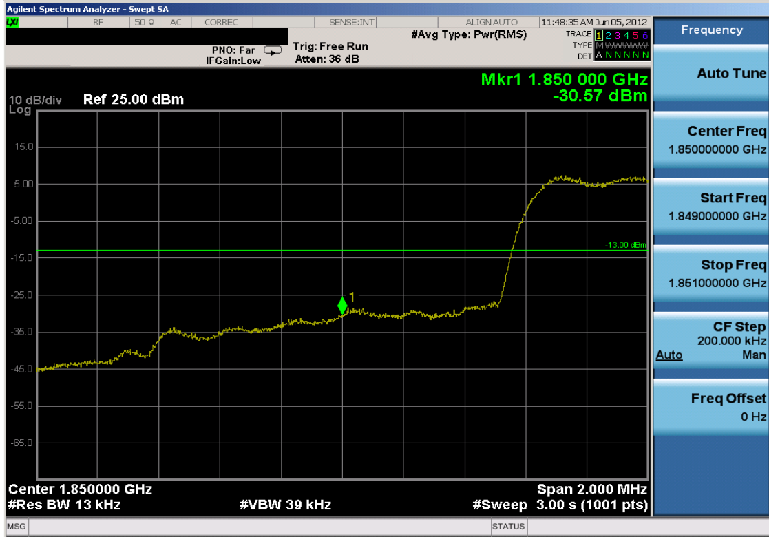
Plot 7-39. Band Edge Plot (PCS CDMA Mode – Ch. 25)
