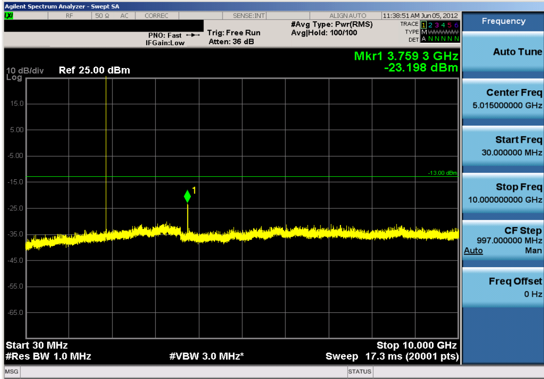
Plot 7-41. Conducted Spurious Plot (PCS CDMA Mode – Ch. 600)
