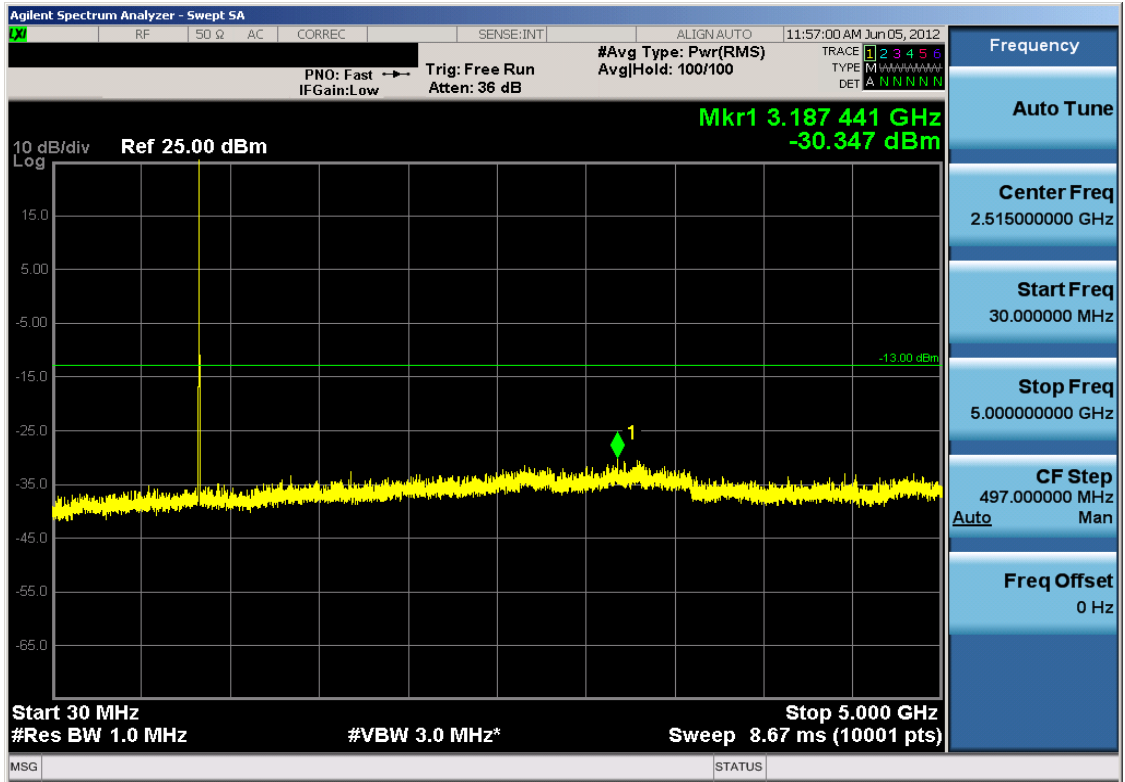
Plot 7-33. Conducted Spurious Plot (Cellular CDMA Mode – Ch. 777)
