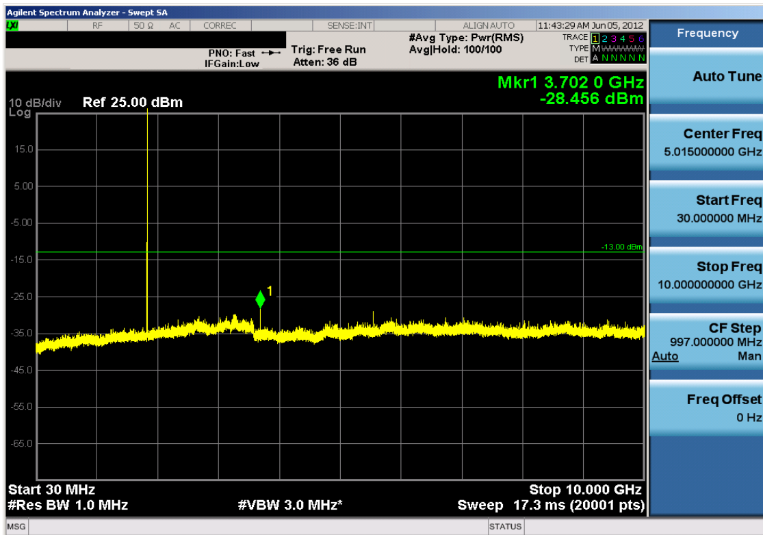
Plot 7-38. Conducted Spurious Plot (PCS CDMA Mode – Ch. 25)
