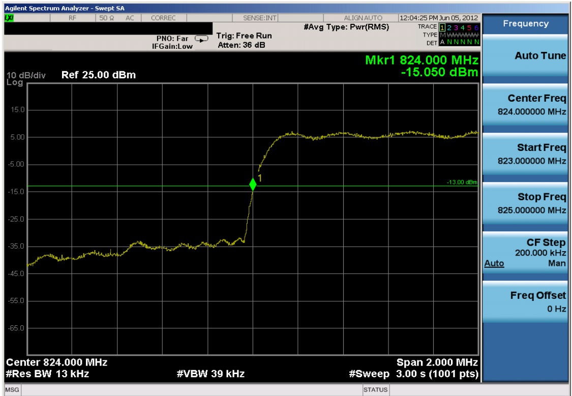
Plot 7-28. Band Edge Plot (Cellular CDMA Mode – Ch. 1013)
