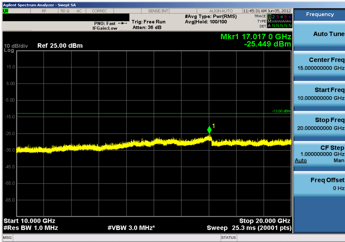
Plot 7-46. Conducted Spurious Plot (PCS CDMA Mode – Ch. 1175)
