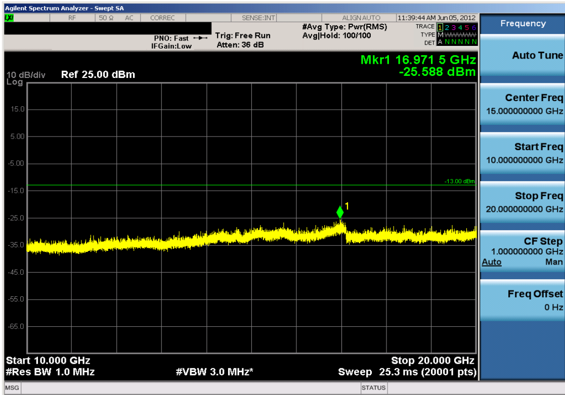
Plot 7-42. Conducted Spurious Plot (PCS CDMA Mode – Ch. 600)
