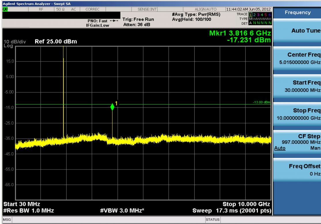
Plot 7-45. Conducted Spurious Plot (PCS CDMA Mode – Ch. 1175)
