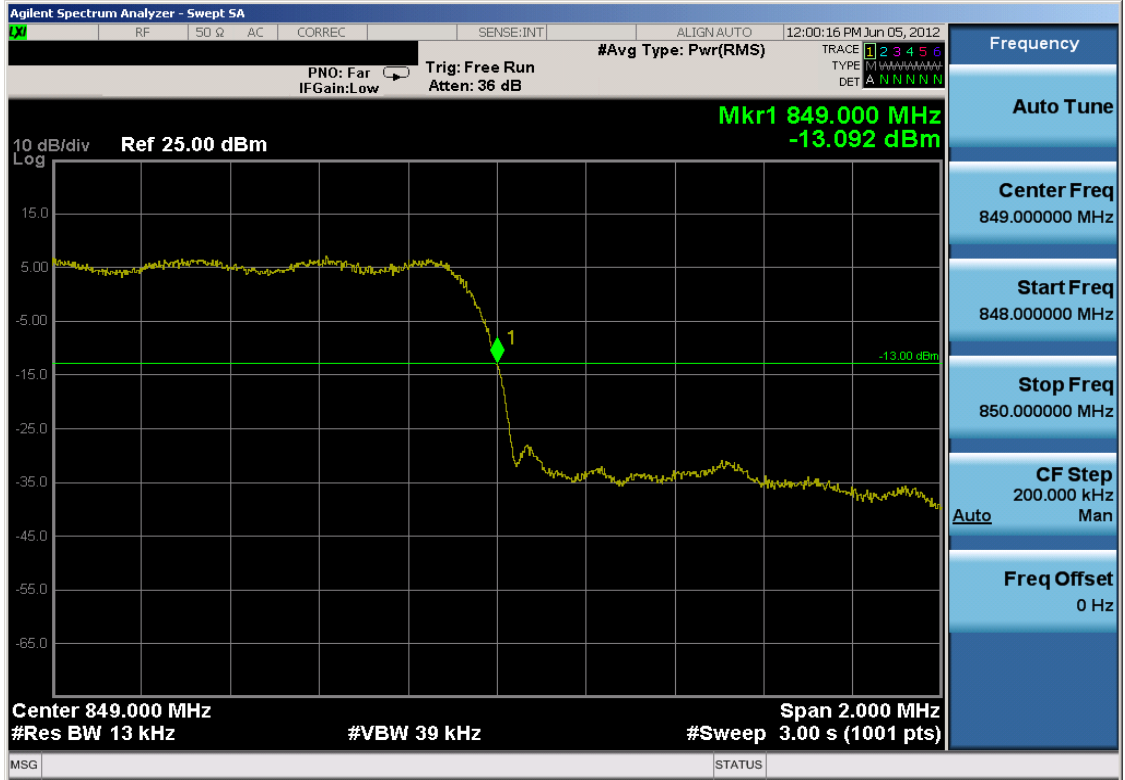
Plot 7-35. Band Edge Plot (Cellular CDMA Mode – Ch. 777)
