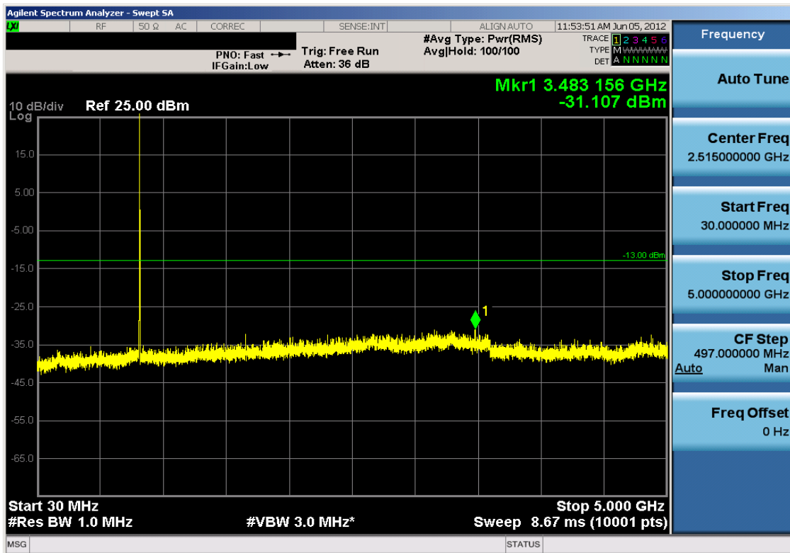
Plot 7-30. Conducted Spurious Plot (Cellular CDMA Mode – Ch. 384)
