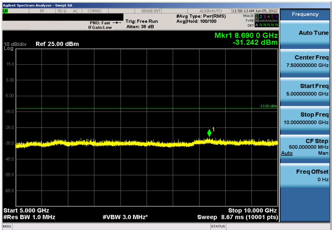
Plot 7-34. Conducted Spurious Plot (Cellular CDMA Mode – Ch. 777)
