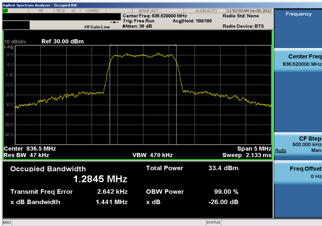
Plot 7-32. Occupied Bandwidth Plot (Cellular CDMA Mode – Ch. 384)
