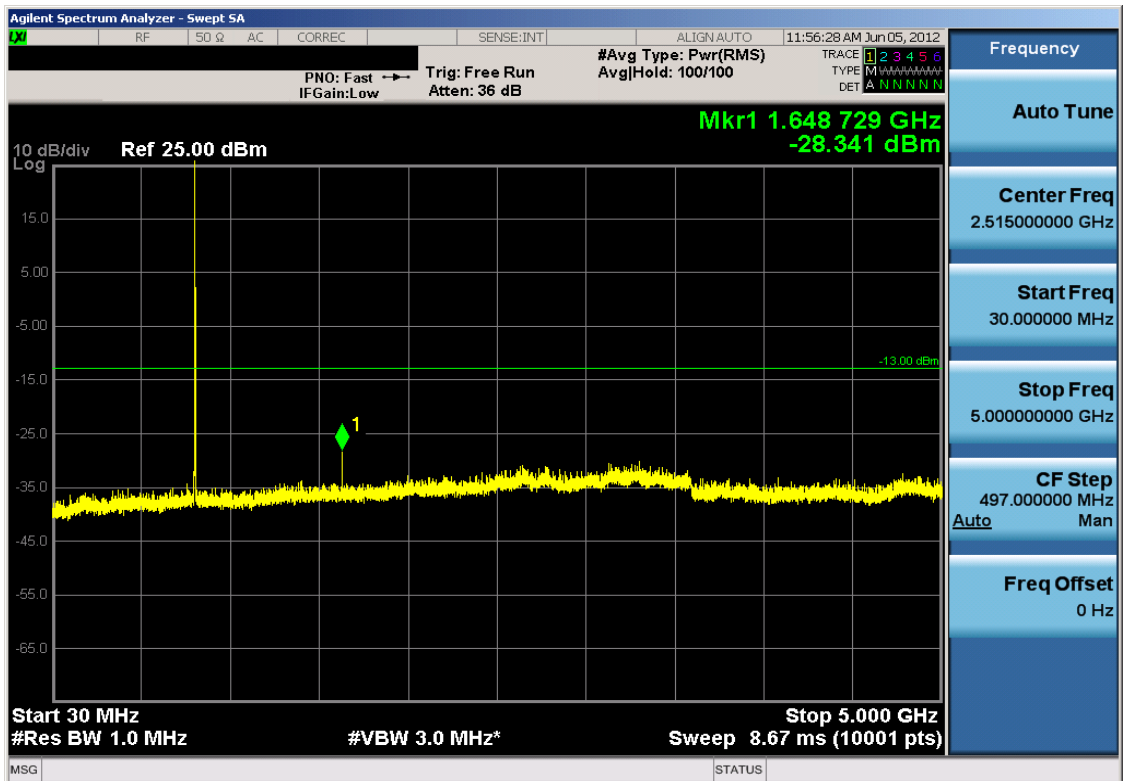
Plot 7-26. Conducted Spurious Plot (Cellular CDMA Mode – Ch. 1013)
