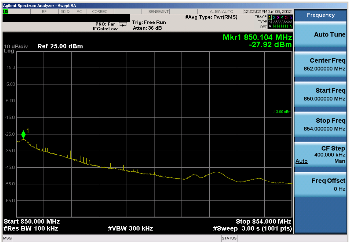
Plot 7-36. 4MHz Span Plot (Cellular CDMA Mode – Ch. 777)
