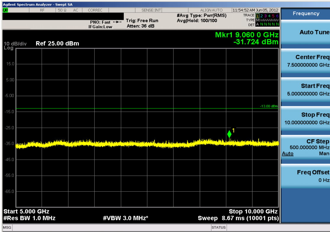
Plot 7-31. Conducted Spurious Plot (Cellular CDMA Mode – Ch. 384)
