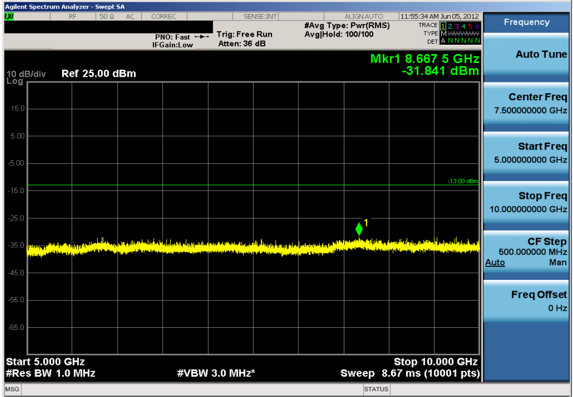
Plot 7-27. Conducted Spurious Plot (Cellular CDMA Mode – Ch. 1013)
