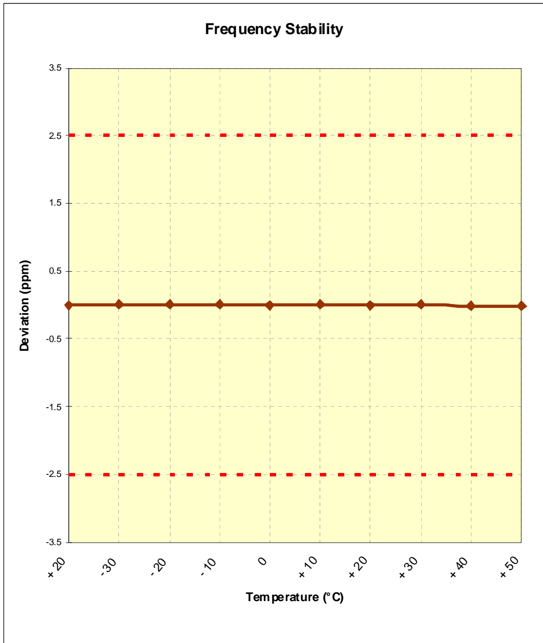
Figure 6-4. Frequency Stability Graph (PCS CDMA Mode – Ch. 600)
