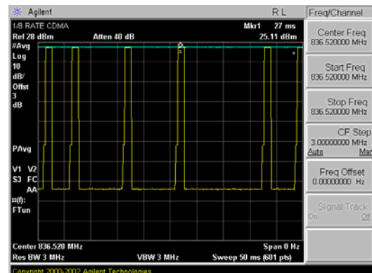
Figure 23 Zero-Span Plots
