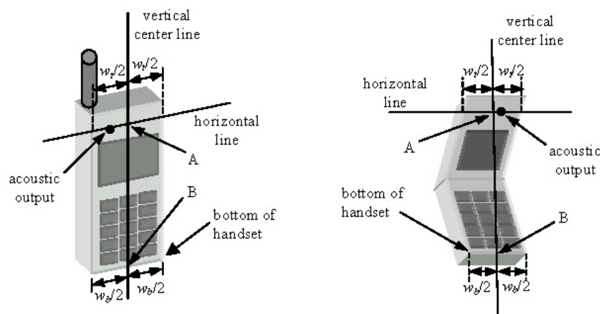
Figure 8-3 Handset Vertical Center & Horizontal Line Reference Points
