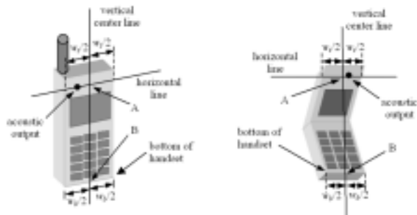
Figure 5.4 Handset vertical and horizontal reference lines
