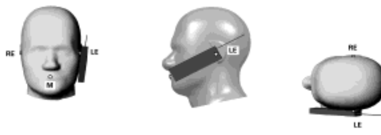
Figure 5.5 Front, Side and Top View of Cheek/Touch Position
