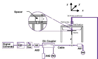
Figure 12.1 Dipole Validation 1
