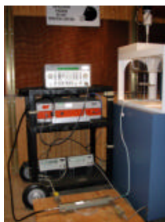
Figure A.0 Dipole Validation Test Setup
