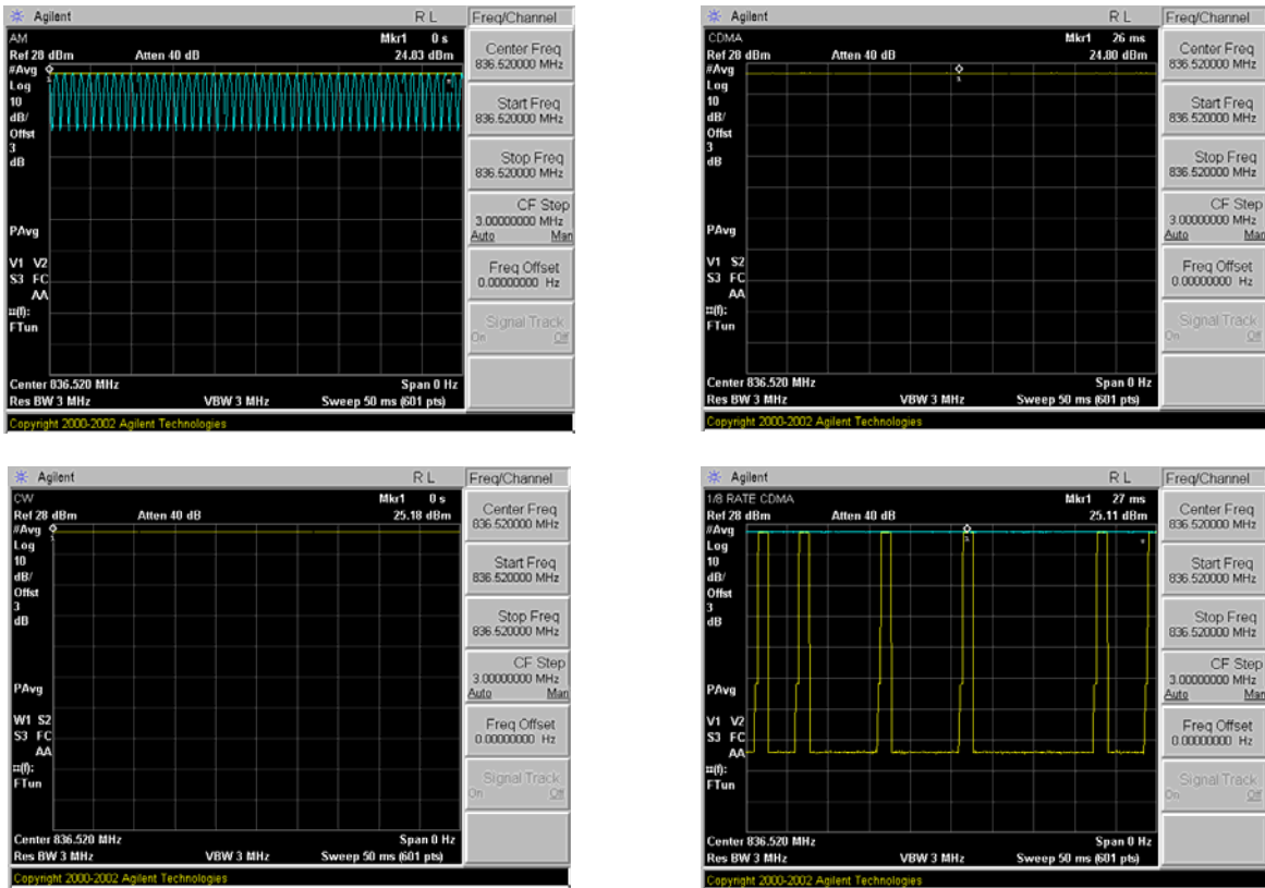
Figure 26 Zero-Span Plots
