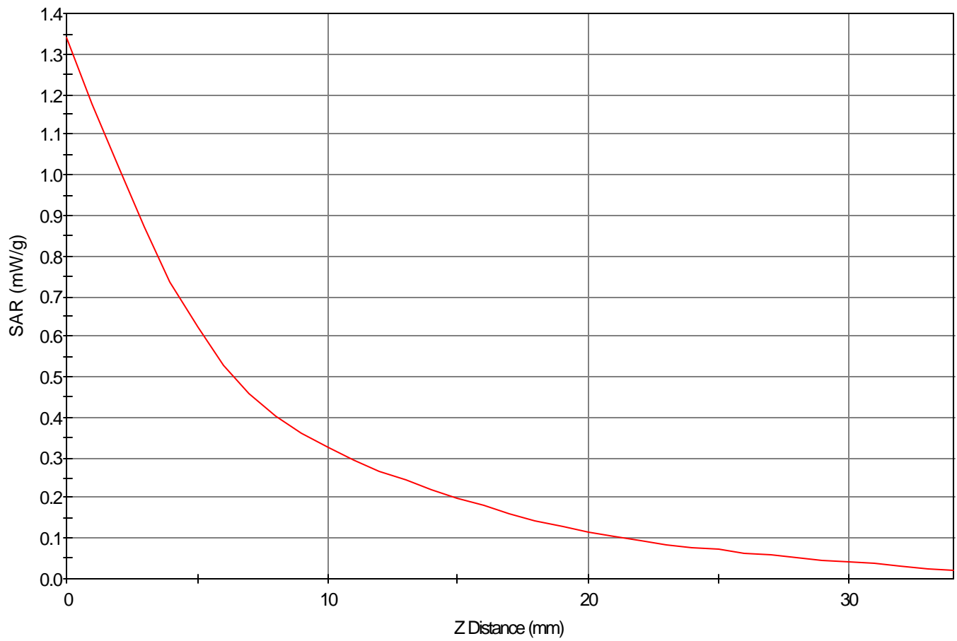
SAR - Z Axis at Hotspot x:-6.0 y:26.0
