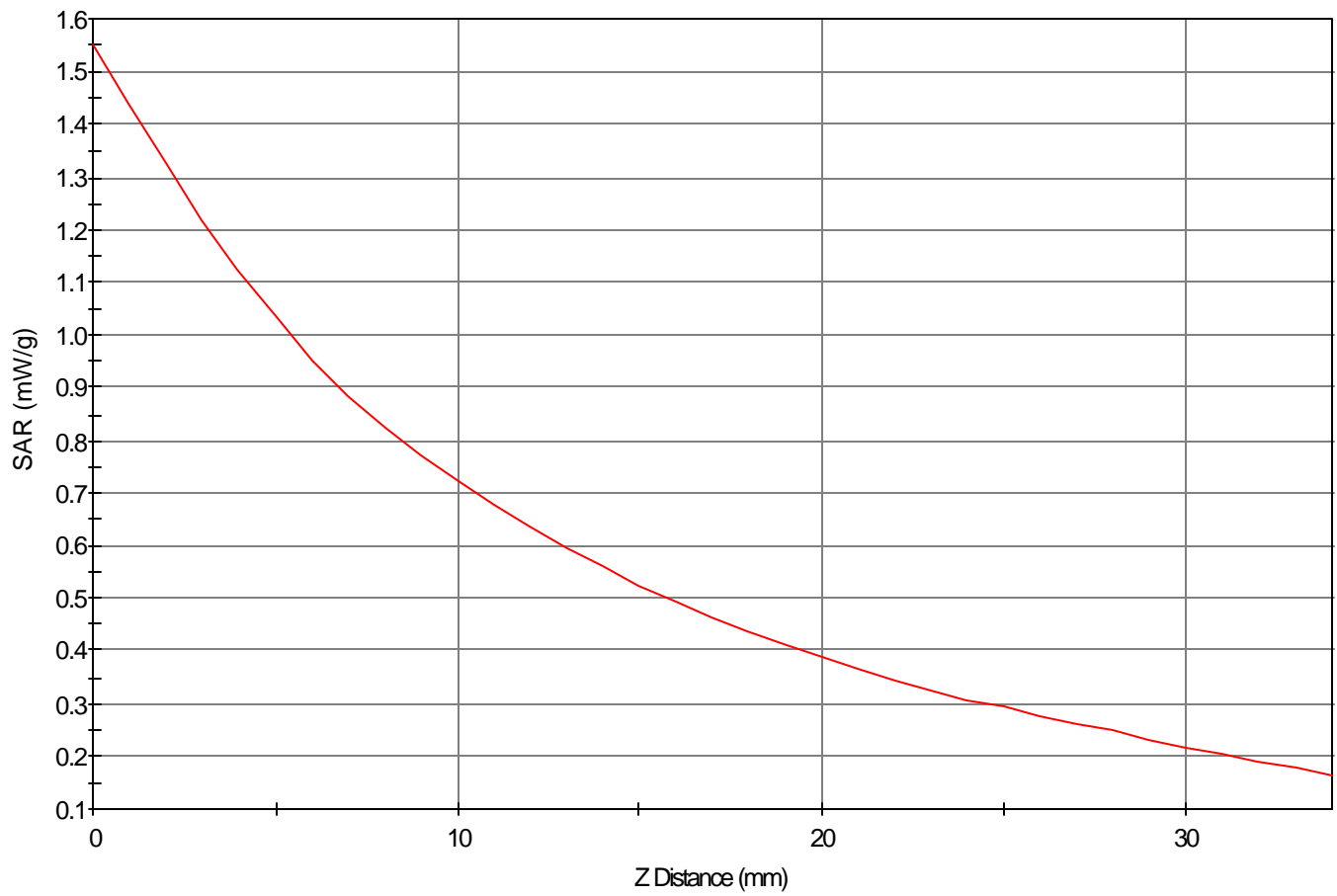
SAR - Z Axis at Hotspot x:84.0 y:18.0
