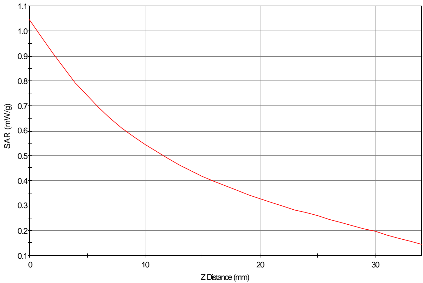
SAR - Z Axis at Hotspot x:81.0 y:9.0
