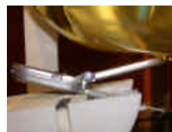
Figure A.12 Left Head SAR Test Setup -- Ear / 15° Tilt Position --
