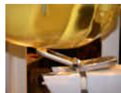
Figure A.10 Right Head SAR Test Setup -- Ear / 15° Tilt Position --
