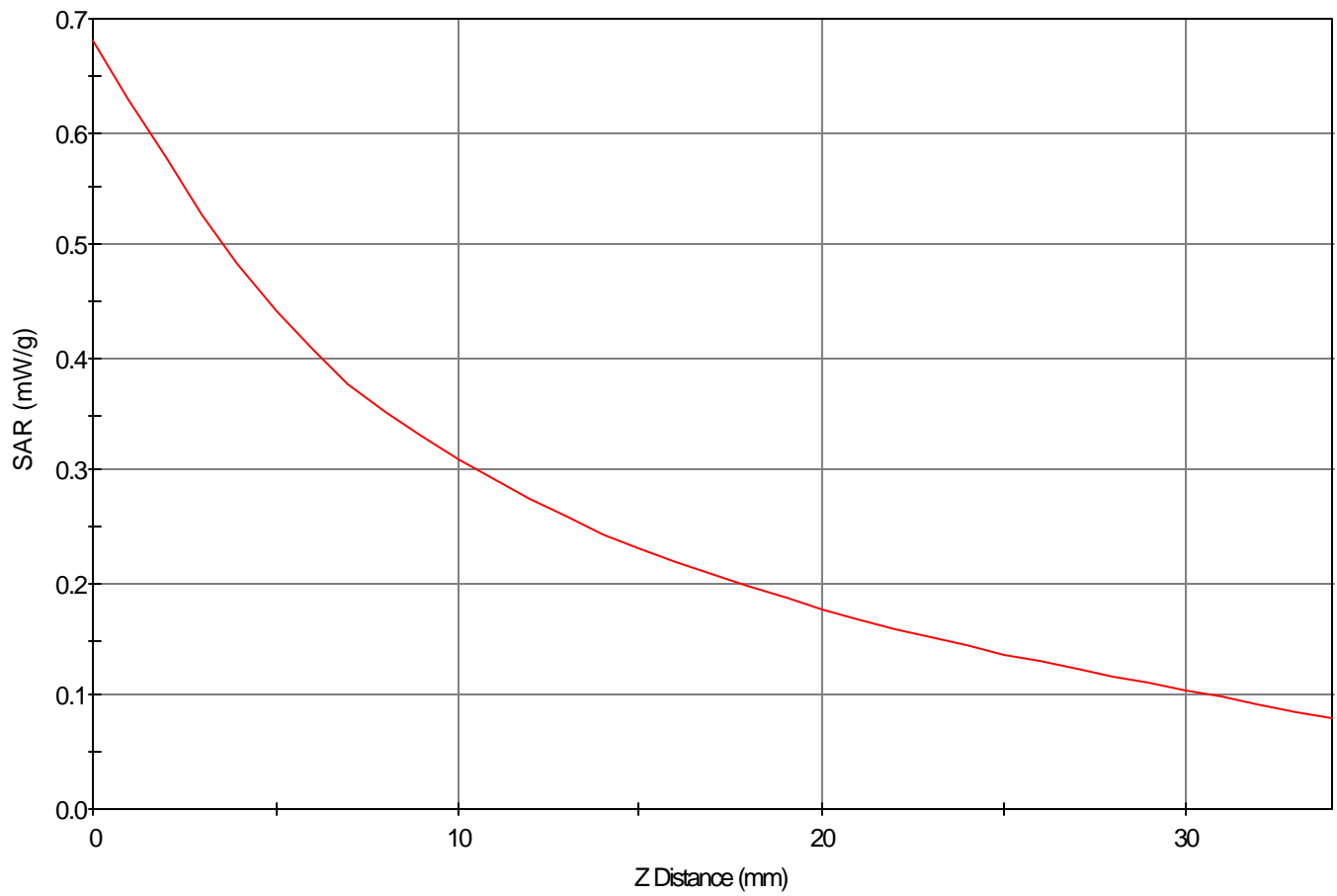
SAR - Z Axis at Hotspot x:9.0 y:-26.0
