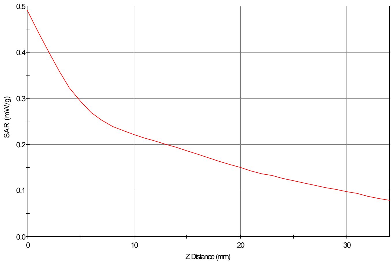
SAR - Z Axis at Hotspot x:79.0 y:17.0
