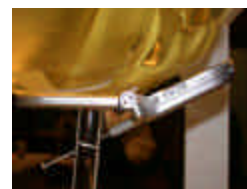
Figure A.1 Right Head SAR Test Setup -- Cheek / Touch Position --
