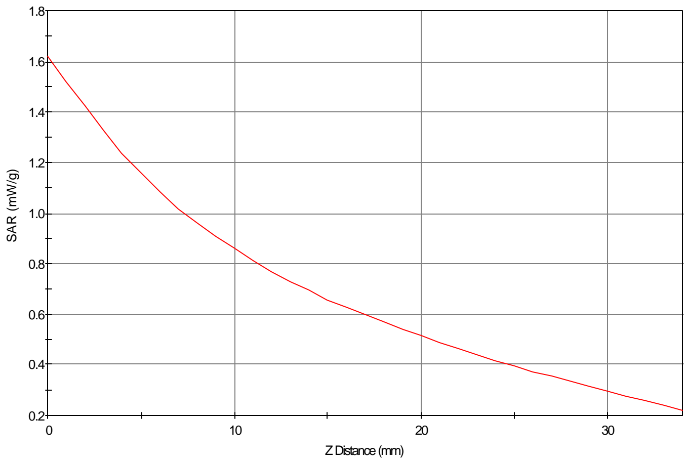
SAR - Z Axis at Hotspot x:81.0 y:10.0
