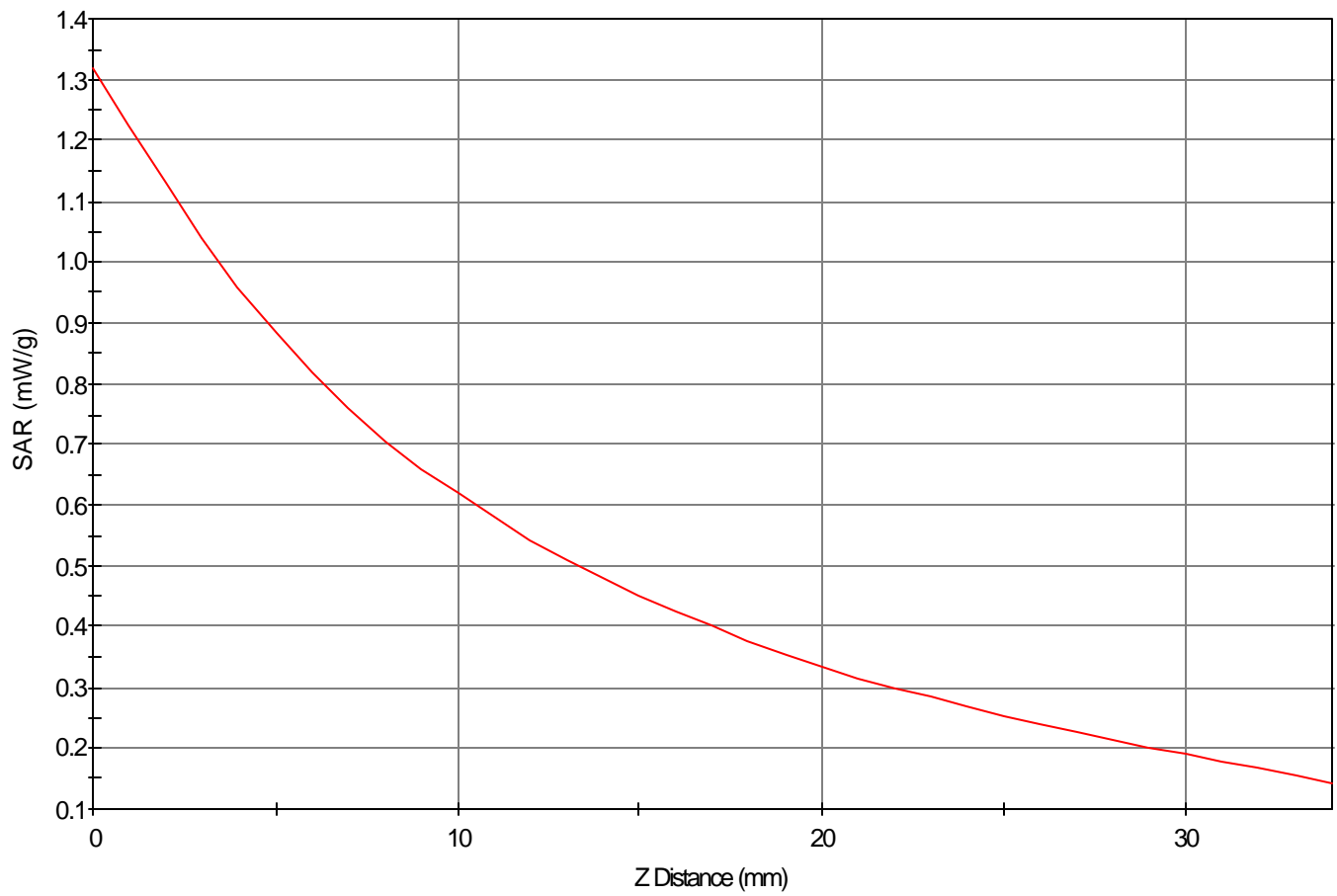
SAR - Z Axis at Hotspot x:84.0 y:20.0
