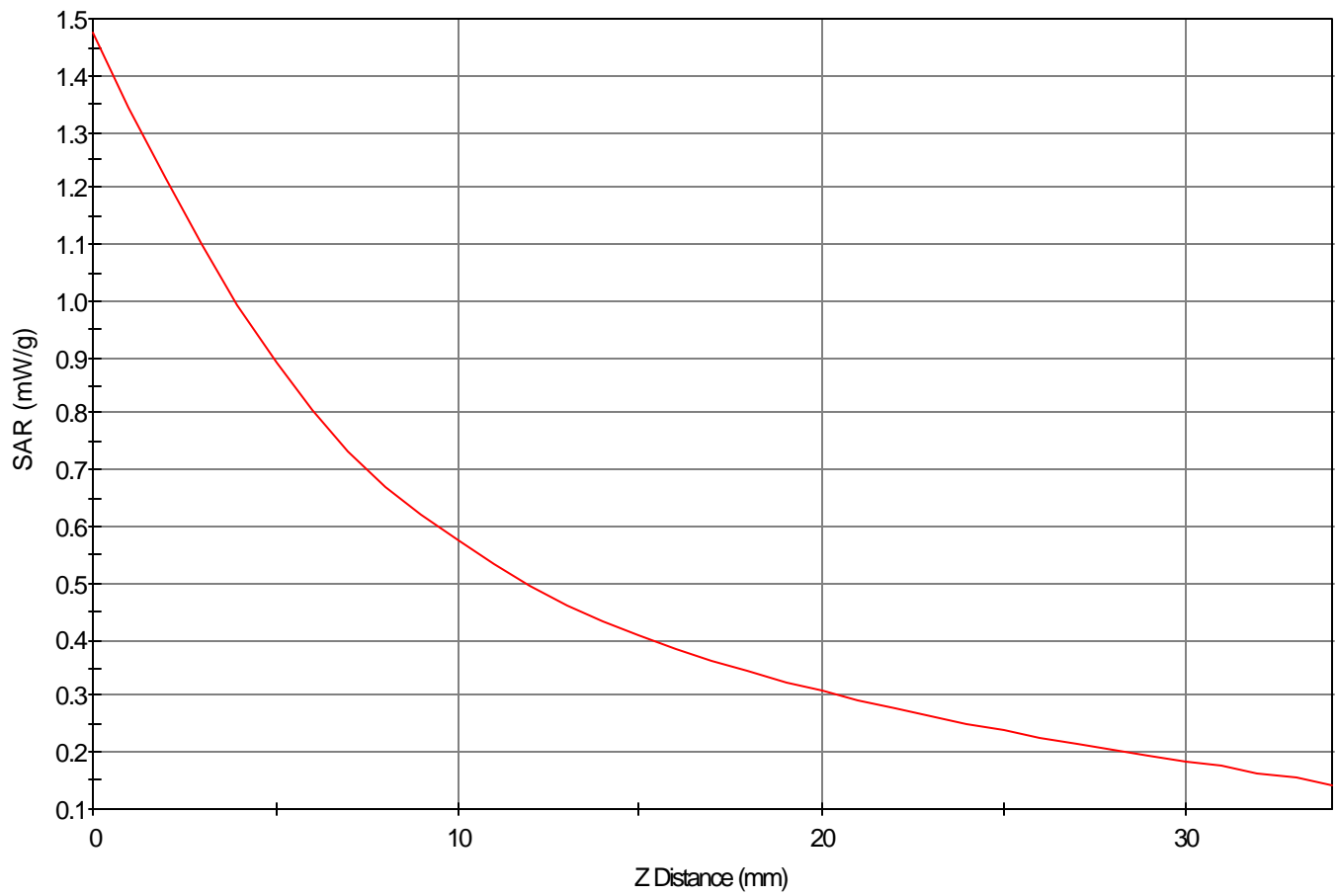
SAR - Z Axis at Hotspot x:79.0 y:5.0
