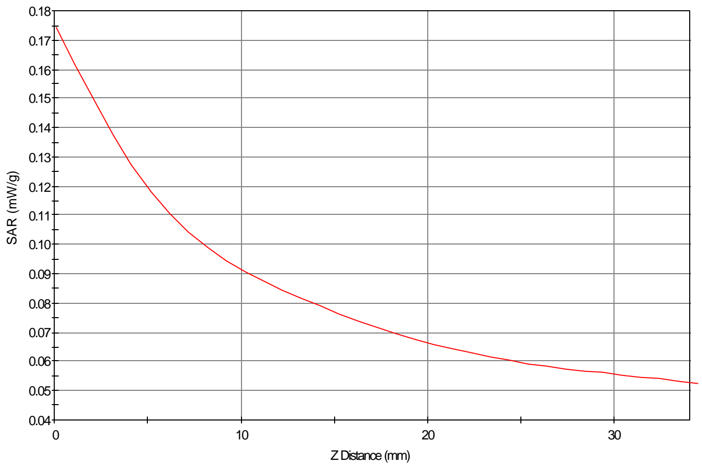
SAR - Z Axis at Hotspot x:70.0 y:-14.0
