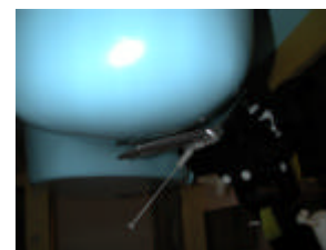
Figure 18. Right Head SAR Test Setup -- Check / Touch Position --
