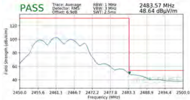
Plot 7-121. Radiated Restricted Band Edge Measurement CDD with WCP (Average)
