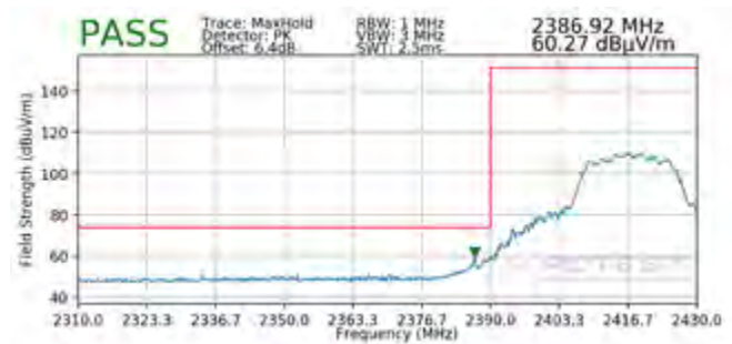
Plot 7-126. Radiated Restricted Lower Band Edge Measurement MIMO (Peak)
