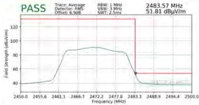
Plot 7-135. Radiated Restricted Band Edge Measurement MIMO with WCP (Average)
