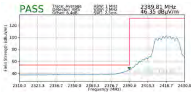
Plot 7-125. Radiated Restricted Lower Band Edge Measurement MIMO (Average)
