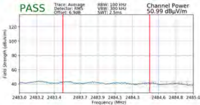
Plot 7-119. Radiated Restricted Upper Band Edge Measurement CDD (Average)
