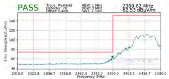
Plot 7-112. Radiated Restricted Lower Band Edge Measurement CDD (Peak)
