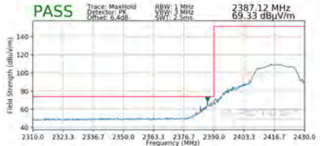
Plot 7-98. Radiated Restricted Lower Band Edge Measurement SISO ANT2 (Peak)
