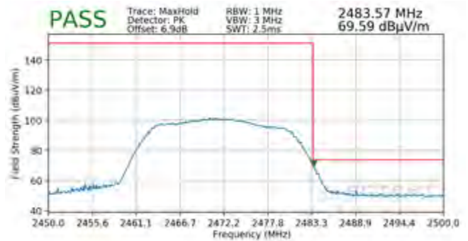
Plot 7-136. Radiated Restricted Band Edge Measurement MIMO with WCP (Peak)
