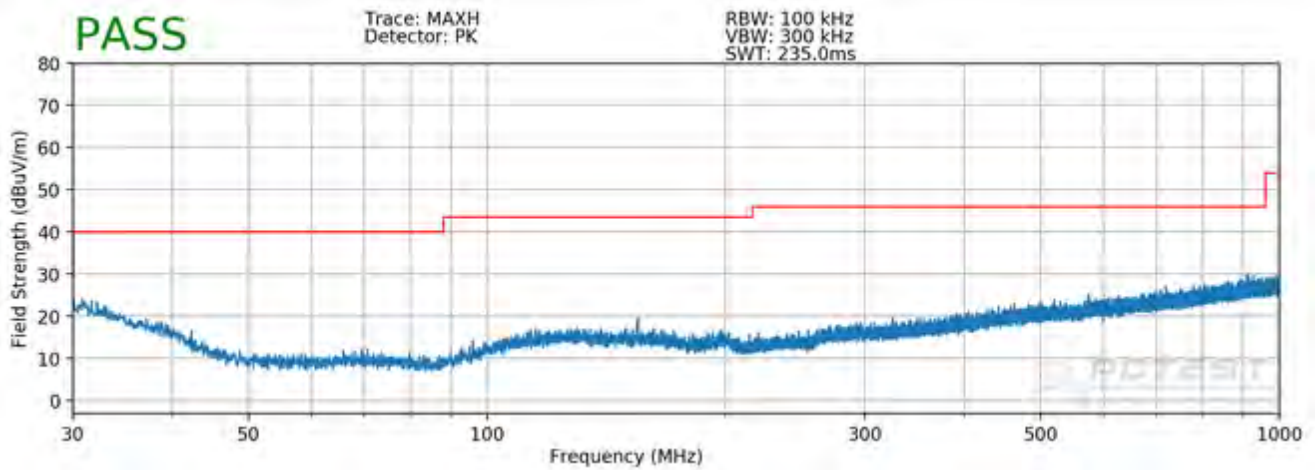
Plot 7-138. Radiated Spurious Plot below 1GHz SISO ANT2
