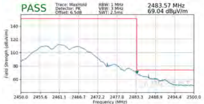
Plot 7-120. Radiated Restricted Upper Band Edge Measurement CDD (Peak)
