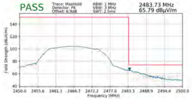
Plot 7-132. Radiated Restricted Upper Band Edge Measurement MIMO (Peak)
