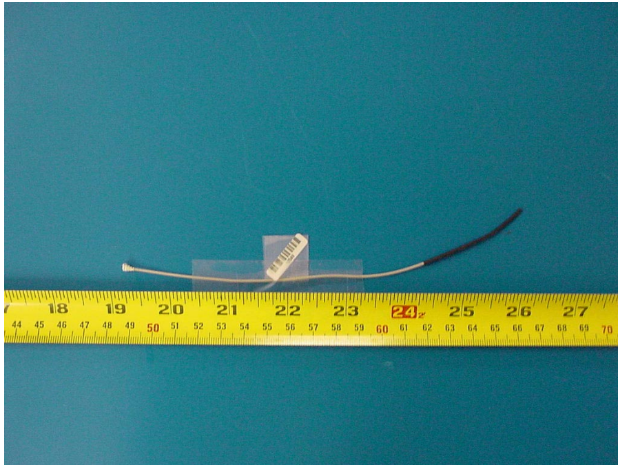
PHOTOGRAPH 8: WLAN DIPOLE ANTENNA
