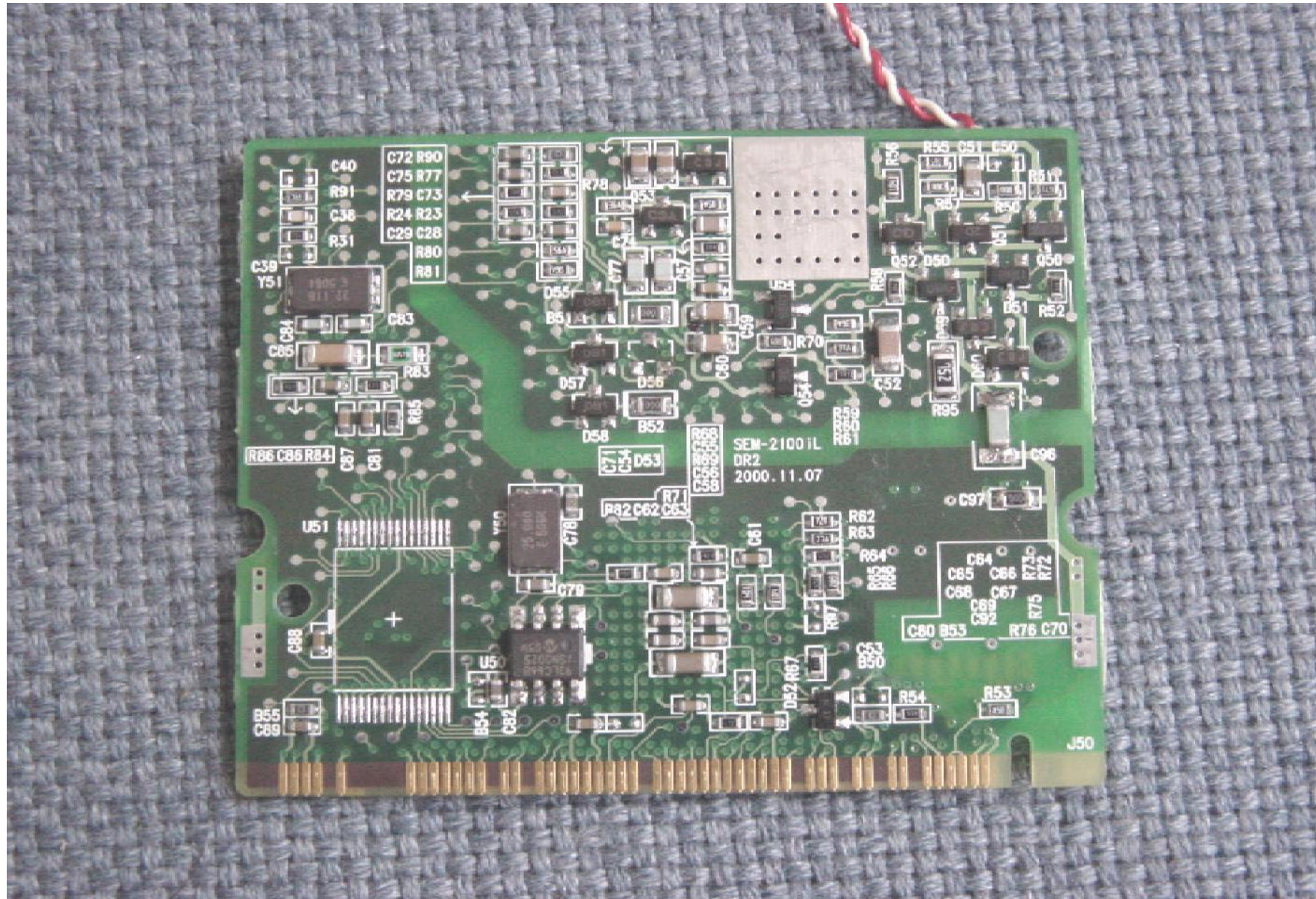
Rear side of Mini PCI LAN/Modem Combo Card
