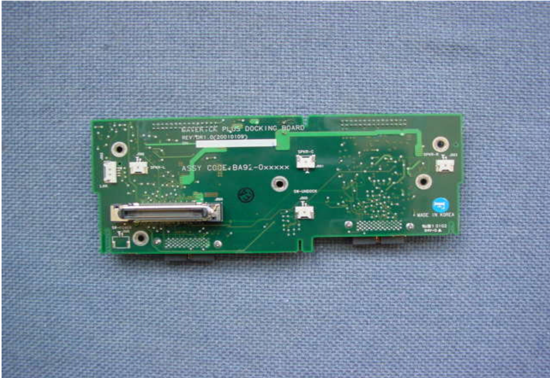
Front side of Docking Board
