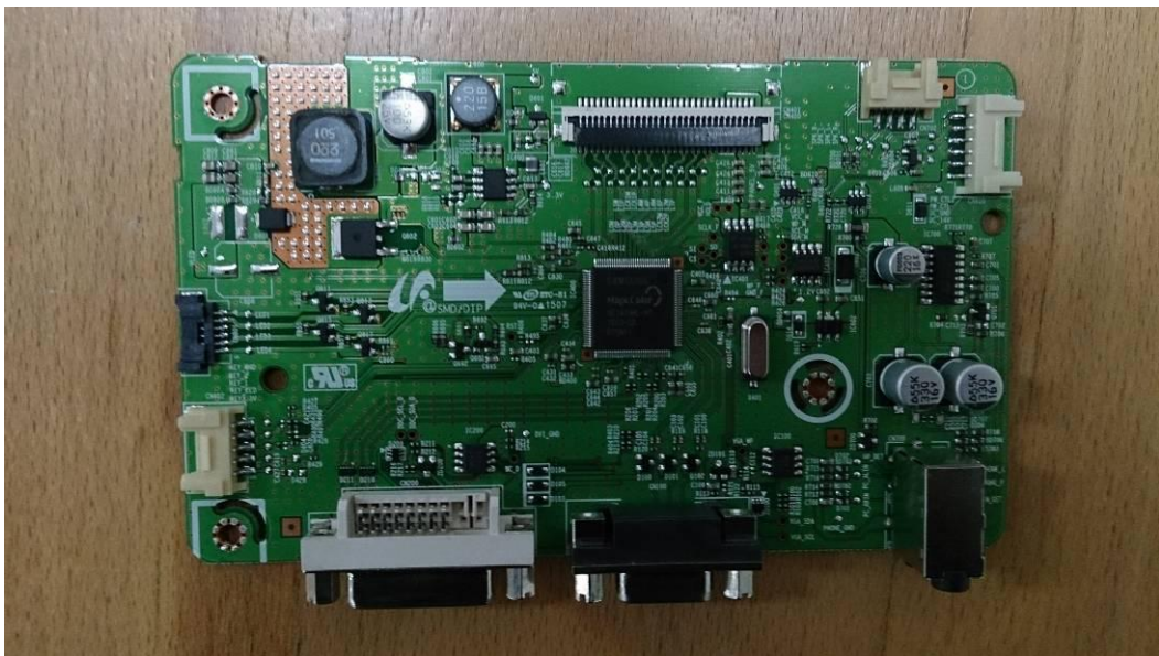
(Main Board )
