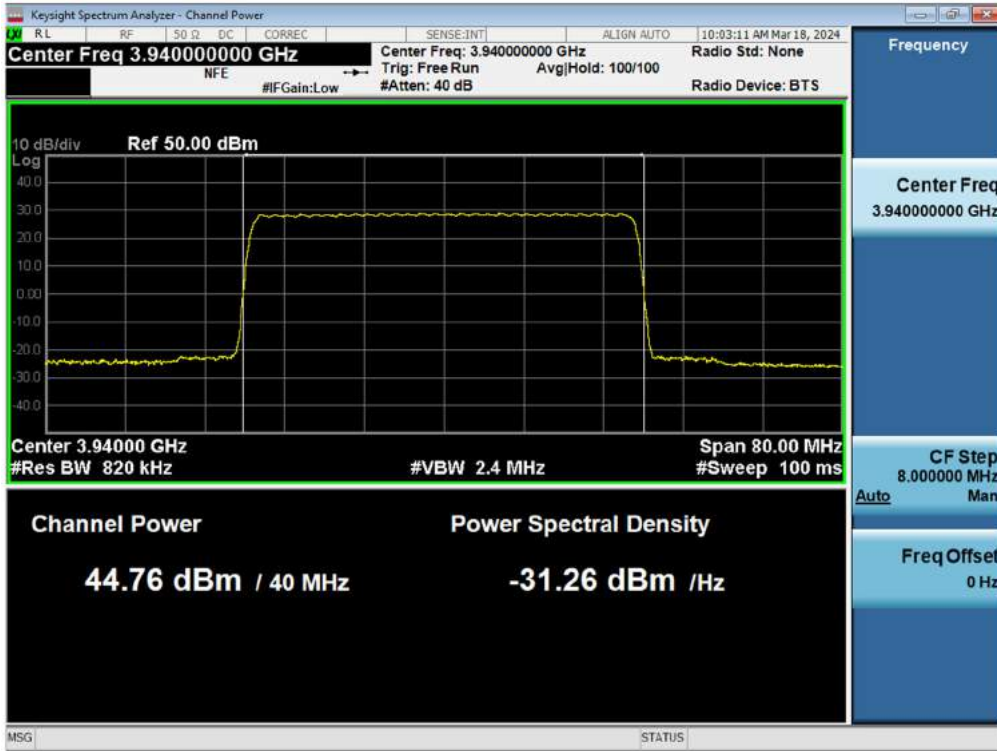
Antenna 6 / (8 Port) 5G NR n77 40 MHz 1 Carrier / QPSK / Middle
