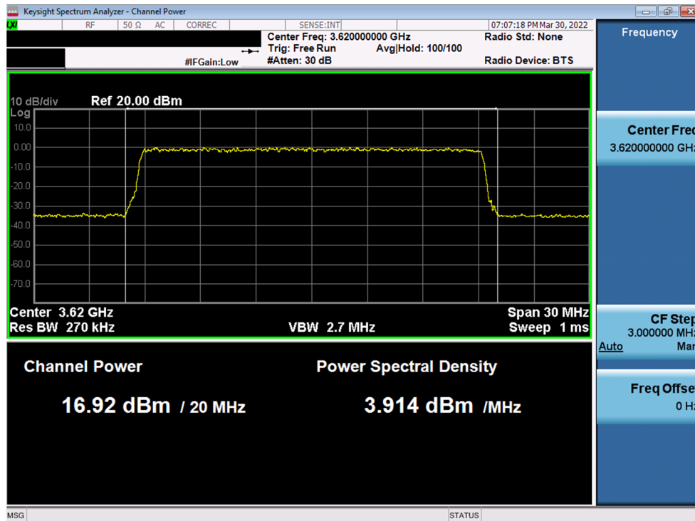
Plot 38. Conducted PSD, Mid-Channel SAS Granted maxEIRP 27 – ANT3
