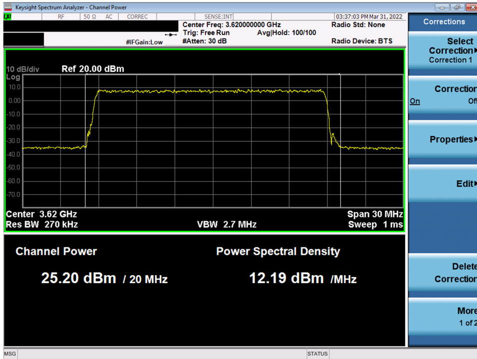
Plot 45. Conducted PSD, Mid-Channel SAS Granted maxEIRP 37 – ANT2
