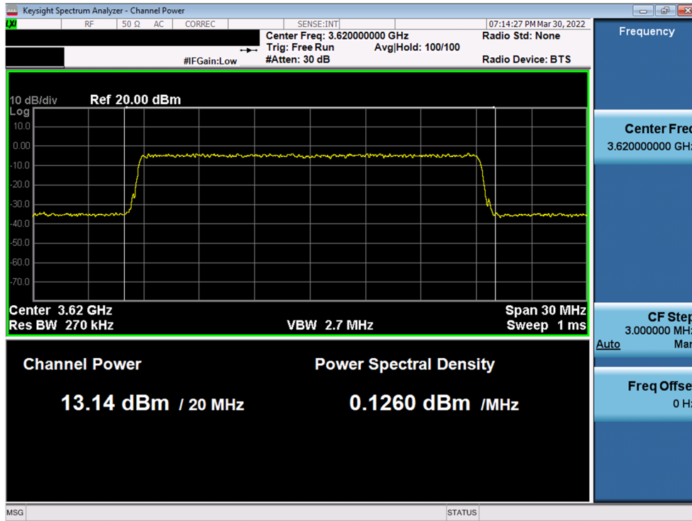
Plot 39. Conducted PSD, Mid-Channel SAS Granted maxEIRP 23 – ANT0
