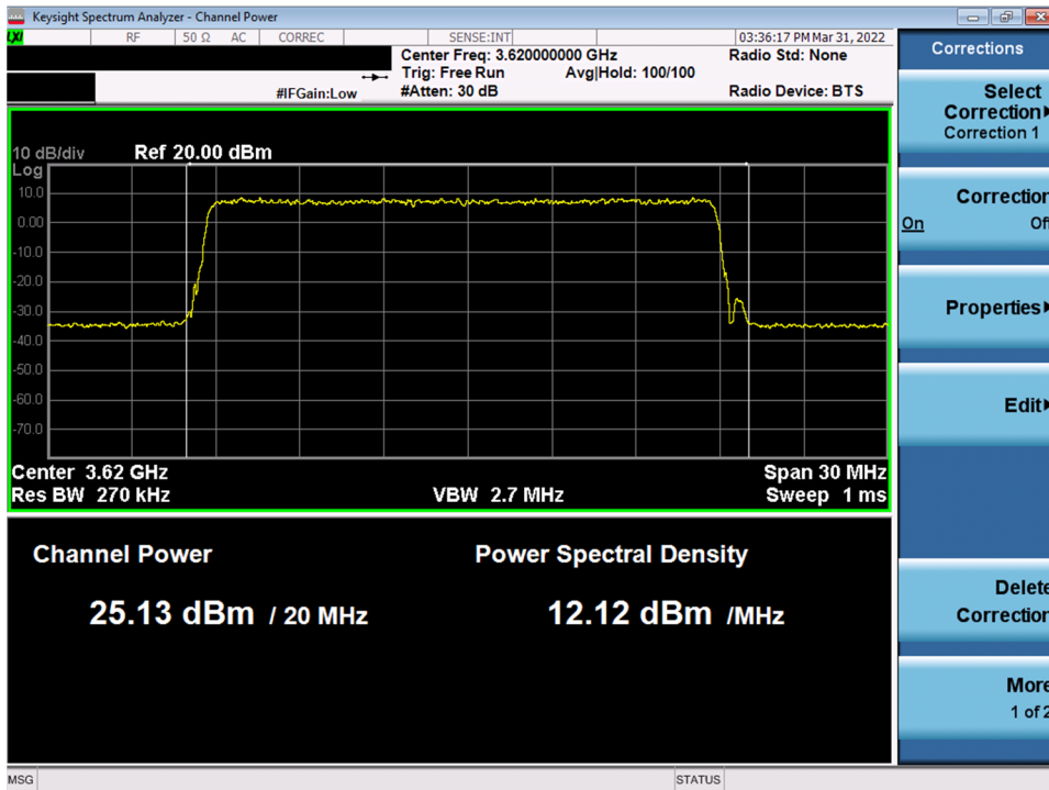
Plot 46. Conducted PSD, Mid-Channel SAS Granted maxEIRP 37 – ANT3
