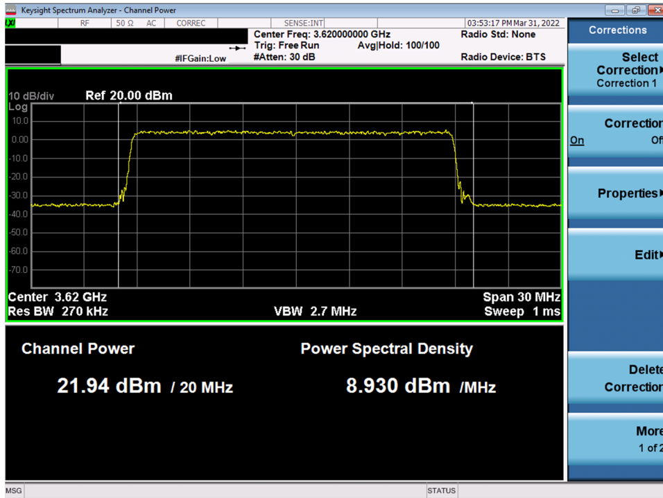
Plot 47. Conducted PSD, Mid-Channel SAS Granted maxEIRP 32 – ANT0
