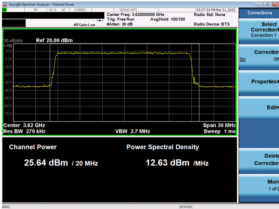
Plot 44. Conducted PSD, Mid-Channel SAS Granted maxEIRP 37 – ANT1
