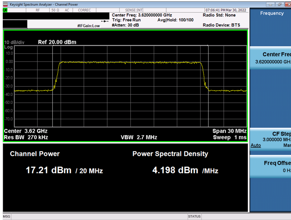
Plot 37. Conducted PSD, Mid-Channel SAS Granted maxEIRP 27 – ANT2
