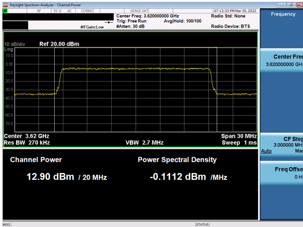
Plot 42. Conducted PSD, Mid-Channel SAS Granted maxEIRP 23 – ANT3
