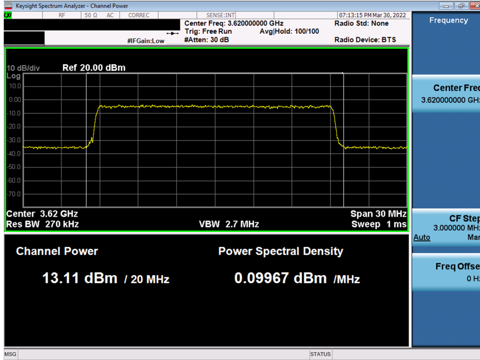
Plot 41. Conducted PSD, Mid-Channel SAS Granted maxEIRP 23 – ANT2
