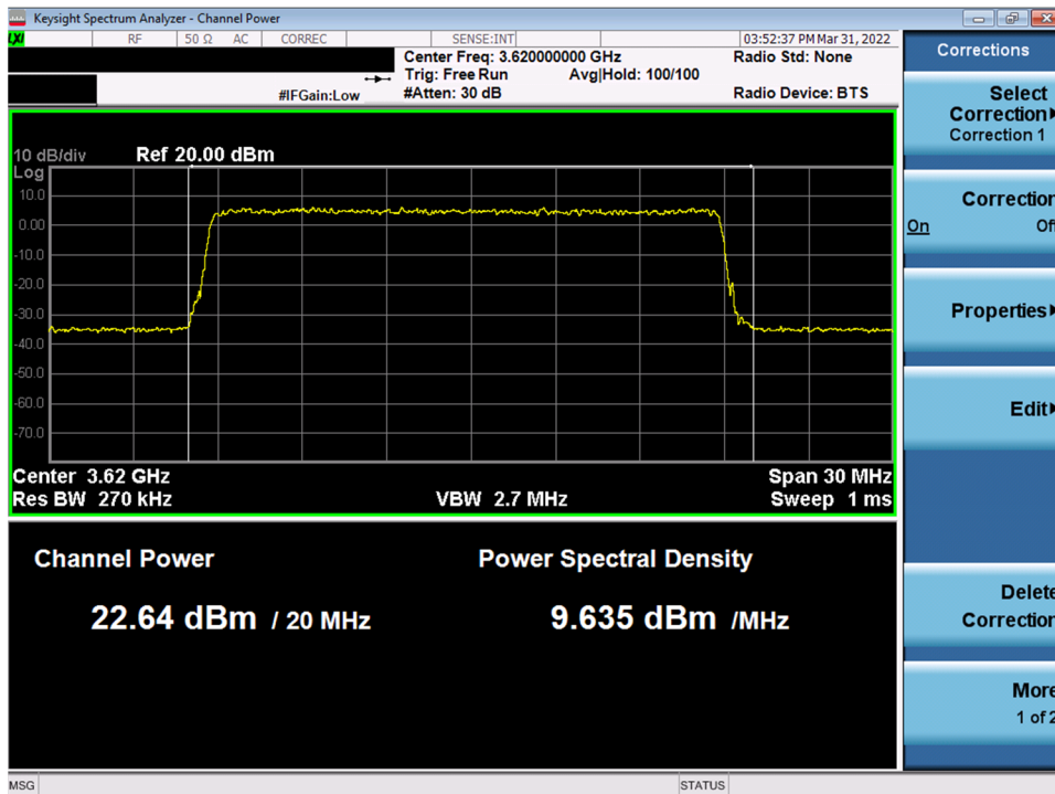
Plot 48. Conducted PSD, Mid-Channel SAS Granted maxEIRP 32 – ANT1
