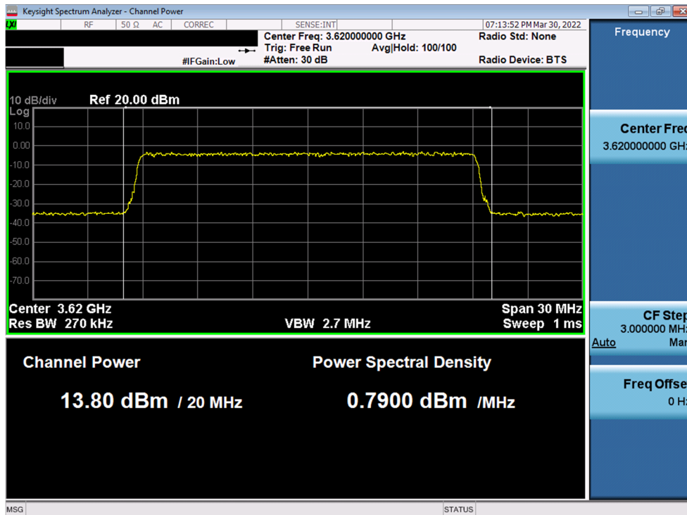
Plot 40. Conducted PSD, Mid-Channel SAS Granted maxEIRP 23 – ANT1
