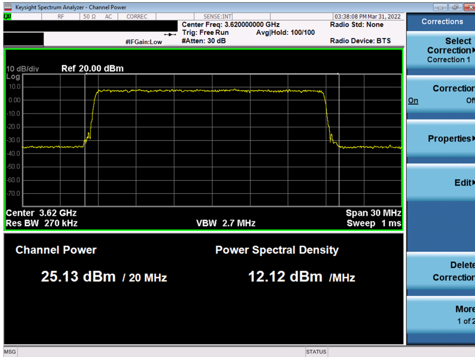
Plot 43. Conducted PSD, Mid-Channel SAS Granted maxEIRP 37 – ANT0
