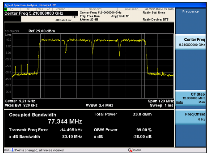
4CC UNII 1 BAND 26dB Bandwidth (QPSK 5210MHz)
