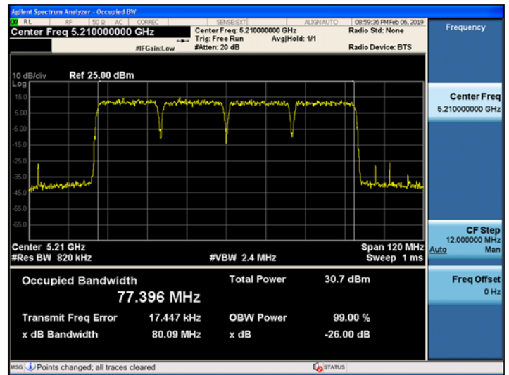
4CC UNII 1 BAND 26dB Bandwidth (256QAM 5210MHz)
