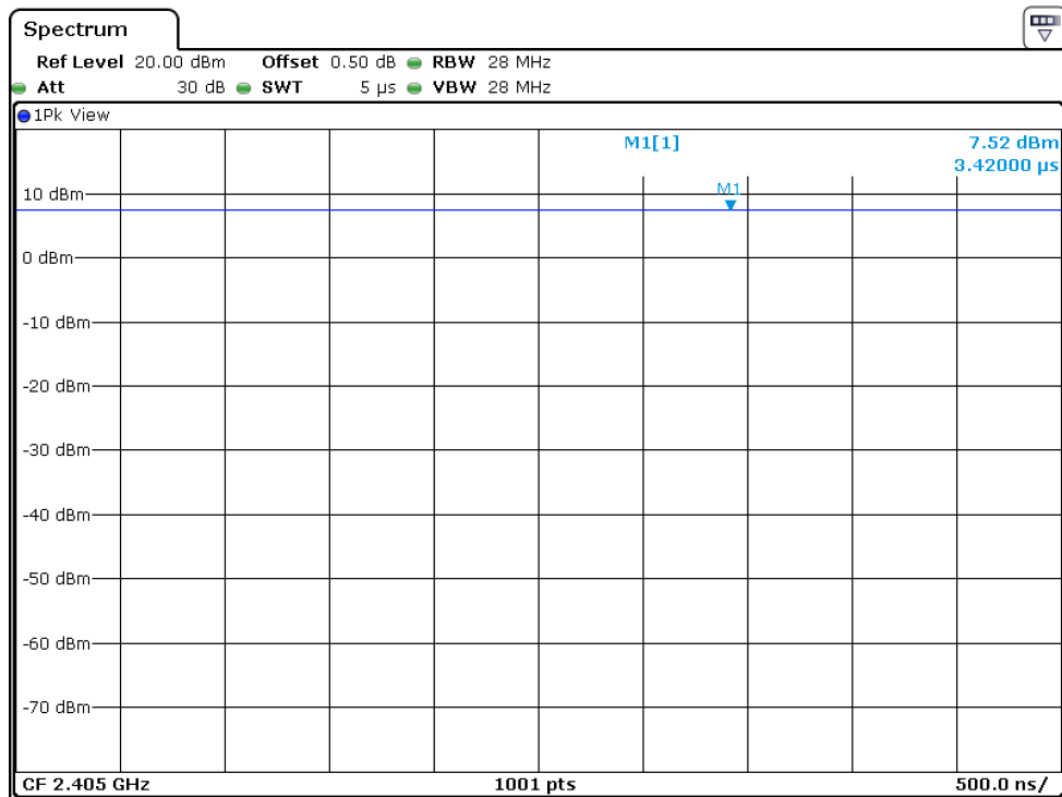
Figure 8-1 Zigbee Transmission Plot
