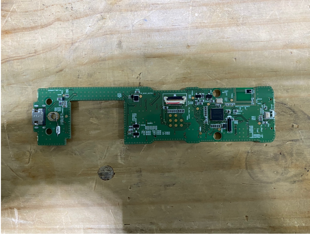
Main PCB_F
