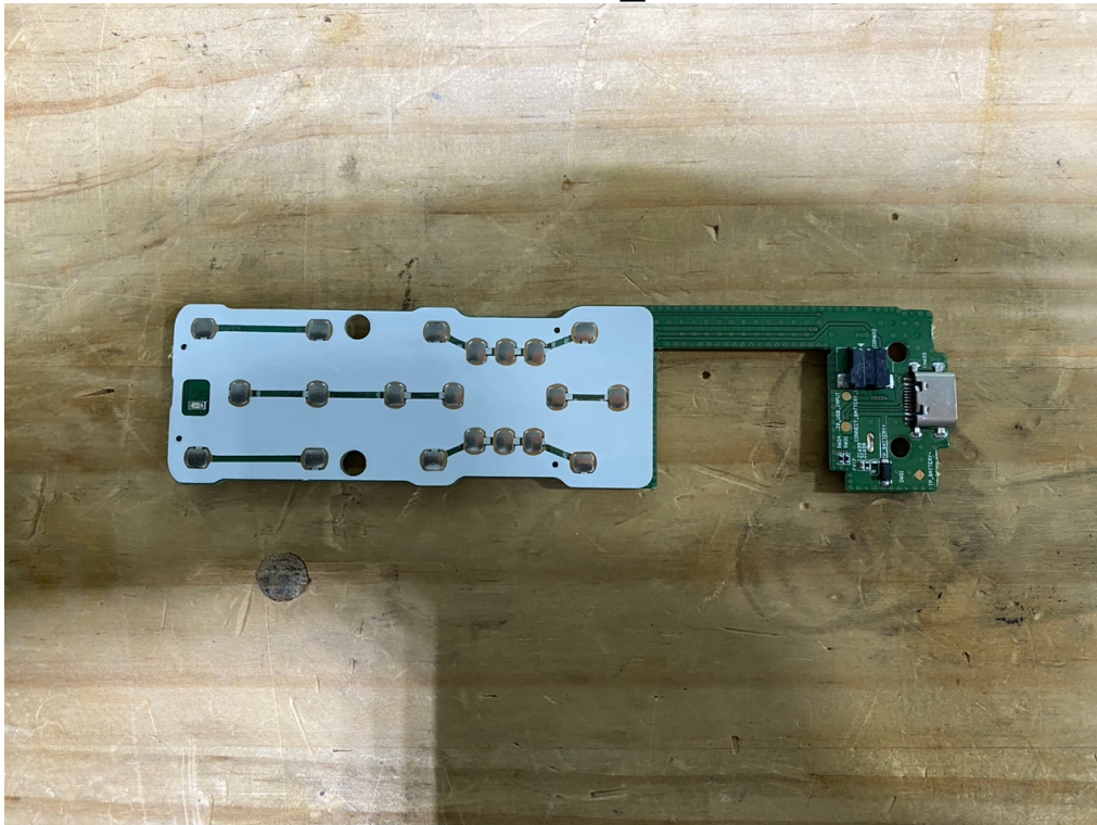
Main PCB_R
