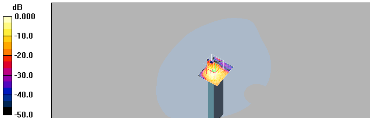
0 dB = 0.087mW/g
