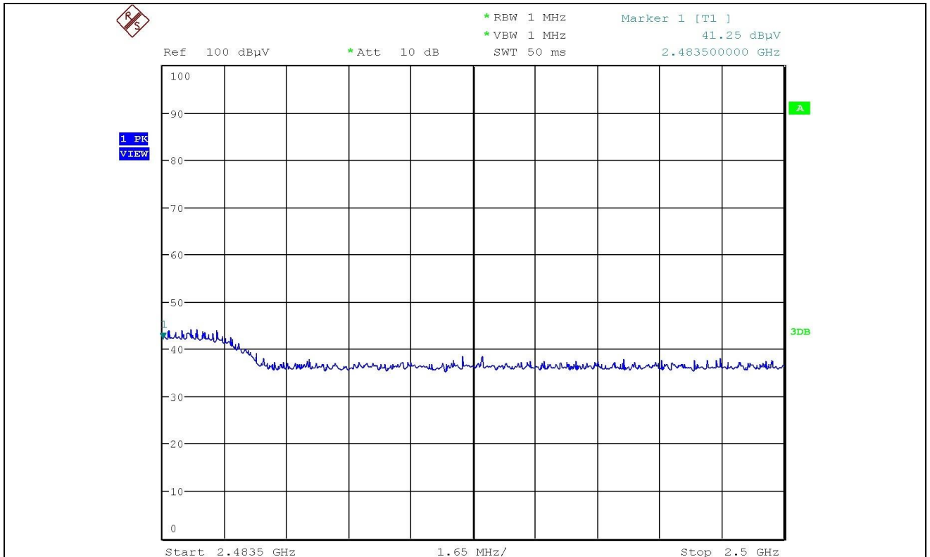
2 483.50 _ Peak _ V
