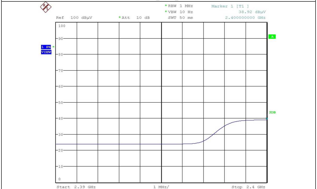
2 400.00 _ Average _ H
