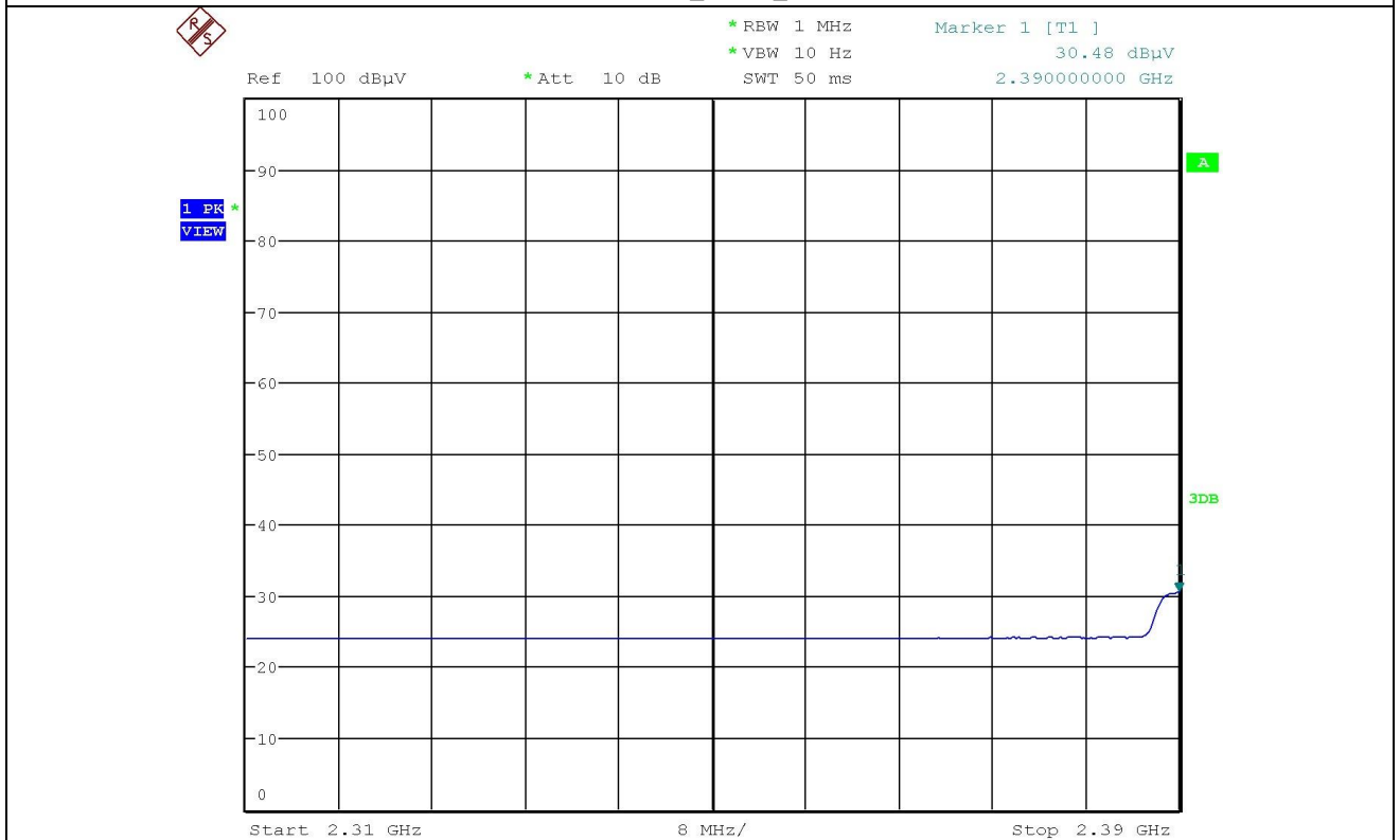
2 390.00 _ Average _ V
