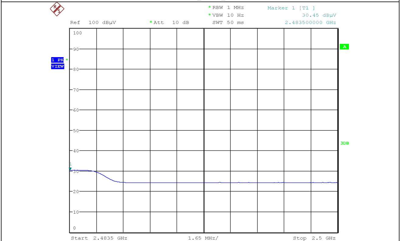
2 483.50 _ Average _ H
