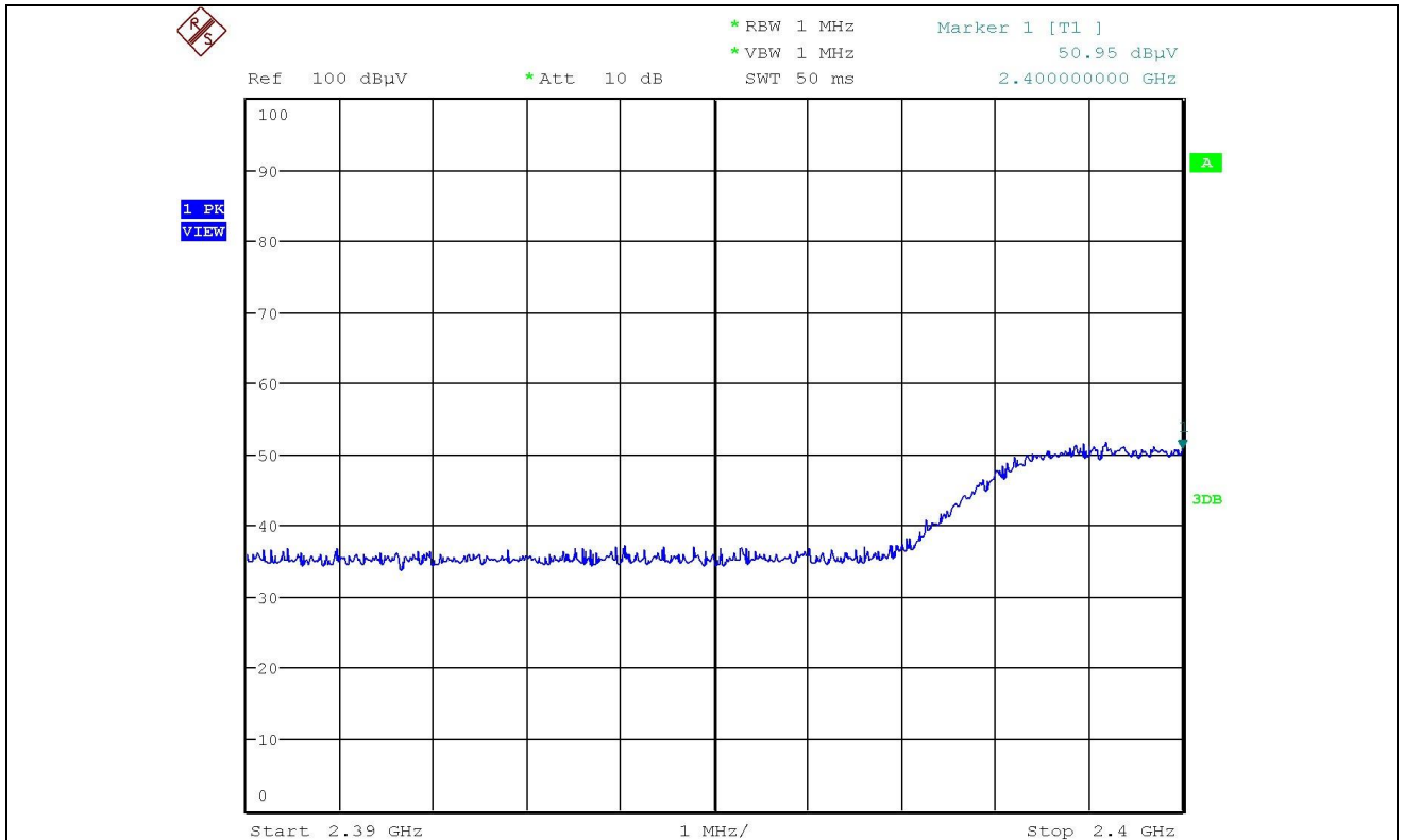
2 400.00 _ Peak _ V
