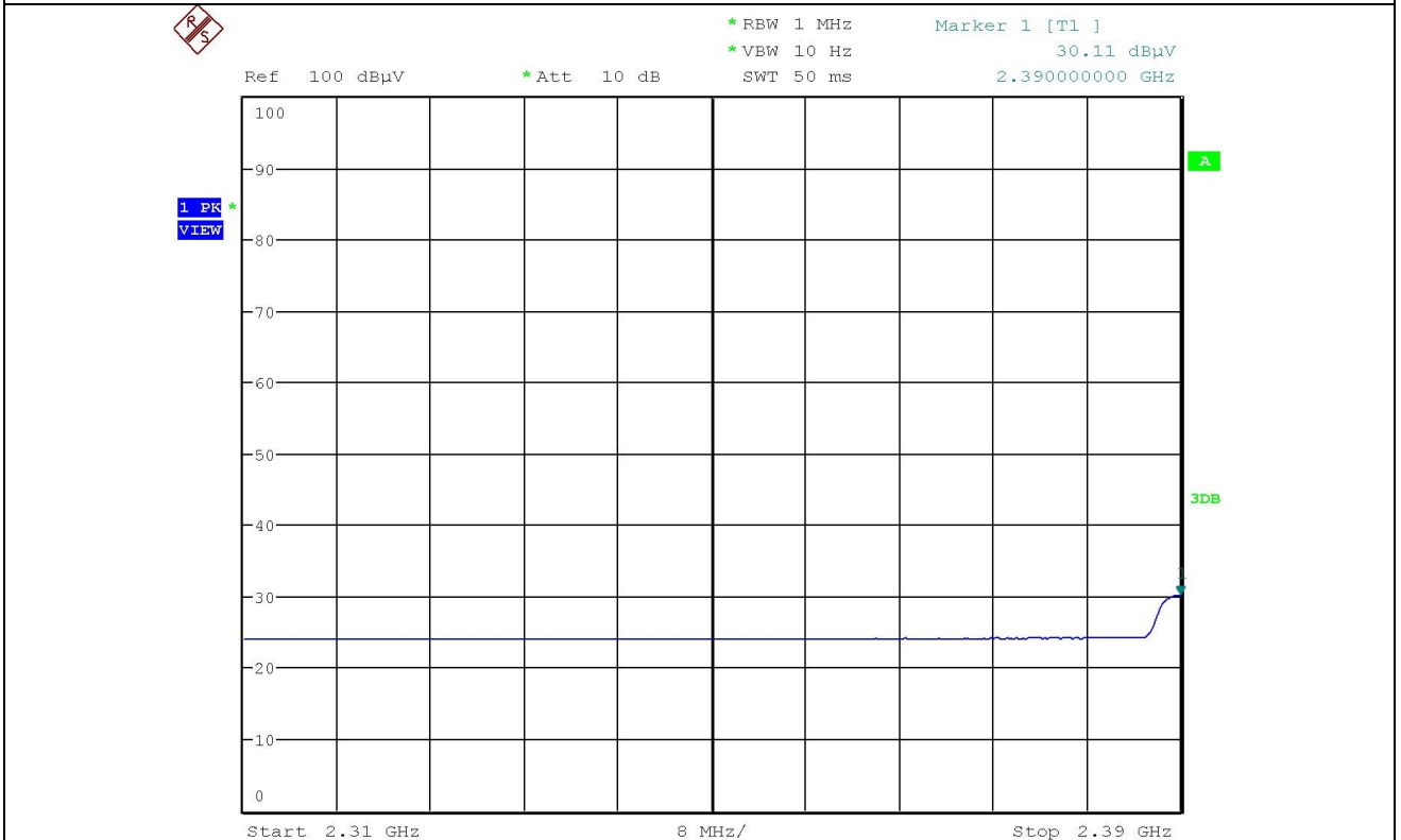
2 390.00 _ Average _ H
