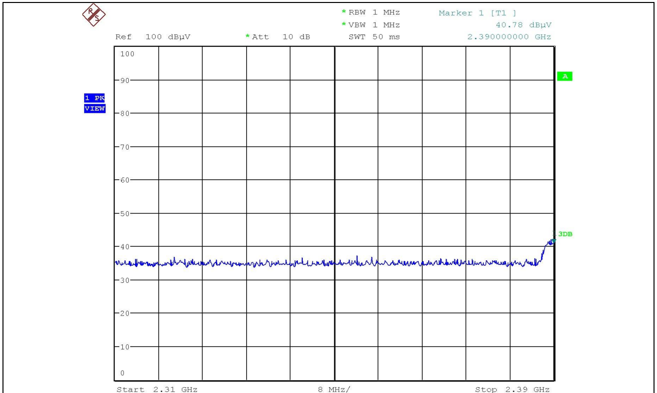
2 390.00 _ Peak _ V
