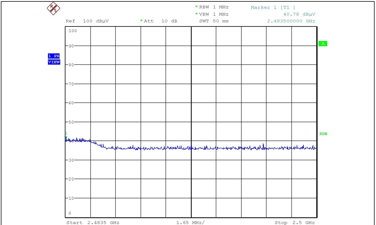
2 483.50 _ Peak _ H
