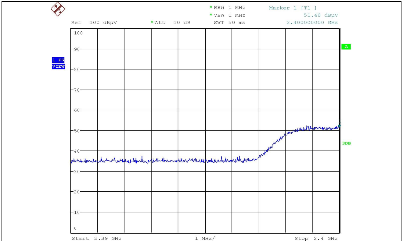
2 400.00 _ Peak _ H
