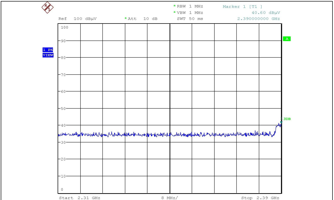
2 390.00 _ Peak _ H
