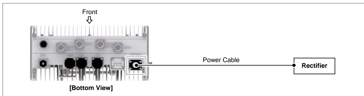
Figure 53. Connecting Power Cable (1)
