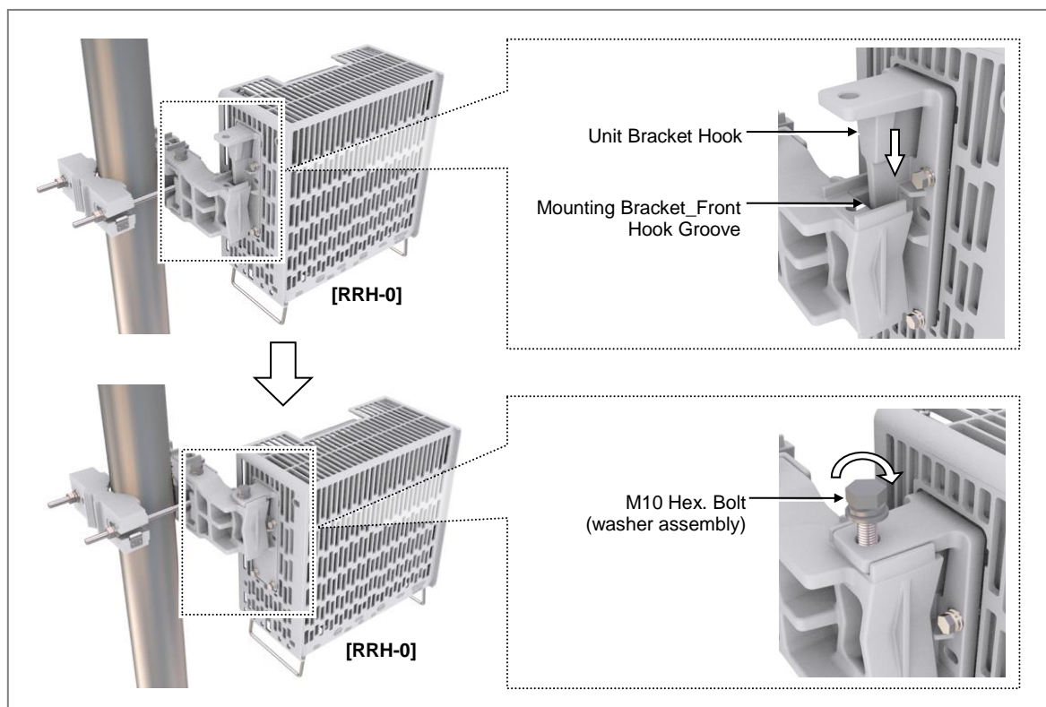
Figure 32. Fixing RRH_3 Sector Pole Type (1)
