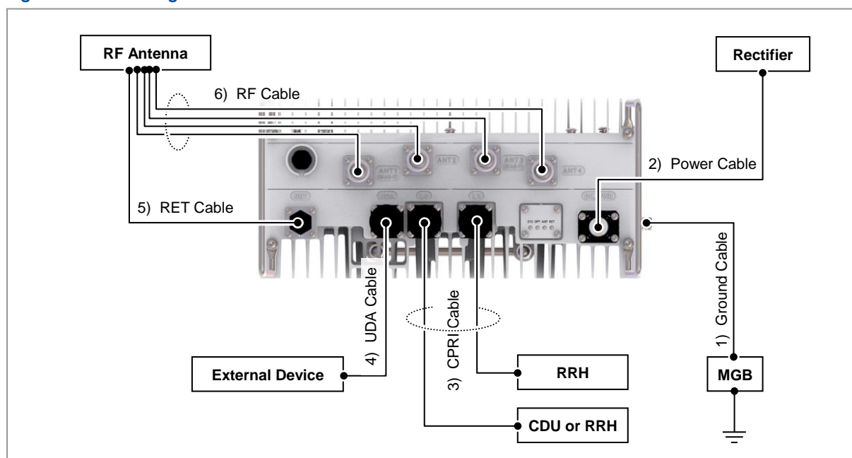
Figure 49. Cable Diagram
