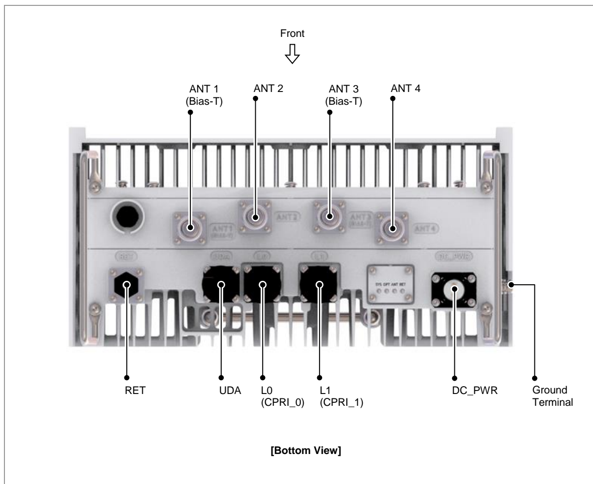
Figure 3. RRH External Interface
