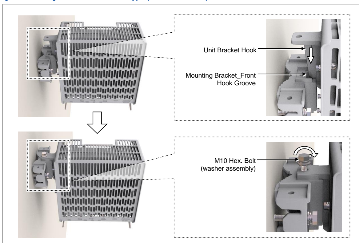
Figure 42. Fixing RRH_1 Sector Pole Type (Side Installation)
