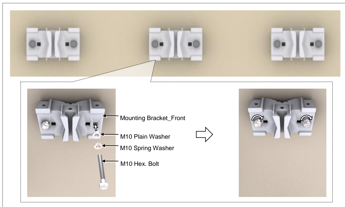
Figure 39. Fixing Mounting Bracket_3 Sector Wall Type (Standard Installation)
