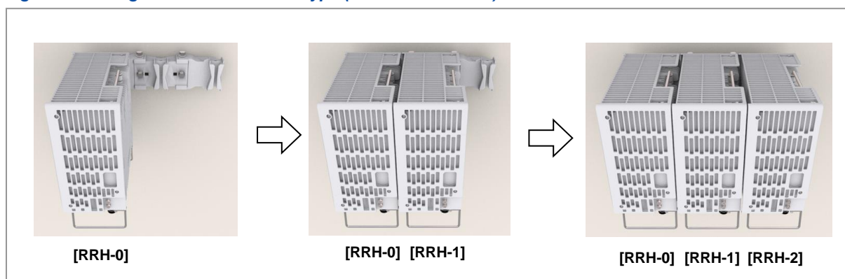
Figure 46. Fixing RRH_3 Sector Wall Type (Side Installation 2)
