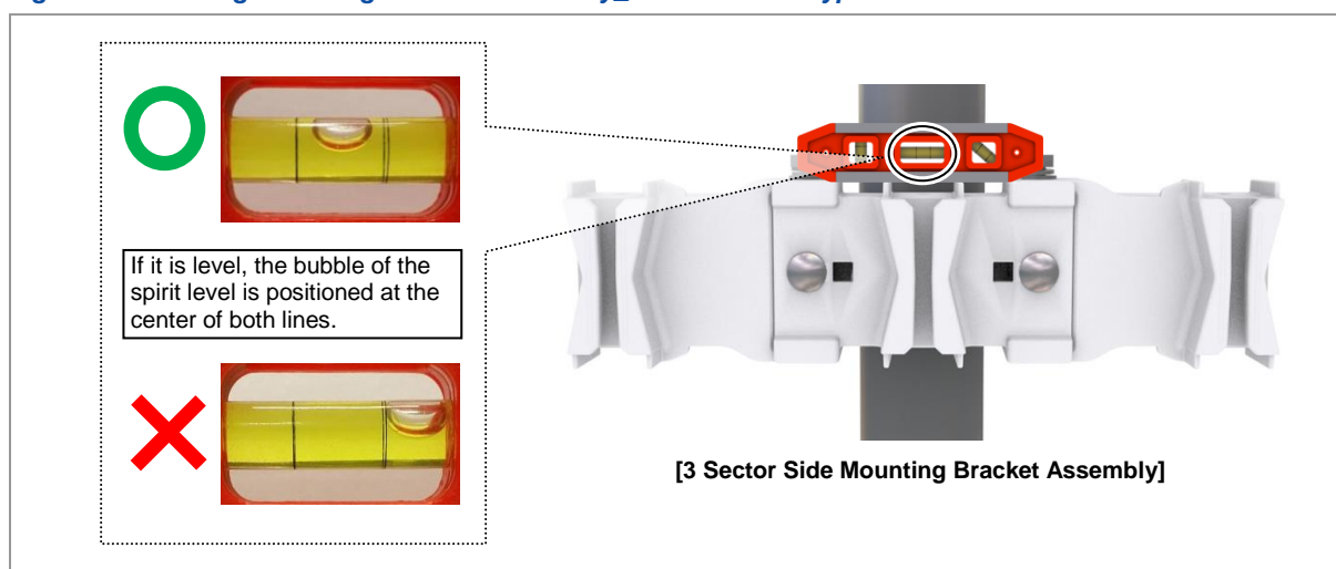
Figure 29. Leveling Mounting Bracket Assembly_3 Sector Pole Type
