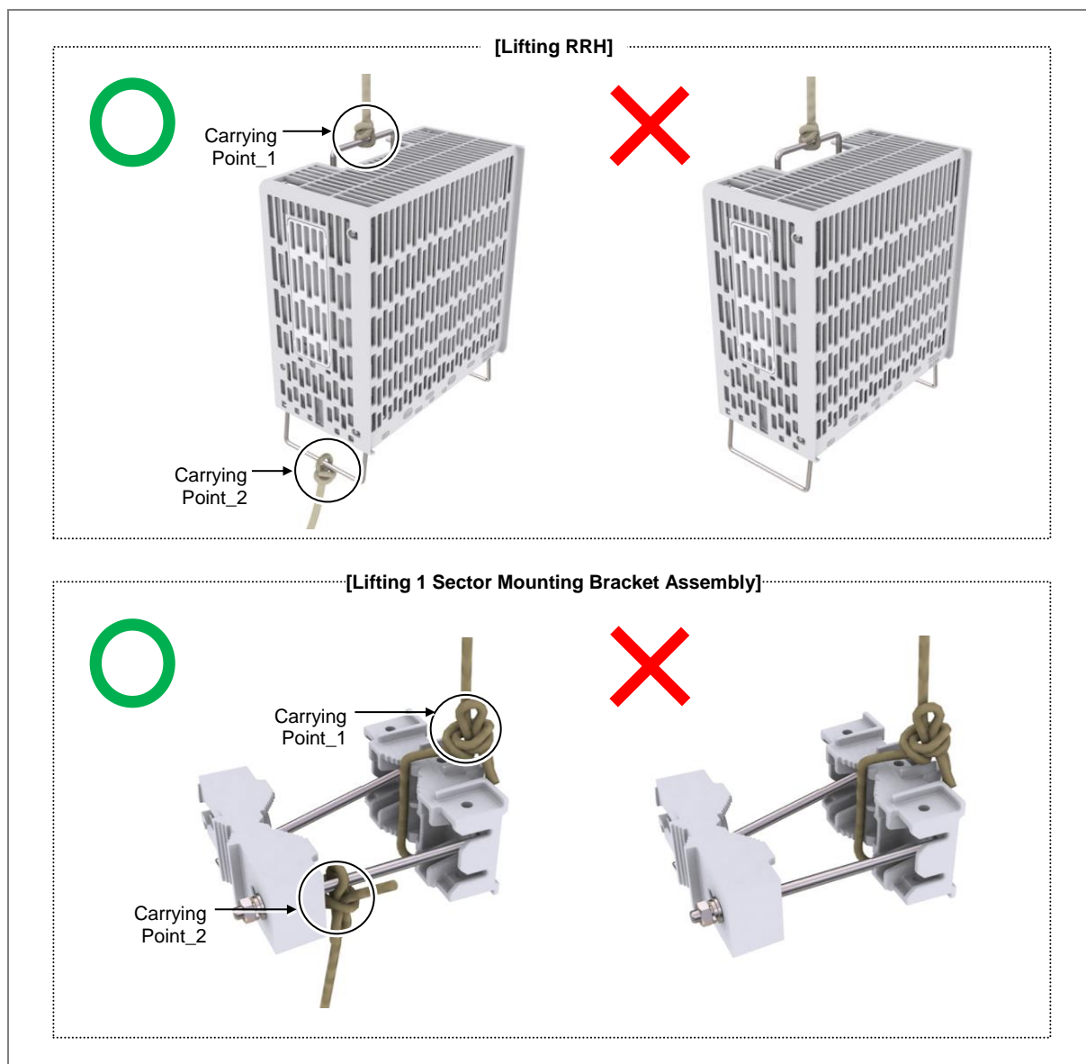
Figure 22. Lifting RRH &amp; Mounting Bracket Assembly_Pole Type
