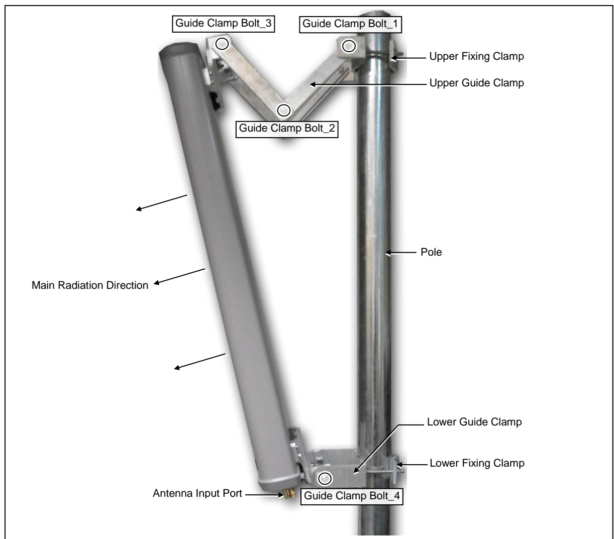
Figure 82. Sector Antenna
