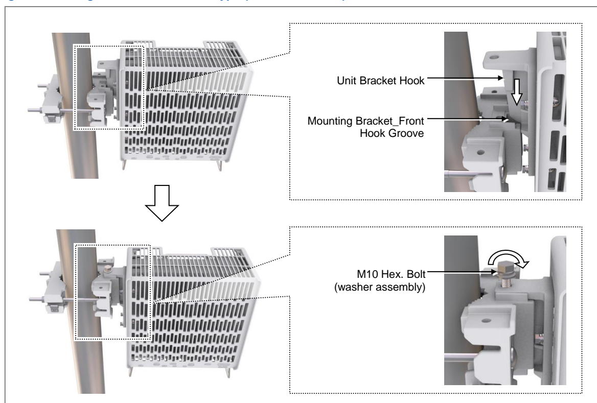
Figure 31. Fixing RRH_1 Sector Pole Type (Side Installation)
