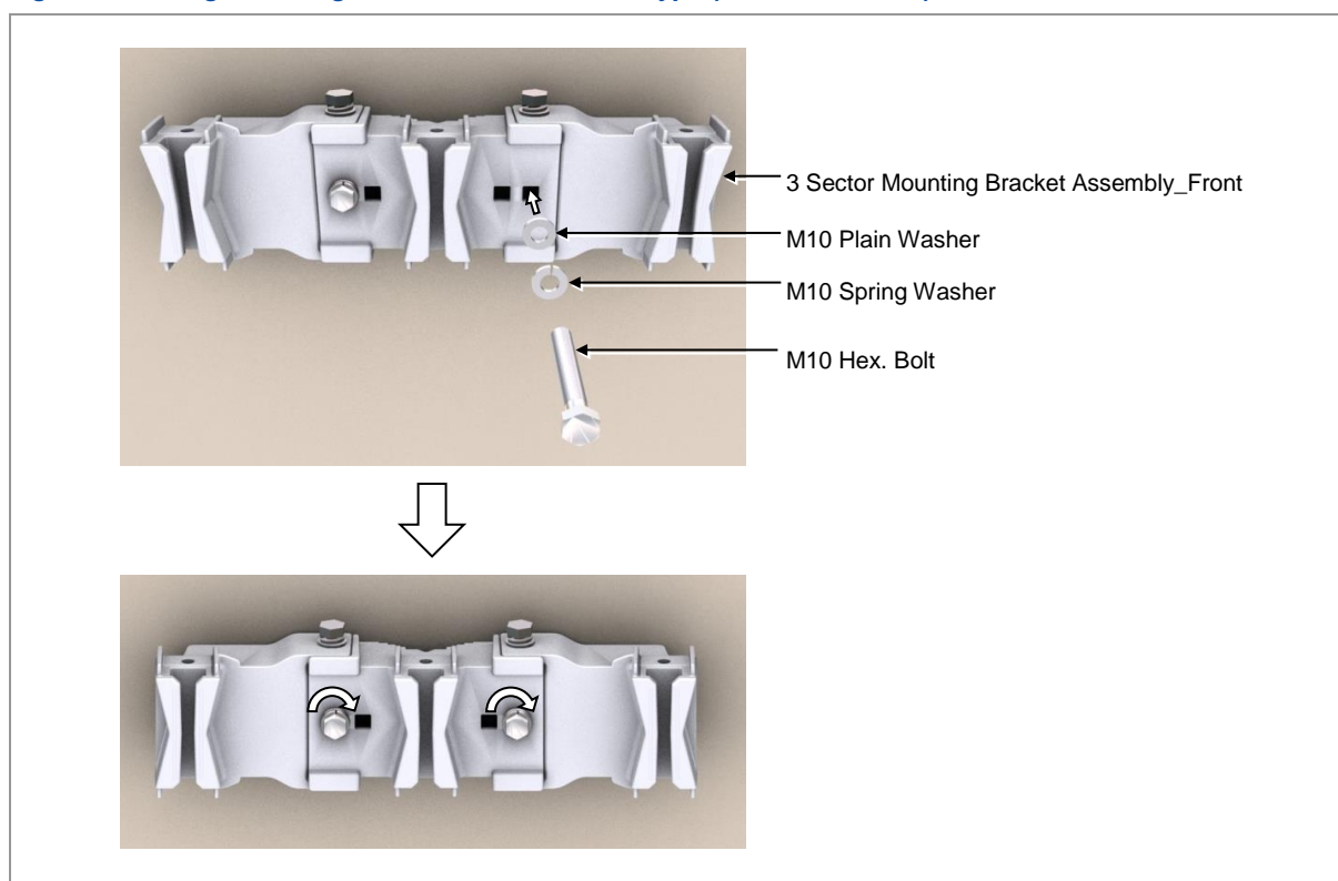
Figure 40. Fixing Mounting Bracket_3 Sector Wall Type (Side Installation)
