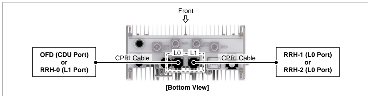
Figure 60. Connecting CPRI Cable_Cascade connection-oriented (1)
