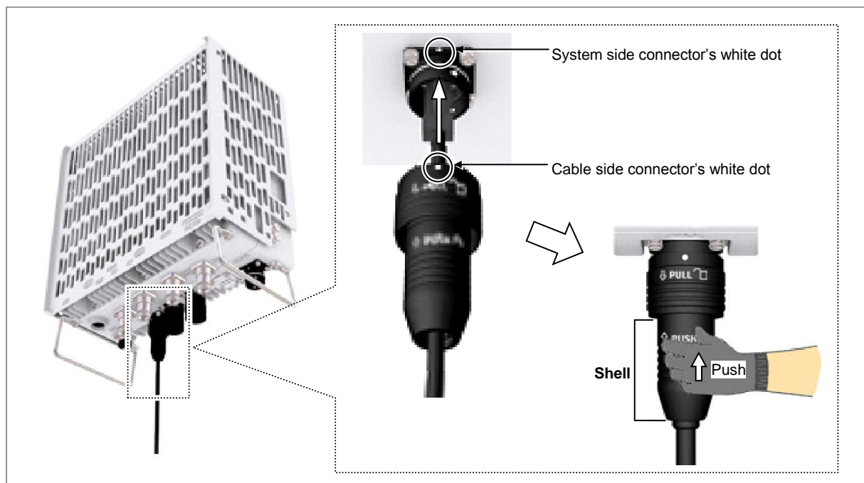
Figure 73. Connecting UDA Cable (6)
