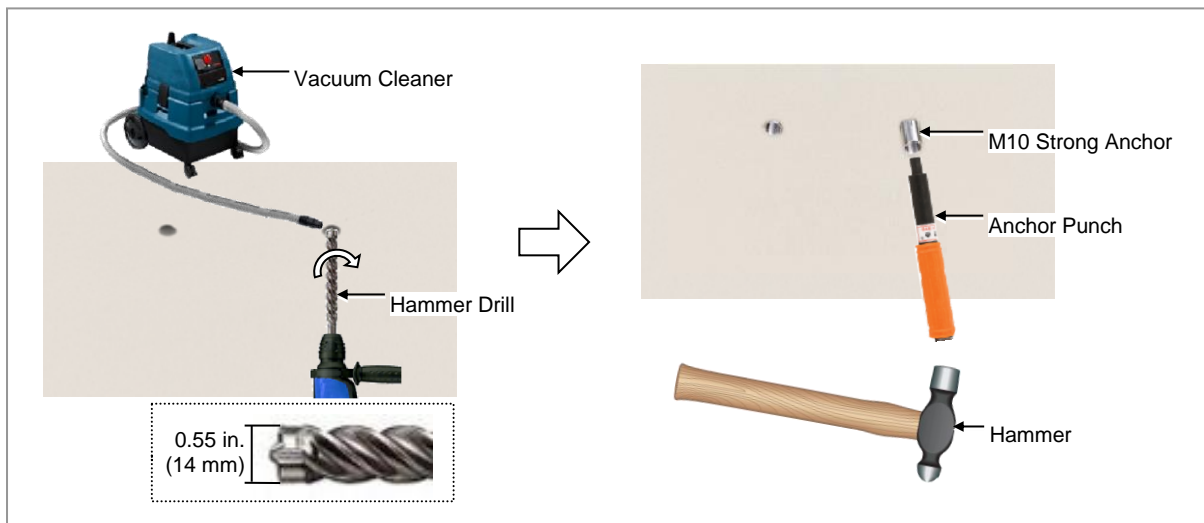
Figure 37. Drilling & Anchoring
