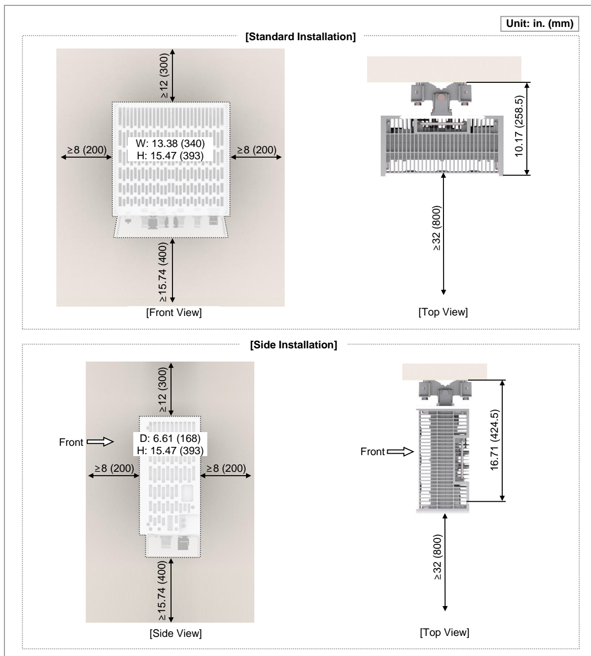
Figure 7. RRH Arrangement_1 Sector Wall Type Installation
