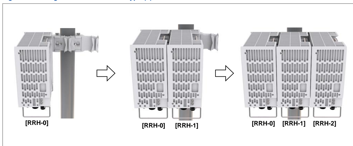
Figure 33. Fixing RRH_3 Sector Pole Type (2)
