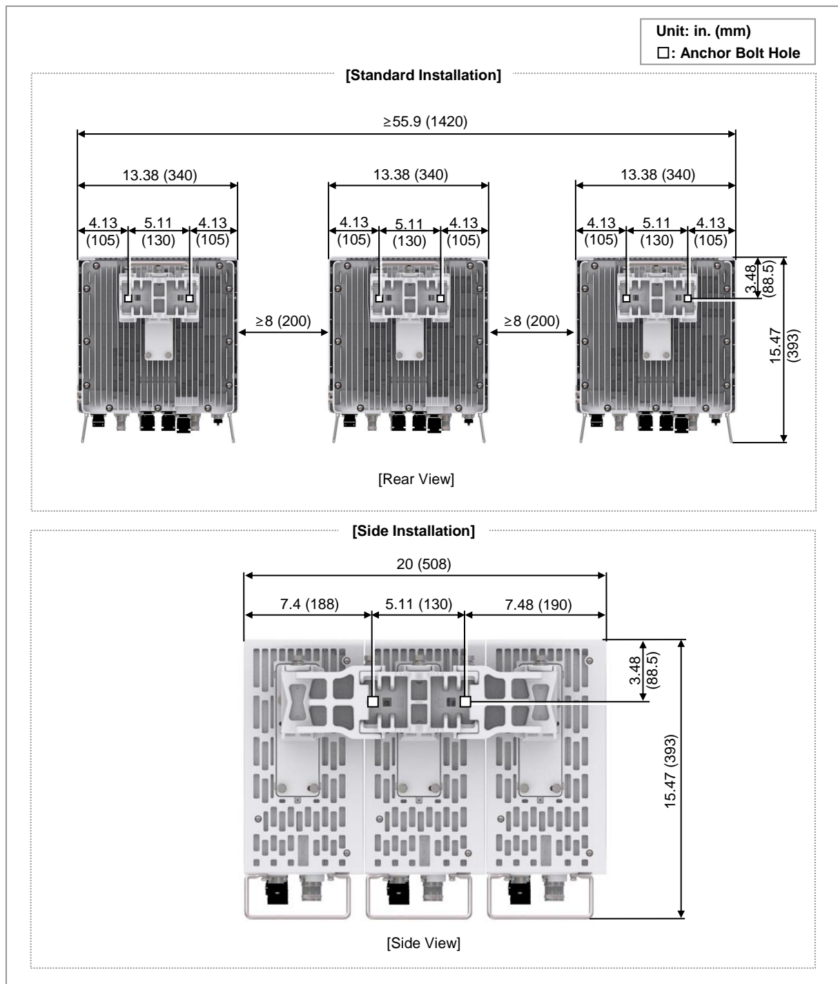
Figure 35. RRH marking dimensions_3 Sector Wall Type
