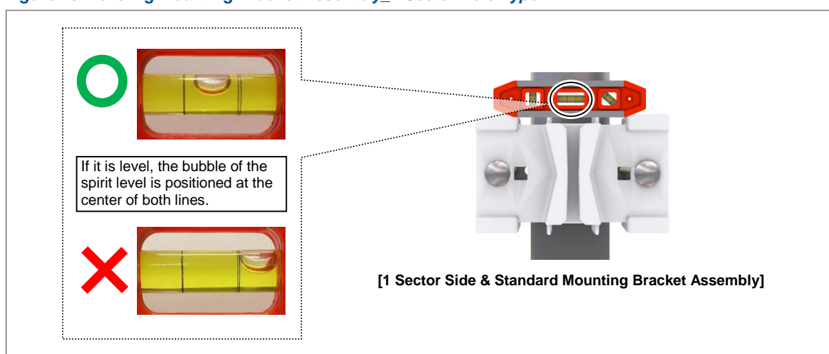
Figure 26. Leveling Mounting Bracket Assembly_1 Sector Pole Type
