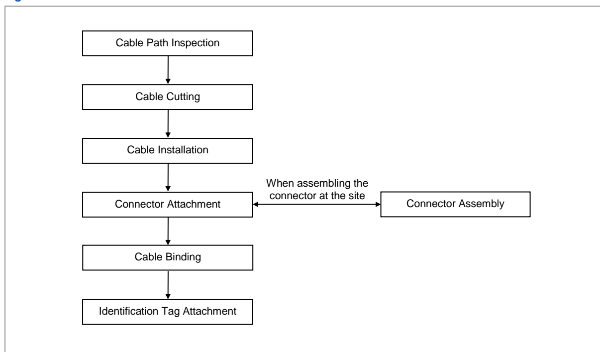
Figure 48. Cable Connection Procedure
