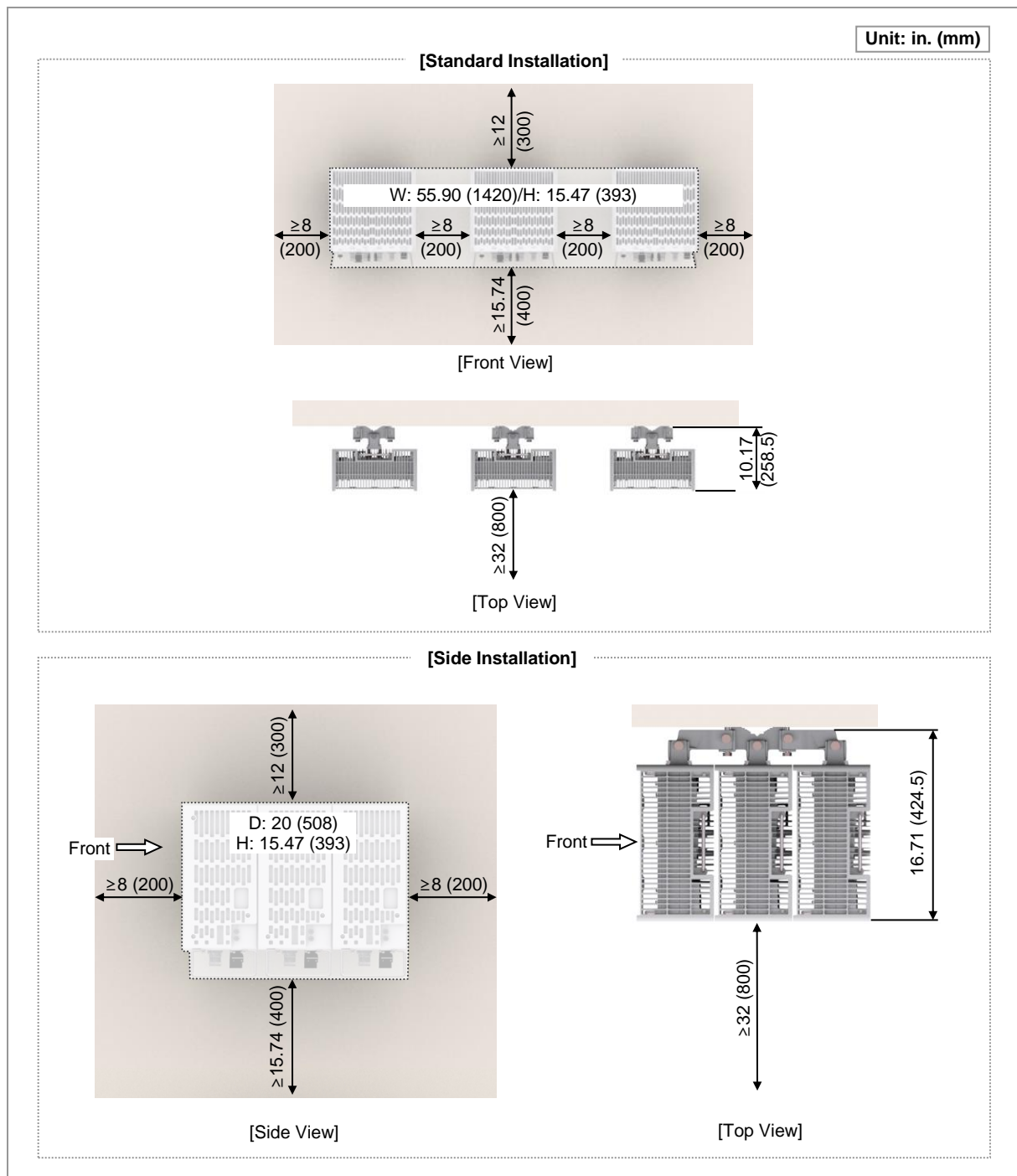
Figure 8. RRH Arrangement_3 Sector Wall Type Installation
