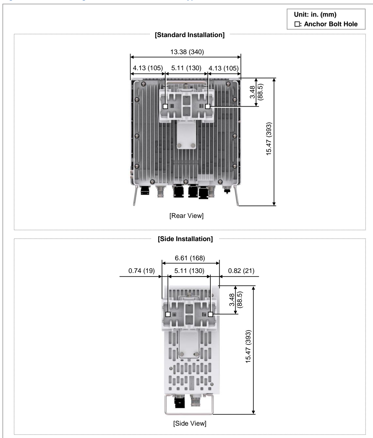
Figure 34. RRH marking dimensions_1 Sector Wall Type
