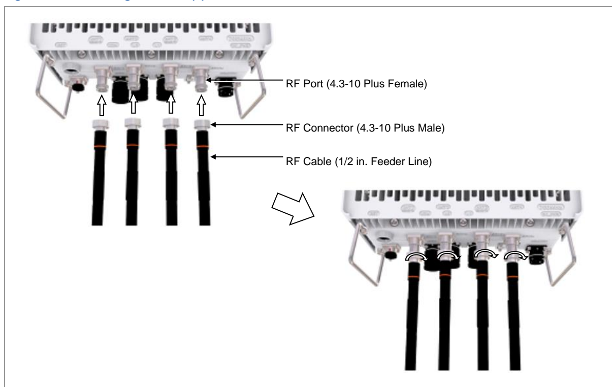
Figure 80. Connecting RF Cable (3)
