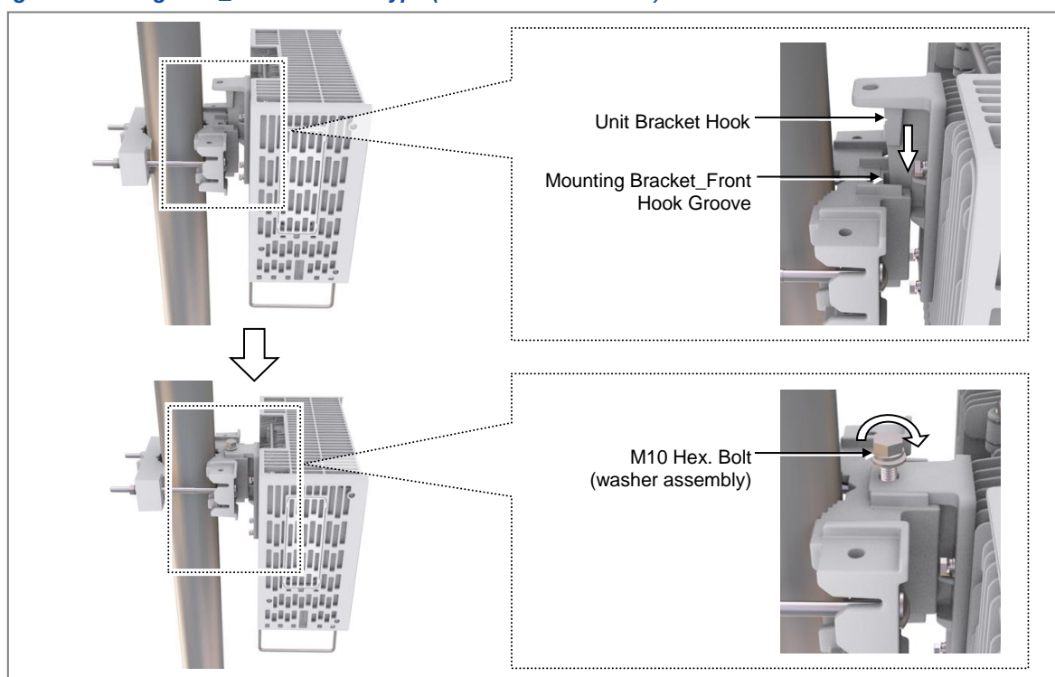
Figure 30. Fixing RRH_1 Sector Pole Type (Standard Installation)
