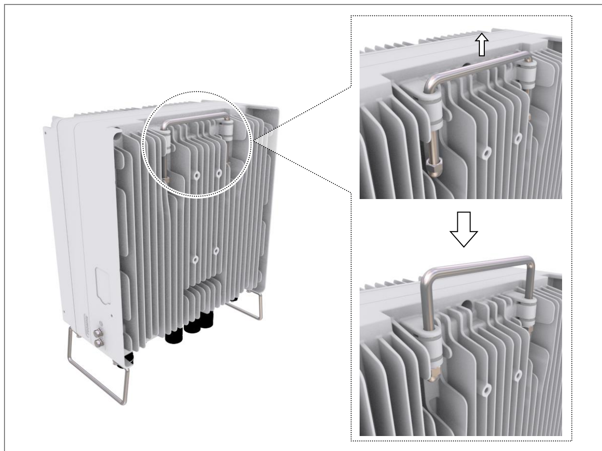
Figure 9. Using a Handle to transport an RRH
