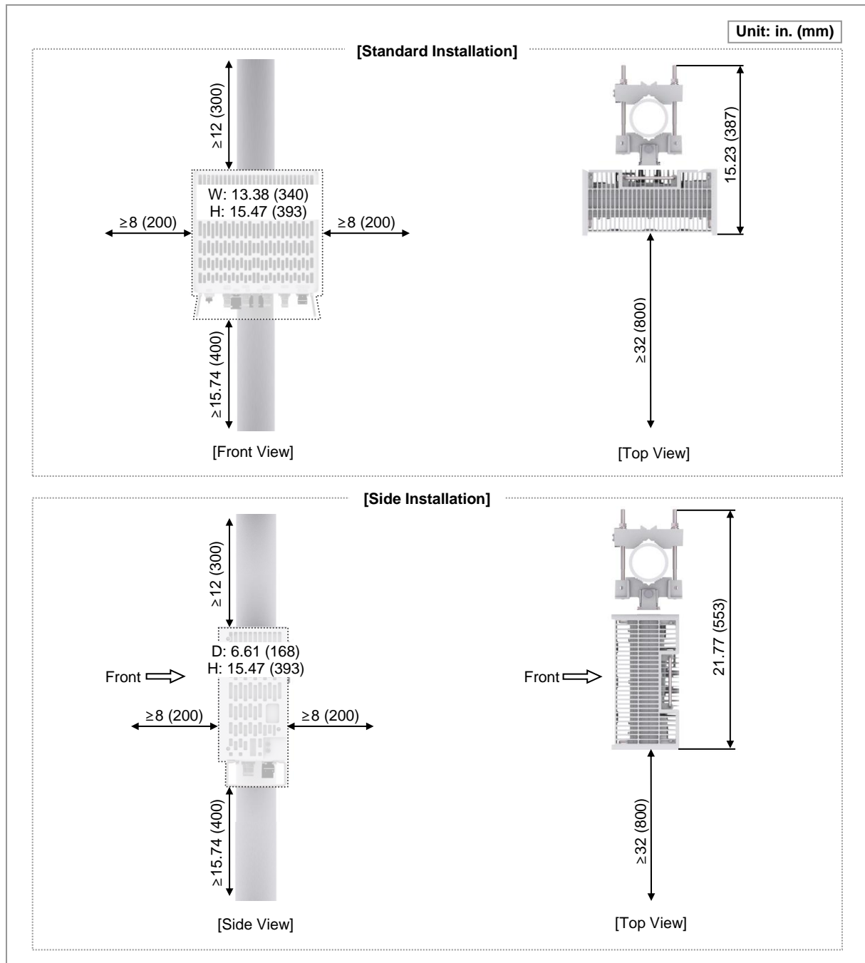
Figure 5. RRH Arrangement_1 Sector Pole Type Installation
