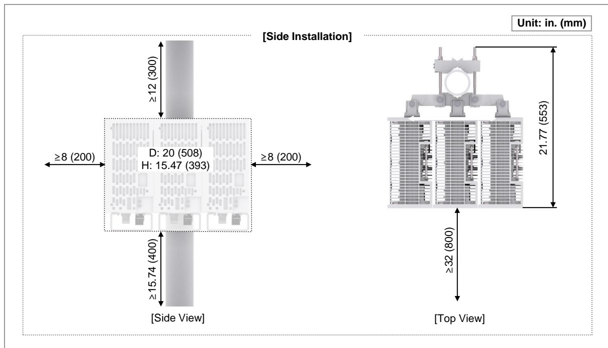
Figure 6. RRH Arrangement_3 Sector Pole Type Installation
