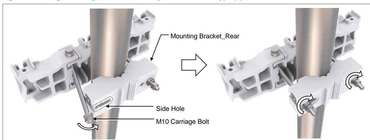
Figure 28. Fixing Mounting Bracket Assembly_3 Sector Pole Type (2)
