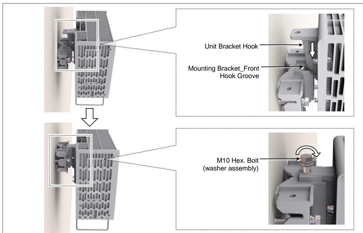
Figure 41. Fixing RRH_1 Sector Wall Type (Standard Installation)
