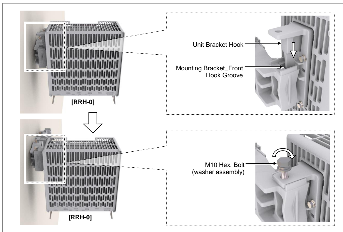
Figure 45. Fixing RRH_3 Sector Wall Type (Side Installation 1)
