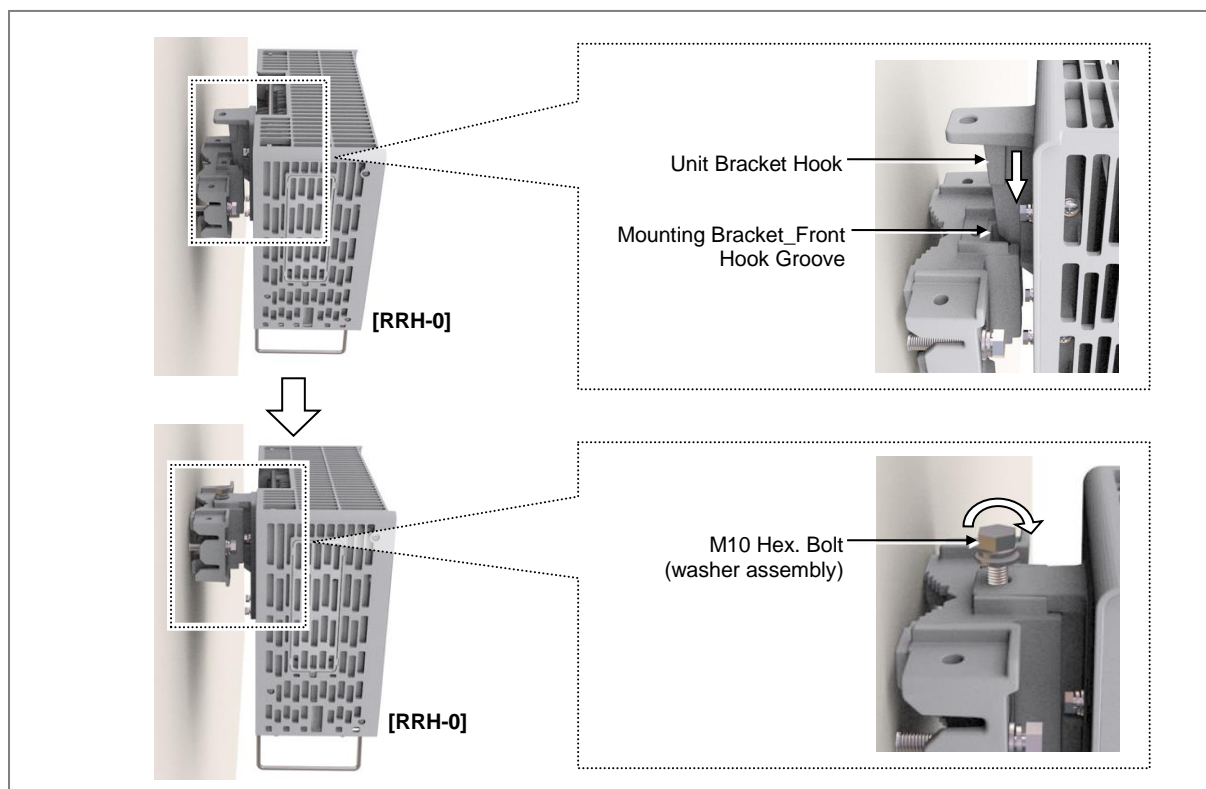
Figure 43. Fixing RRH_3 Sector Wall Type (Standard Installation 1)
