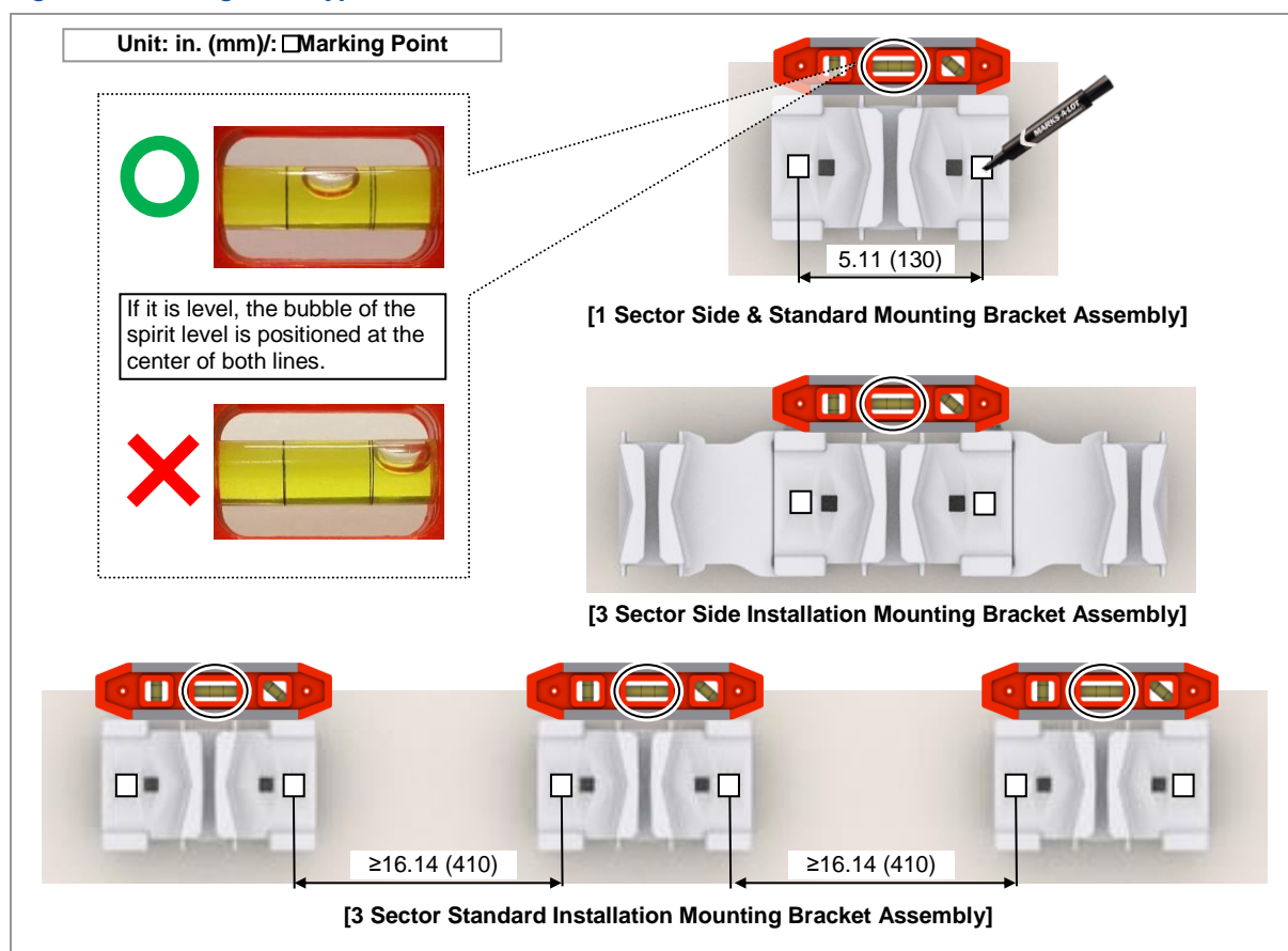
Figure 36. Marking_Wall Type
