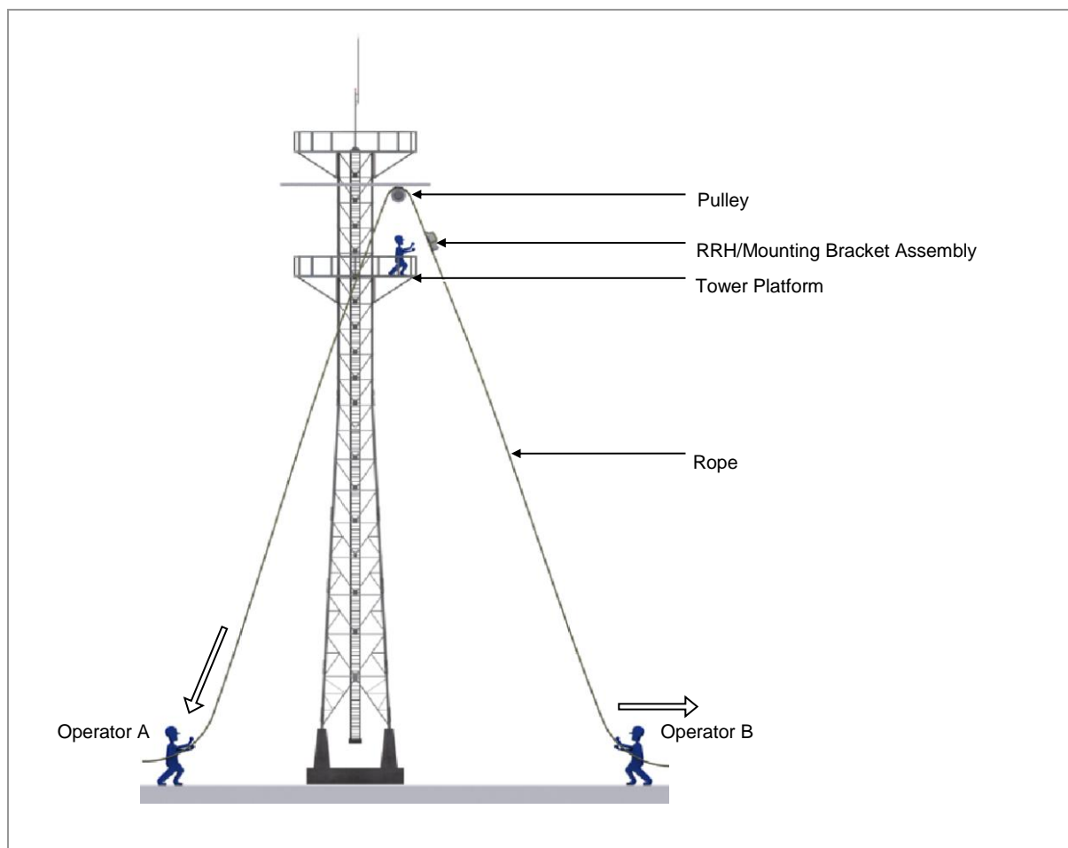
Figure 23. Lifting RRH &amp; Mounting Bracket Assembly_Pole Type
