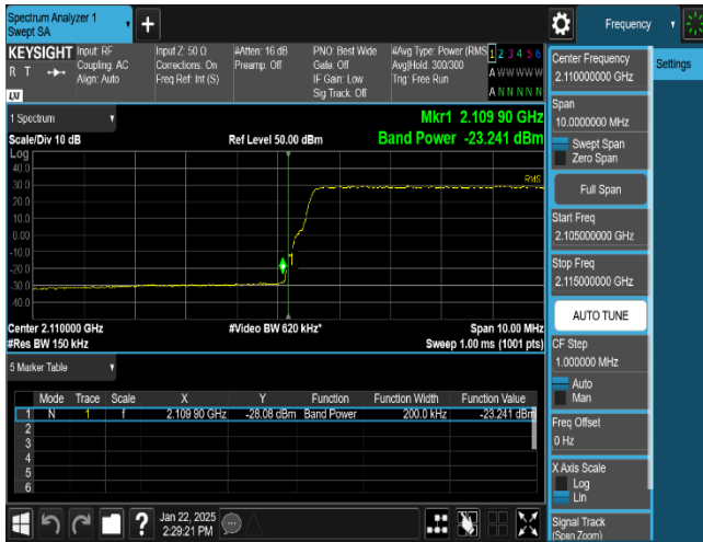
Plot 8-63. Band Edge Emission Summary Data Plot (B(n)66_2C_LTE_10M+NR_10M_QPSK -Low Edge, Port 1)
