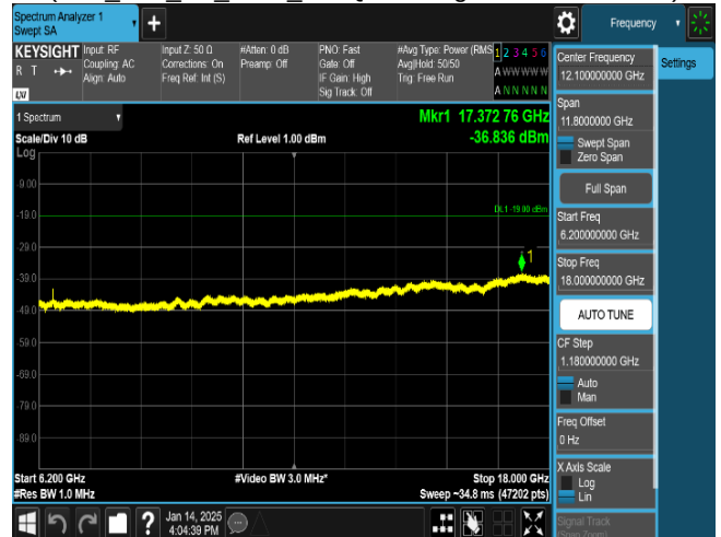
Plot 8-83. Conducted Spurious Emission Plot 6.2 GHz to 18 GHz
