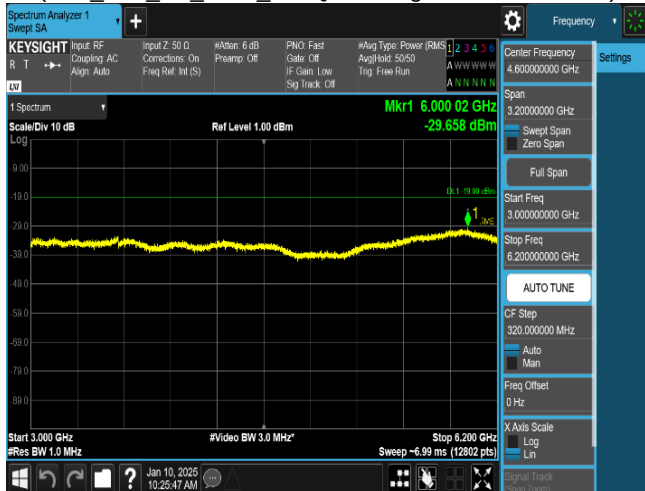
Plot 8-82. Conducted Spurious Emission Plot 3 GHz to 6.2 GHz
