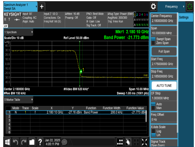
Plot 8-64. Band Edge Emission Summary Data Plot (B(n)66_2C_LTE_10M+NR_10M_QPSK -High Edge, Port 0)
