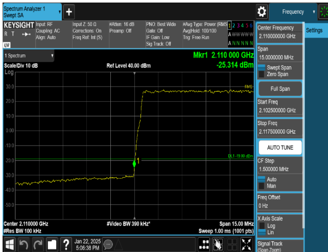
Plot 8-65. Band Edge Emission Summary Data Plot (B(n)66_2NC_LTE_10M+NR_10M_QPSK -Low Edge, Port 3)
