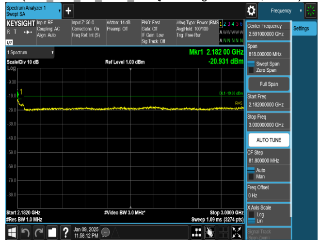
Plot 8-81. Conducted Spurious Emission Plot 2.182 GHz to 3 GHz
