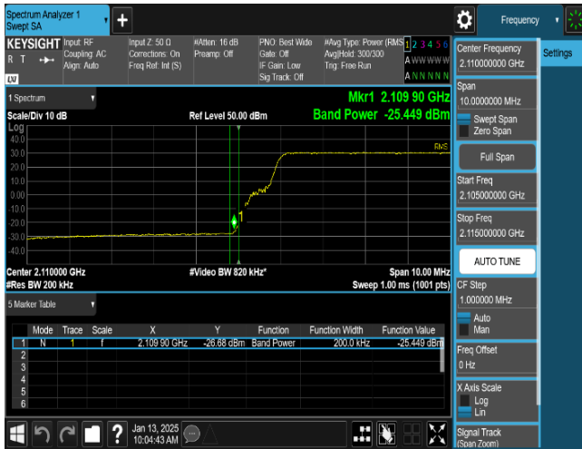
Plot 8-51. Band Edge Emission Summary Data Plot (LTE_B66_1C_20M_QPSK - Low Edge, Port 0)
