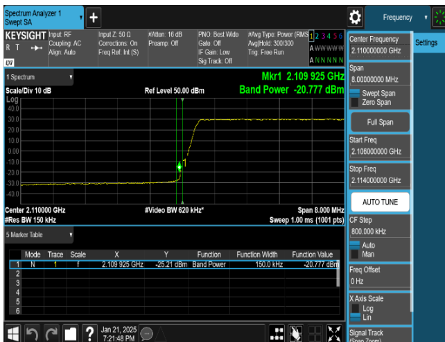
Plot 8-55. Band Edge Emission Summary Data Plot (NR_n66_1C_15M_256QAM - Low Edge, Port 3)
