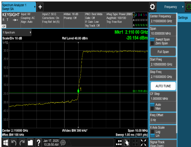
Plot 8-53. Band Edge Emission Summary Data Plot (NR_n66_1C_10M_16QAM - Low Edge, Port 2)
