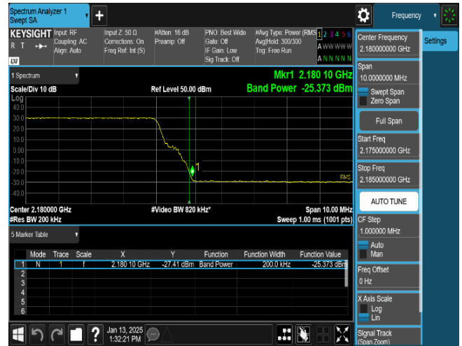
Plot 8-52. Band Edge Emission Summary Data Plot (LTE_B66_1C_20M_QPSK - High Edge, Port 1)
