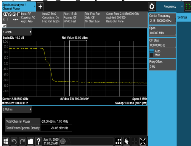
Plot 8-80. Conducted Spurious Emission Plot 2.181 MHz to 2.182 GHz
