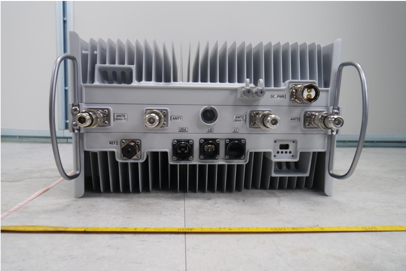
Bottom view
