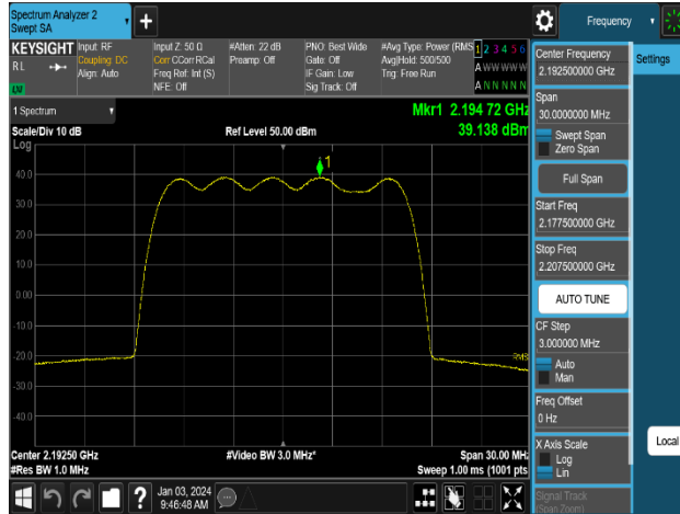
Plot 8-9. Power Spectral Density Plot (n66_1C_15M_16QAM - High Channel, Port 0)
