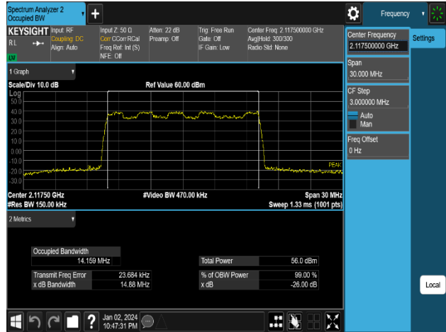
Plot 8-2. Occupied Bandwidth Plot (n66_1C_15M_16QAM - Low Channel, Port 2)
