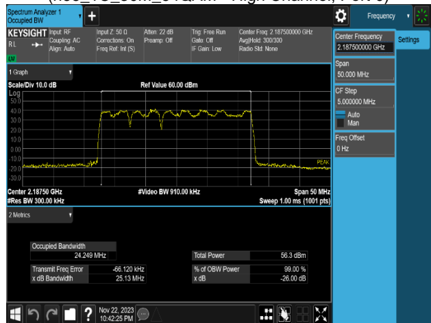
Plot 8-6. Occupied Bandwidth Plot (n66_3C_5M+5M+15M_16QAM - High Channel, Port 0)
