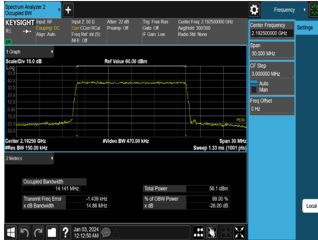
Plot 8-1. Occupied Bandwidth Plot (n66_1C_15M_QPSK - High Channel, Port 3)
