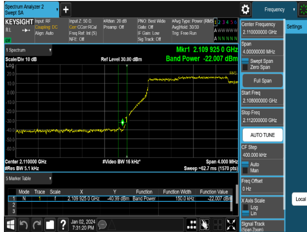
Plot 8-31. Band Edge Emission Plot (n66_1C_15M_16QAM - Low Channel, Port 0)
