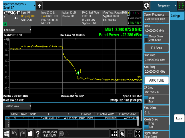
Plot 8-32. Band Edge Emission Plot (n66_1C_15M_16QAM - High Channel, Port 1)
