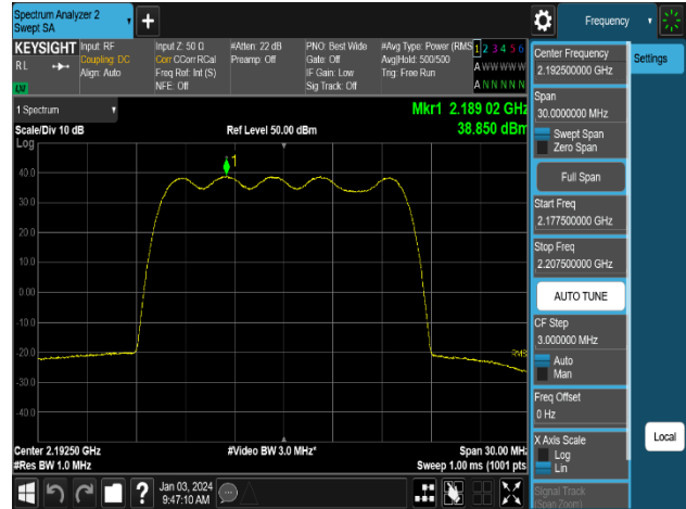
Plot 8-10. Power Spectral Density Plot (n66_1C_15M_16QAM - High Channel, Port 1)
