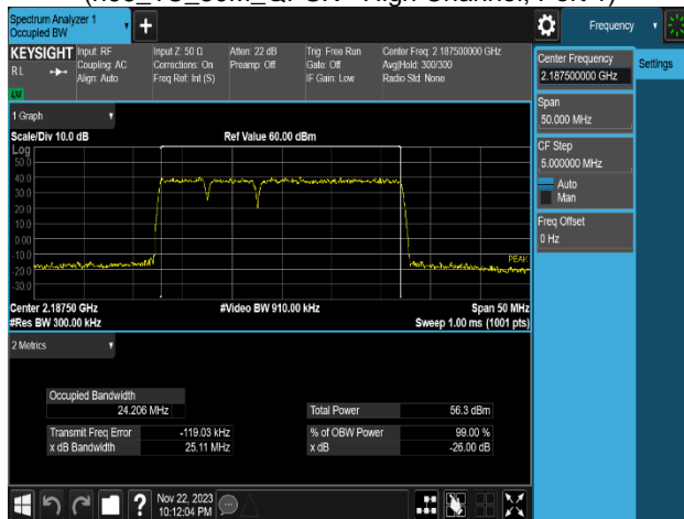
Plot 8-5. Occupied Bandwidth Plot (n66_3C_5M+5M+15M_QPSK - High Channel, Port 3)
