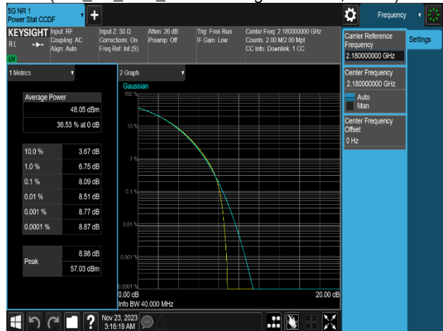
Plot 8-30. Peak To Average Power Ratio Plot (n66_3C_5M+5M+30M_QPSK - High Channel, Port 1)
