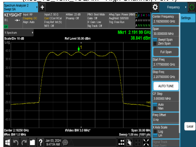
Plot 8-12. Power Spectral Density Plot (n66_1C_15M_16QAM - High Channel, Port 3)
