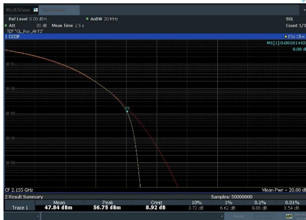
Plot 8-27. Peak To Average Power Ratio Plot (n66_1C_20M_QPSK - Mid Channel, Port 3)
