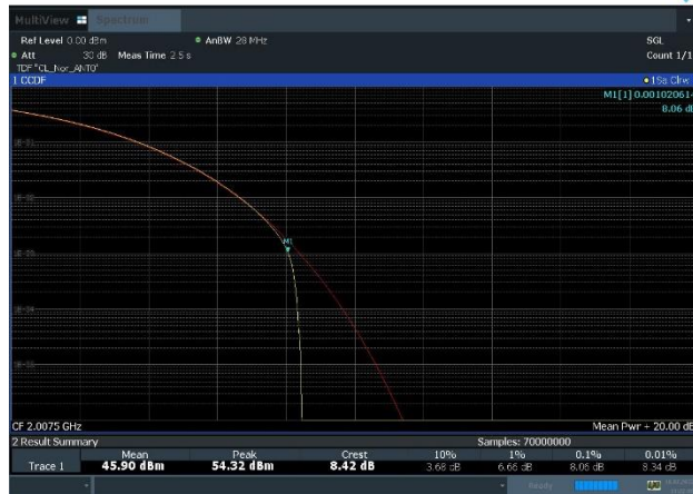
Plot 8-31. Peak To Average Power Ratio Plot (n70_1C_25M_QPSK-Mid Channel, Port 0)
