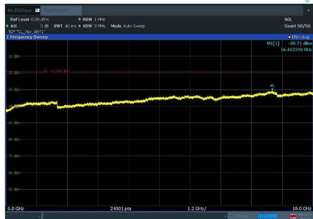
Plot 8-67. Conducted Spurious Emission Plot 6 GHz to 18 GHz (n66_2C_5M+20M_16QAM - Low Channel, Port 1)
