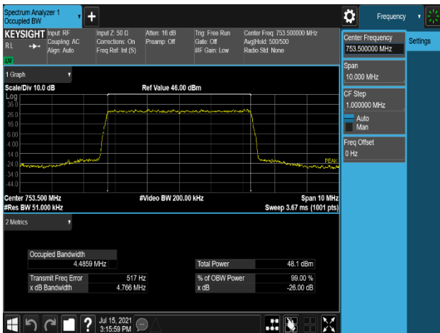
Plot 7-63. Occupied Bandwidth Plot (LTE_B13_5M_1C_64QAM - High Channel, Port 1)
