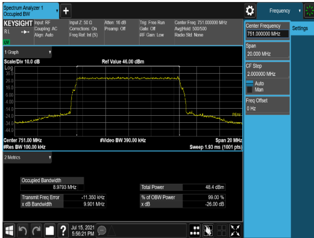
Plot 7-67. Occupied Bandwidth Plot (LTE_B13_10M_1C_64QAM - Port 0)
