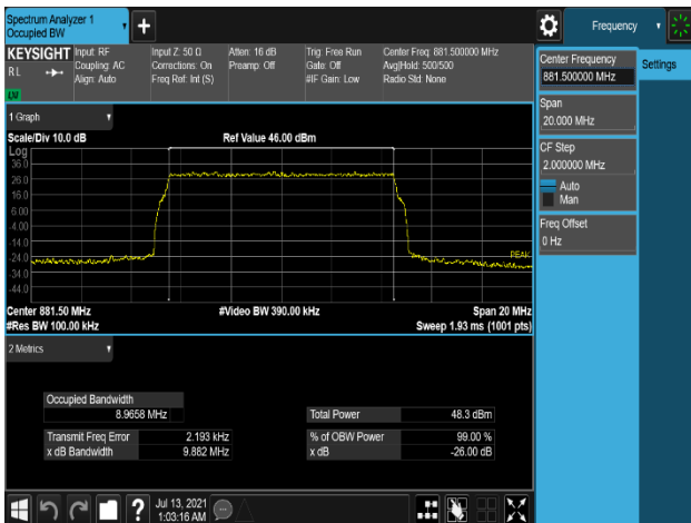
Plot 7-17. Occupied Bandwidth Plot (LTE_B5_10M_1C_QPSK - Mid Channel, Port 1)
