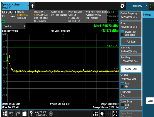
Plot 7-467. Conducted Spurious Emission Plot 895 MHz to 1 GHz (DSS_B5_10M_8:2)_1C_256QAM -- High Channel, Port 3)
