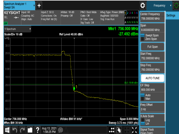
Plot 7-316. Band Edge Emission (756MHz to 757MHz) Plot (LTE_B13_5M+NB-lot(IB)_1C – Port 0)
