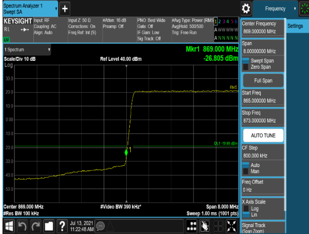
Plot 7-299. Band Edge Emission (868MHz to 869MHz) Plot (LTE_B5_5M+5M_2C_QPSK - Low Channel, Port 0)
