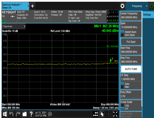
Plot 7-345. Conducted Spurious Emission Plot 858 MHz to 868 MHz (LTE_B5_5M_1C_64QAM - High Channel, Port 0)
