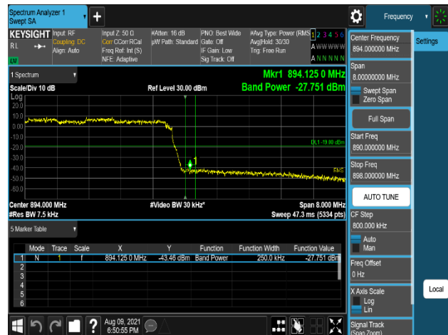
Plot 7-336. Band Edge Emission (894MHz to 895MHz) Integration method Plot (DSS_B5_10M+10M+5M_3C_16QAM - High Channel, Port 2)
