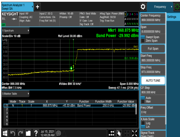
Plot 7-303. Band Edge Emission (868MHz to 869MHz) Integration method Plot (B2 5M+10M+10M 3C QPSK - Low Channel, Port 0)
