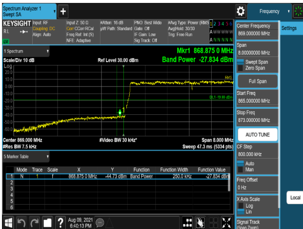
Plot 7-335. Band Edge Emission (868MHz to 869MHz) Integration method Plot (DSS_B5_10M+10M+5M_3C_16QAM - Low Channel, Port 2)
