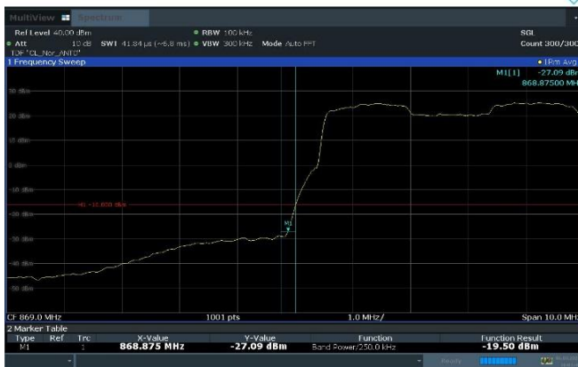
Plot 8-13. Band Edge Emission Summary Data Plot (n5_1C_25M_16QAM - Low Edge_2T, Port 0)
