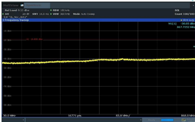
Plot 8-19. Conducted Spurious Emission Plot 30 MHz to 868 MHz (n5_1C_25M_4T_QPSK - Mid Channel, Port 2)
