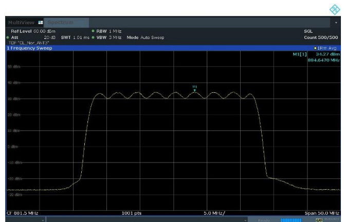
Plot 8-10. Equivalent Radiated Power Plot (n5_1C_25M_4T_16QAM - Mid Channel, Port 3)
