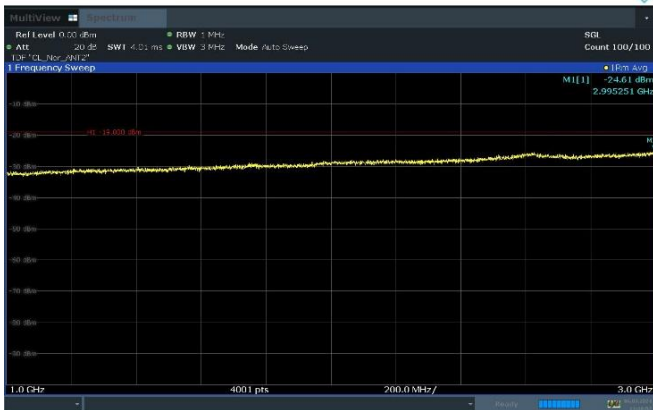
Plot 8-21. Conducted Spurious Emission Plot 1 GHz to 3 GHz (n5_1C_25M_4T_QPSK - Mid Channel, Port 2)
