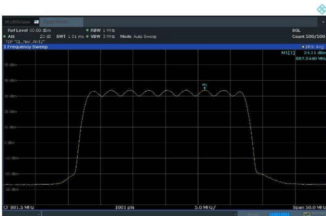
Plot 8-9. Equivalent Radiated Power Plot (n5_1C_25M_4T_16QAM - Mid Channel, Port 2)
