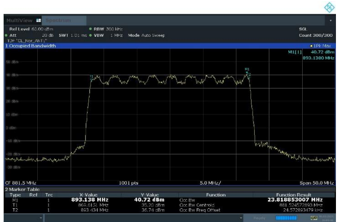
Plot 8-2. Occupied Bandwidth Plot (n5_1C_25M_2T_16QAM - Mid Channel, Port 1)
