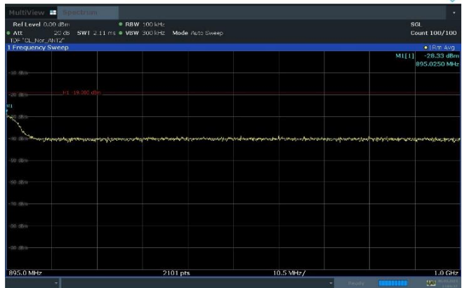
Plot 8-20. Conducted Spurious Emission Plot 895 MHz to 1 GHz (n5_1C_25M_4T_QPSK - Mid Channel, Port 2)
