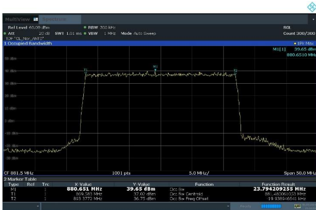
Plot 8-1. Occupied Bandwidth Plot (n5_1C_25M_2T_QPSK - Mid Channel, Port 0)
