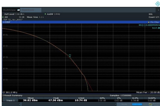
Plot 8-12. Peak To Average Power Ratio Plot (n5_1C_25M_4T_16QAM - Mid Channel, Port 2)
