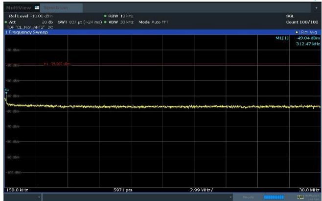
Plot 8-18. Conducted Spurious Emission Plot 150 kHz to 30 MHz (n5_1C_25M_4T_QPSK - Mid Channel, Port 2)
