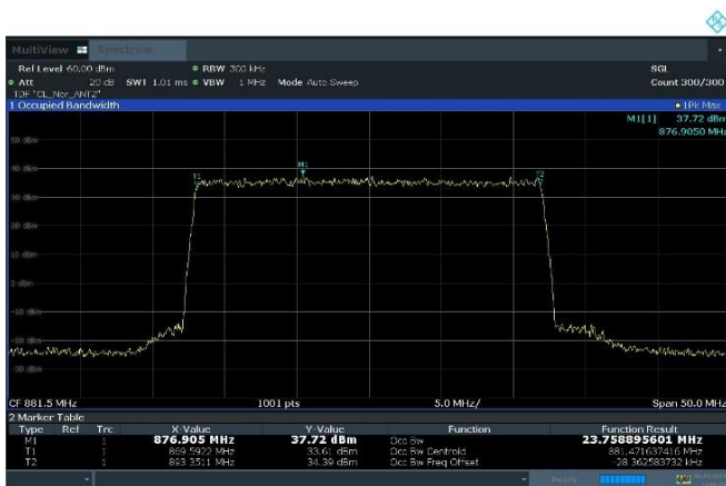
Plot 8-3. Occupied Bandwidth Plot (n5_1C_25M_4T_QPSK - Mid Channel, Port 2)
