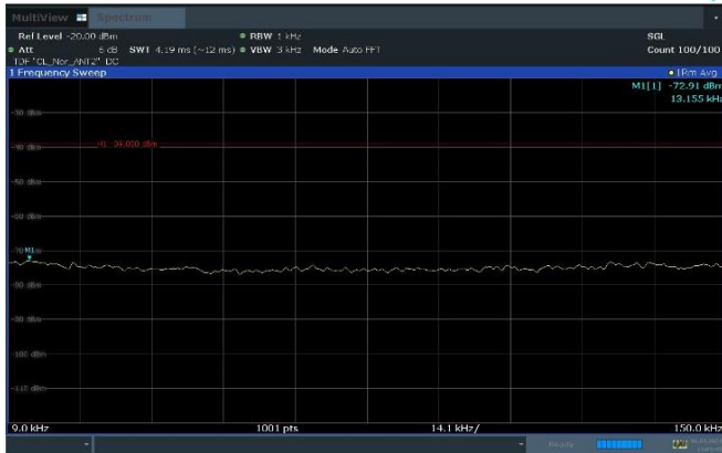
Plot 8-17. Conducted Spurious Emission Plot 9 kHz to 150 kHz (n5_1C_25M_4T_QPSK - Mid Channel, Port 2)
