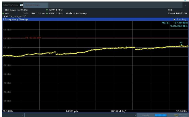
Plot 8-22. Conducted Spurious Emission Plot 3 GHz to 10 GHz (n5_1C_25M_4T_QPSK - Mid Channel, Port 2)
