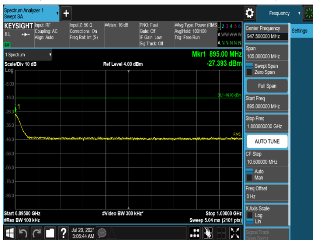
Plot 7-673. Conducted Spurious Emission Plot 895 MHz to 1 GHz (B5_10M_2T_1C_16QAM - High Channel, Port 1)
