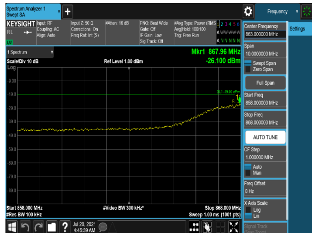
Plot 7-690. Conducted Spurious Emission Plot 858 MHz to 868 MHz (B5_5M+5M_2C_2T_256QAM- Low Channel, Port 0)
