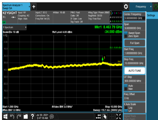
Plot 7-668. Conducted Spurious Emission Plot 1 GHz to 10 GHz (B5_5M_1C_2T_QPSK - High Channel, Port 1)
