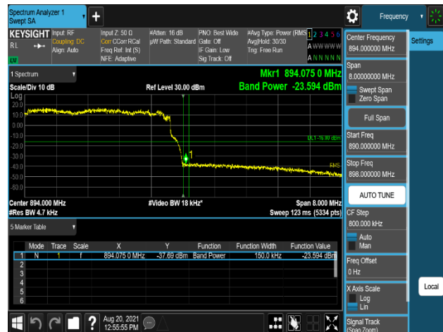
Plot 7-650. Band Edge Emission (894MHz to 895MHz) Plot Integration method Plot (B5_10M(DSS)+5M_2C_64QAM - High Channel, Port 0)
