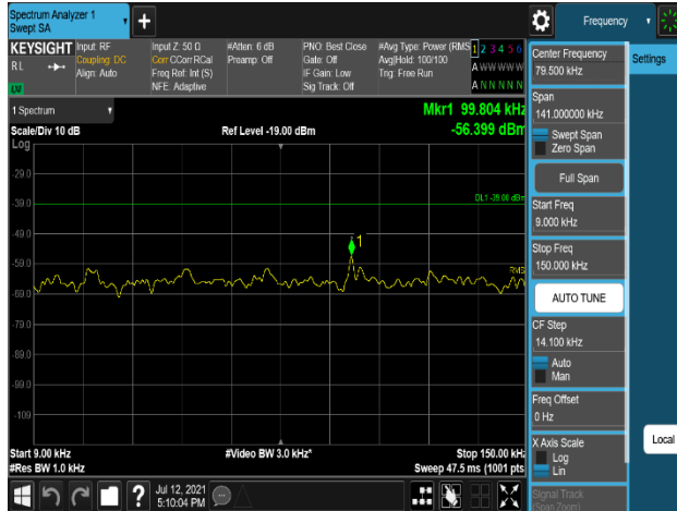
Plot 7-675. Conducted Spurious Emission Plot 9 kHz to 150 kHz (B5_5M_1C_QPSK - Low Channel, Port 1)
