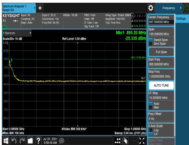
Plot 7-691. Conducted Spurious Emission Plot 895 MHz to 1 GHz (B5_5M+5M_2C_2T_QPSK - High Channel, Port 0)
