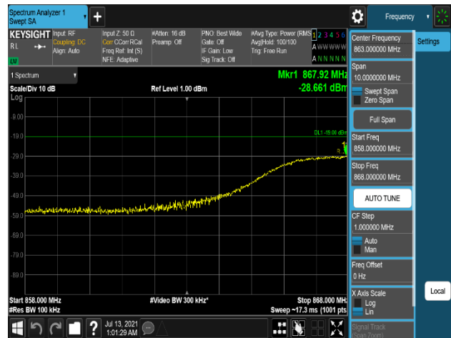
Plot 7-684. Conducted Spurious Emission Plot 858 MHz to 868 MHz (B5_10M_1C_256QAM - Low Channel, Port 2)
