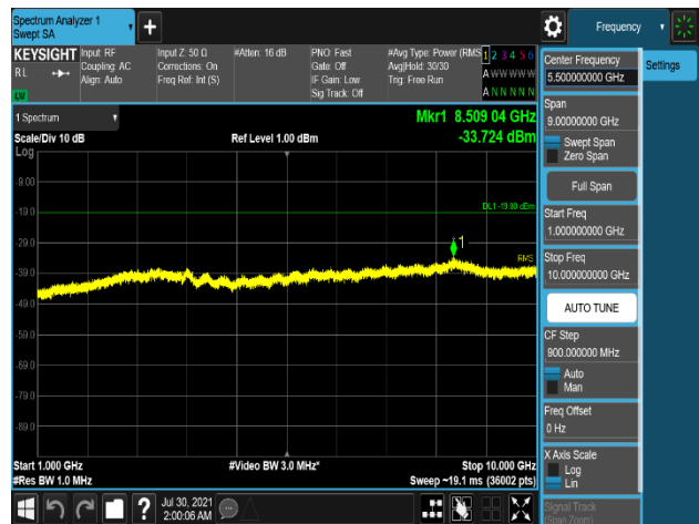
Plot 7-680. Conducted Spurious Emission Plot 1 GHz to 10 GHz (B5_5M_1C_2T_64QAM - Low Channel, Port 1)
