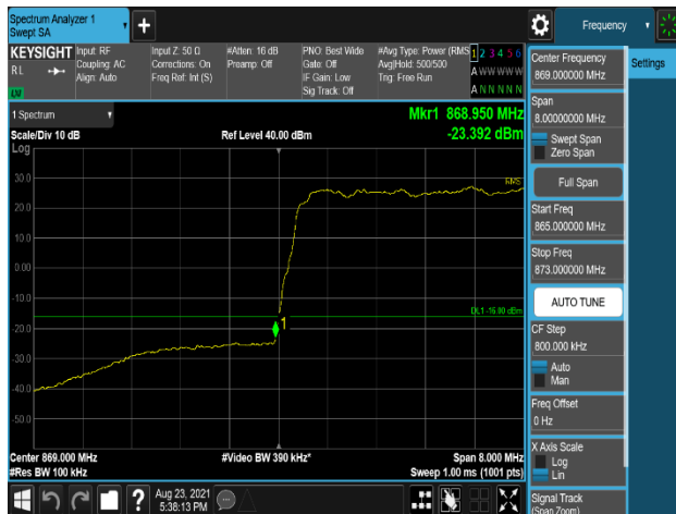
Plot 7-661. Band Edge Emission (868MHz to 869MHz) Plot (B5_10M(DSS)+10M_2C_256QAM - Low Channel, Port 0)
