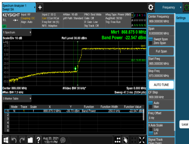
Plot 7-653. Band Edge Emission (868MHz to 869MHz) Integration method Plot (B5_10M(DSS)+10M+5M_3C_QPSK - Low Channel, Port 0)
