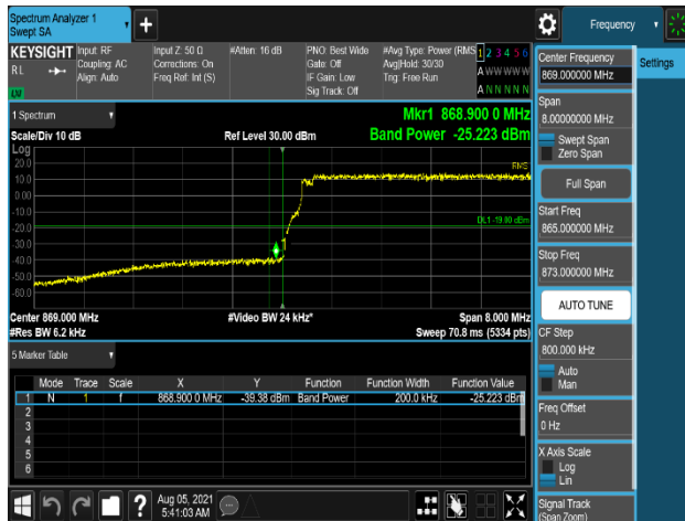
Plot 7-645. Band Edge Emission (868MHz to 869MHz) Plot Integration method Plot (B5_10M(DSS)+10M_2C_QPSK - Low Channel, Port 3)
