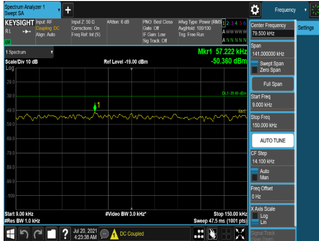
Plot 7-687. Conducted Spurious Emission Plot 9 kHz to 150 kHz (B5_5M+5M_2C_2T_16QAM - Low Channel, Port 0)
