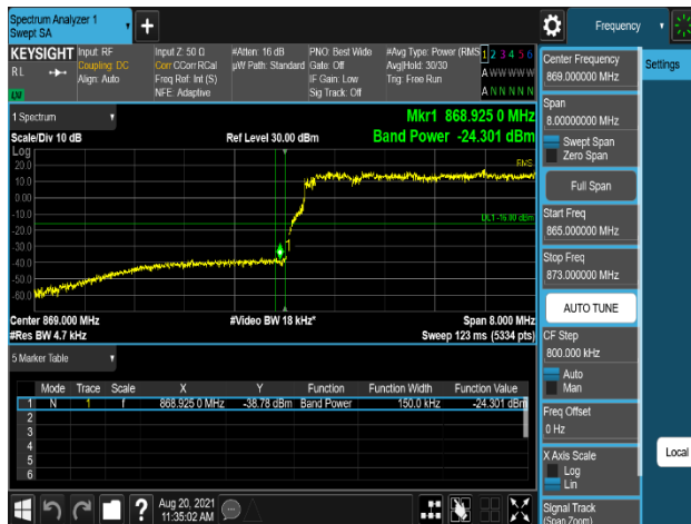
Plot 7-649. Band Edge Emission (868MHz to 869MHz) Plot Integration method Plot (B5_10M(DSS)+5M_2C_256QAM - Low Channel, Port 0)
