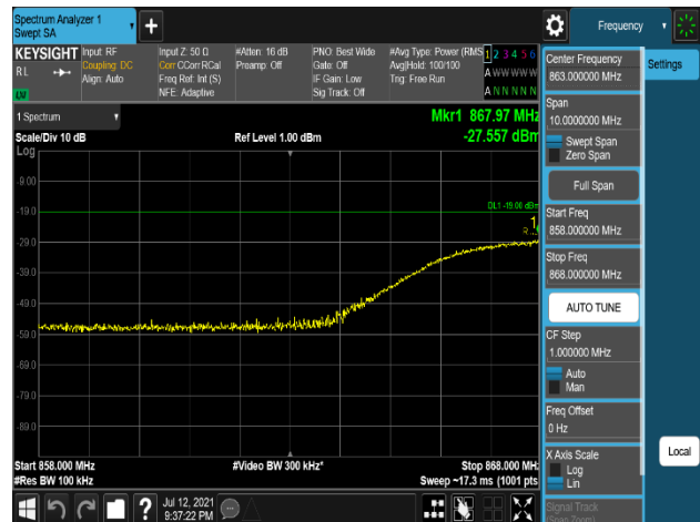
Plot 7-678. Conducted Spurious Emission Plot 858 MHz to 868 MHz (B5_5M_1C_64QAM - Low Channel, Port 2)
