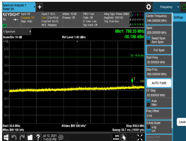
Plot 7-677. Conducted Spurious Emission Plot 30 MHz to 858 MHz (B5_5M_1C_QPSK - High Channel, Port 1)
