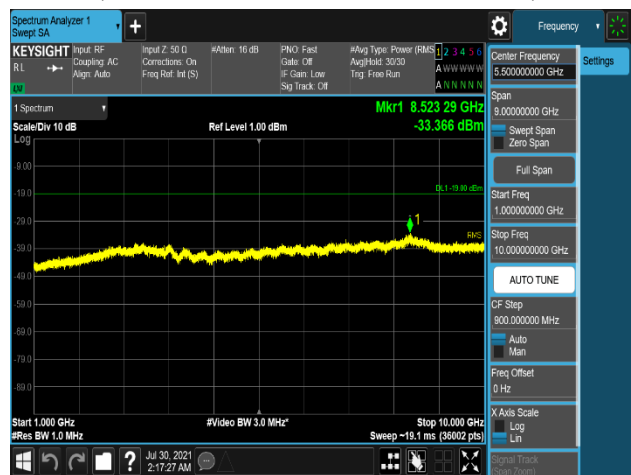
Plot 7-686. Conducted Spurious Emission Plot 1 GHz to 10 GHz (B5_10M_1C_QPSK - Low Channel, Port 1)
