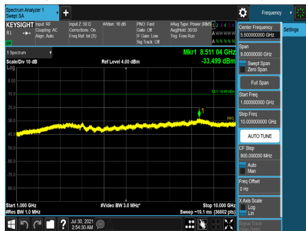
Plot 7-674. Conducted Spurious Emission Plot 1 GHz to 10 GHz (B5_10M_1C_2T_256QAM - Low Channel, Port 1)
