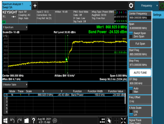
Plot 7-643. Band Edge Emission (868MHz to 869MHz) Plot Integration method Plot (B5_10M(DSS)+5M_2C_16QAM - Low Channel, Port 2)
