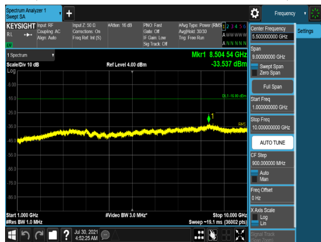
Plot 7-692. Conducted Spurious Emission Plot 1 GHz to 10 GHz (B5_5M+5M_2C_2T_256QAM - High Channel, Port 1)
