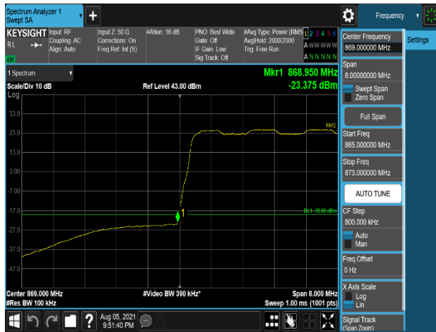
Plot 7-657. Band Edge Emission (868MHz to 869MHz) Plot (B5_10M(DSS)+10M_2C_16QAM - Low Channel, Port 3)
