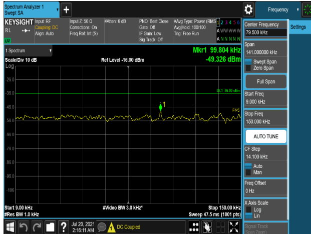
Plot 7-669. Conducted Spurious Emission Plot 9 kHz to 150 kHz (B5_10M_1C_2T_16QAM - Middle Channel, Port 1)
