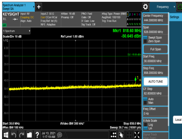
Plot 7-683. Conducted Spurious Emission Plot 30 MHz to 858 MHz (B5_10M_1C_QPSK - Middle Channel, Port 1)
