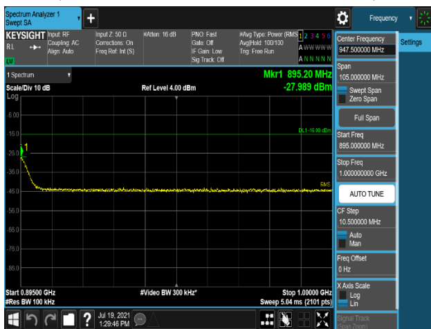
Plot 7-667. Conducted Spurious Emission Plot 895 MHz to 1 GHz (B5_5M_1C_2T_64QAM - High Channel, Port 1)
