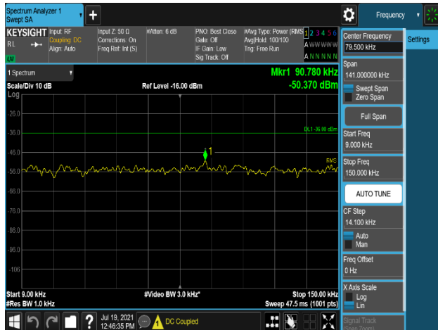
Plot 7-663. Conducted Spurious Emission Plot 9 kHz to 150 kHz (B5_5M_1C_2T_256QAM - Middle Channel, Port 0)
