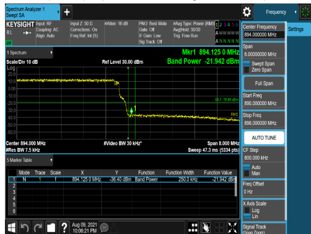
Plot 7-648. Band Edge Emission (894MHz to 895MHz) Integration method Plot (B5_10M(DSS)+10M+5M_3C_QPSK - High Channel, Port 3)
