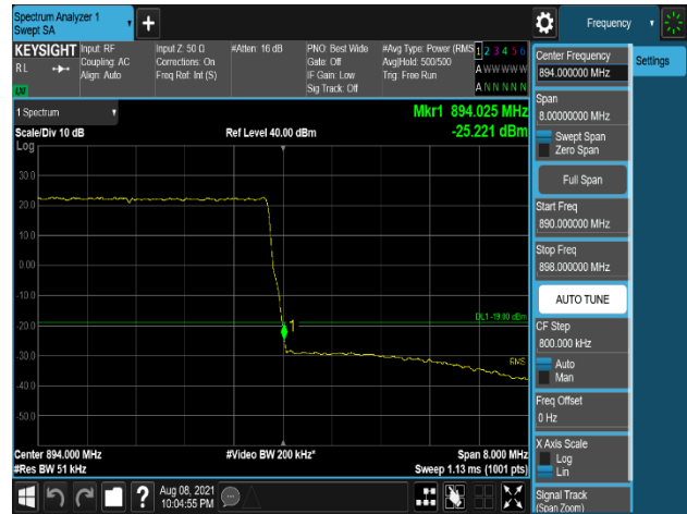
Plot 7-656. Band Edge Emission (894MHz to 895MHz) Plot (B5_10M(DSS)+5M_2C_256QAM - High Channel, Port 3)
