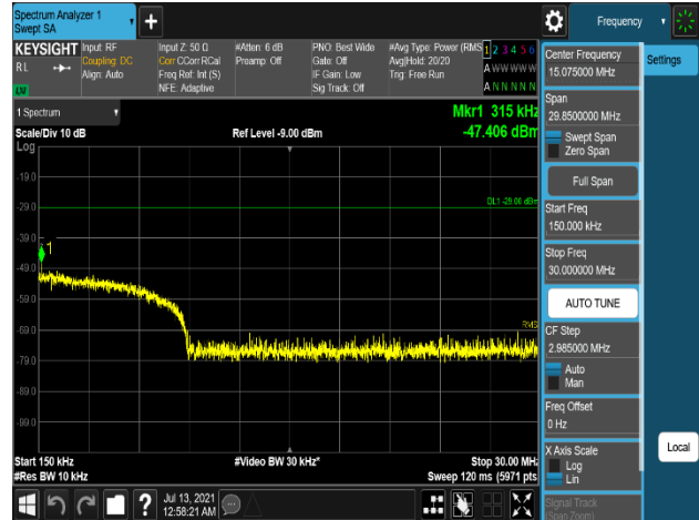
Plot 7-682. Conducted Spurious Emission Plot 150 kHz to 30 MHz (B5_10M_1C_256QAM - Low Channel, Port 1)
