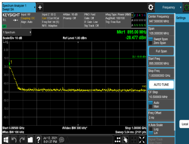
Plot 7-679. Conducted Spurious Emission Plot 895 MHz to 1 GHz (B5_5M_1C_16QAM - High Channel, Port 3)
