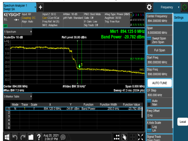
Plot 7-654. Band Edge Emission (894MHz to 895MHz) Integration method Plot (B5_10M(DSS)+10M+5M_3C_16QAM - High Channel, Port 0)
