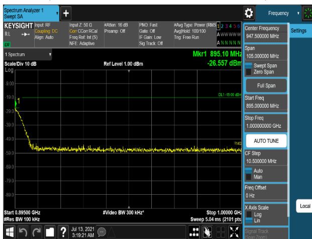
Plot 7-685. Conducted Spurious Emission Plot 895 MHz to 1 GHz (B5_10M_1C_256QAM - High Channel, Port 3)
