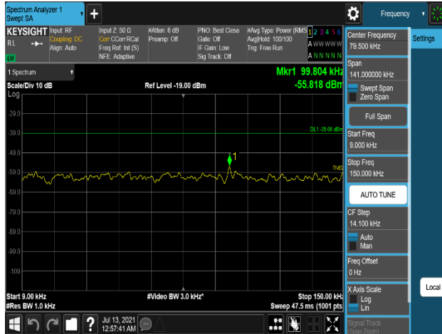
Plot 7-681. Conducted Spurious Emission Plot 9 kHz to 150 kHz (B5_10M_1C_256QAM - Low Channel, Port 3)
