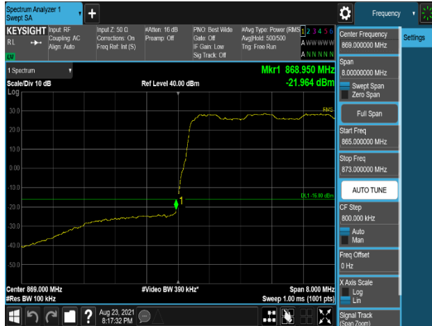
Plot 7-659. Band Edge Emission (868MHz to 869MHz) Plot (B5_10M(DSS)+5M_2C_16QAM - Low Channel, Port 0)
