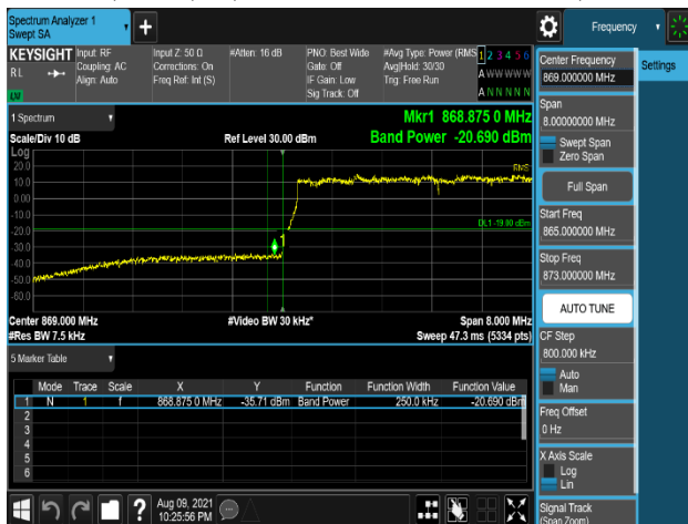
Plot 7-647. Band Edge Emission (868MHz to 869MHz) Integration method Plot (B5_10M(DSS)+10M+5M_3C_16QAM - Low Channel, Port 2)
