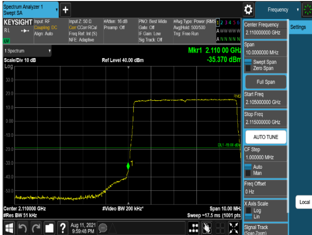
Plot 7-991. Band Edge Emission (2109MHz to 2110MHz) Plot (B66_5M+5M+5M+5M_4C_64QAM - Low Channel, Port 2)
