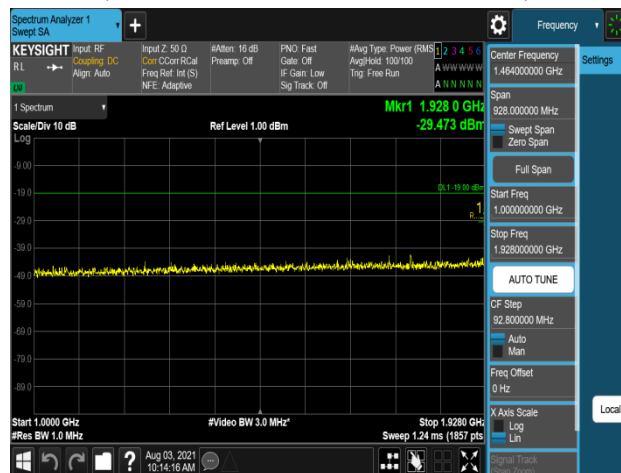
Plot 7-1018. Conducted Spurious Emission Plot 1 GHz to 1.928 GHz (B2_15M_1C_QPSK - Low Channel, Port 0)
