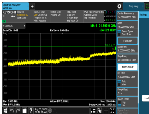
Plot 7-1020. Conducted Spurious Emission Plot 6 GHz to 22 GHz (B2_15M_1C_QPSK - Low Channel, Port 1)
