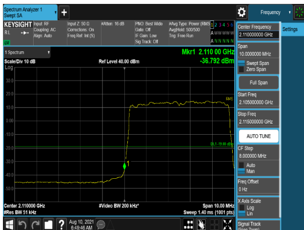
Plot 7-983. Band Edge Emission (2109MHz to 2110MHz) Plot (B66_5M+5M+20M_3C_16QAM - Low Channel, Port 0)
