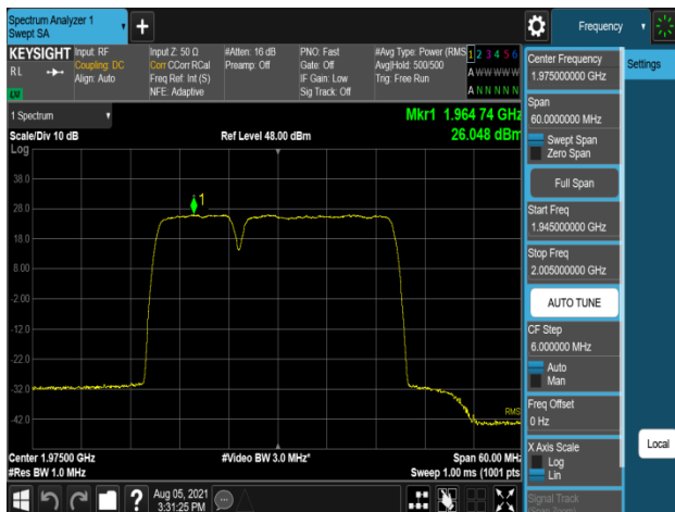
Plot 7-611. Peak Power Spectral Density Plot (B2_10M+20M_2C_16QAM – High Channel, Port 2)
