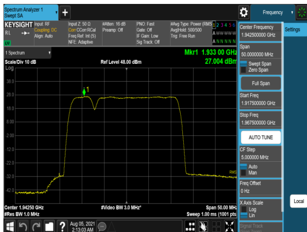
Plot 7-591. Peak Power Spectral Density Plot (B2_5M+20M_2C_16QAM - Low Channel, Port 2)
