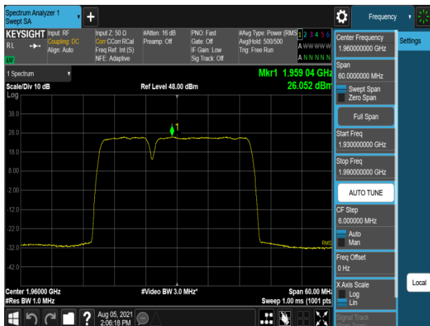
Plot 7-605. Peak Power Spectral Density Plot (B2_10M+20M_2C_16QAM - Mid Channel, Port 0)
