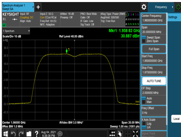
Plot 7-581. Peak Power Spectral Density Plot (B2_5M+5M_2C_16QAM - Mid Channel, Port 0)
