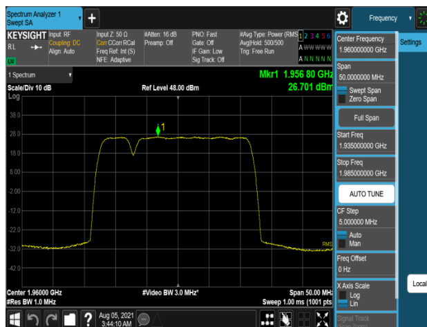
Plot 7-594. Peak Power Spectral Density Plot (B2_5M+20M_2C_16QAM - Mid Channel, Port 1)
