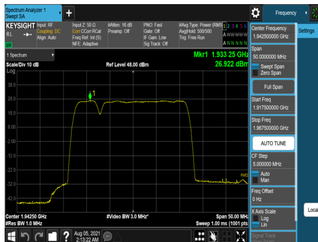
Plot 7-592. Peak Power Spectral Density Plot (B2_5M+20M_2C_16QAM - Low Channel, Port 3)
