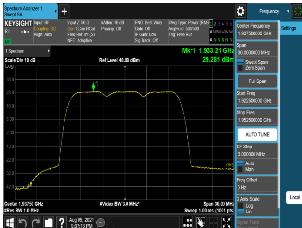
Plot 7-615. Peak Power Spectral Density Plot (B2_5M+5M+5M_3C_16QAM - Low Channel, Port 2)
