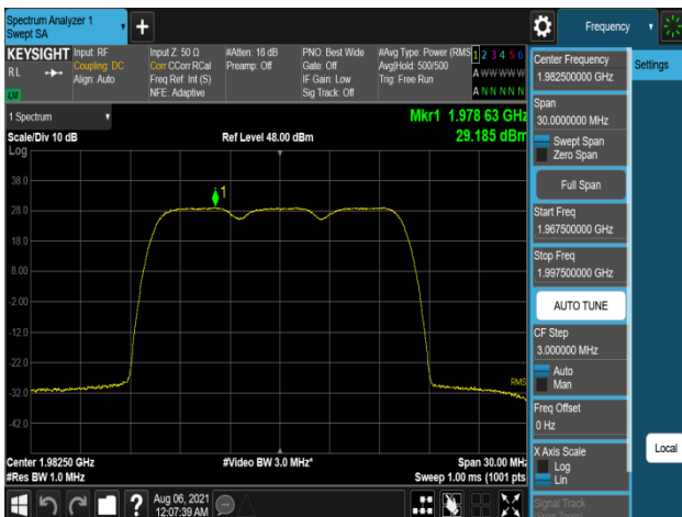
Plot 7-623. Peak Power Spectral Density Plot (B2_5M+5M+5M_3C_16QAM - High Channel, Port 2)
