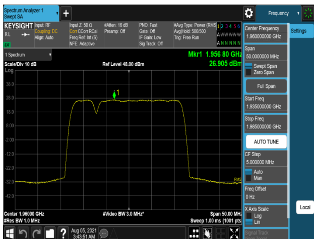
Plot 7-593. Peak Power Spectral Density Plot (B2_5M+20M_2C_16QAM - Mid Channel, Port 0)
