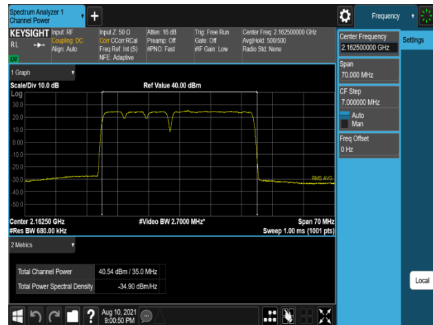
Plot 7-514. Conducted Average Output Power Plot (B66_5M+5M+5M+20M_4C_QPSK - High Channel, Port 1)
