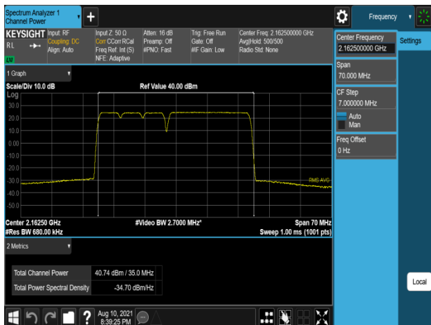
Plot 7-515. Conducted Average Output Power Plot (B66_5M+5M+5M+20M_4C_QPSK - High Channel, Port 2)
