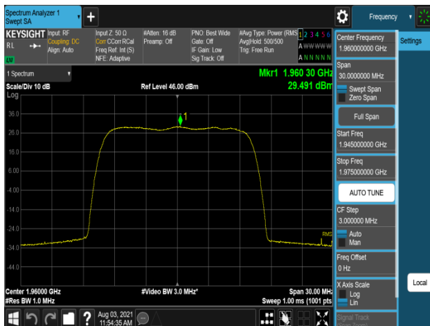
Plot 7-557. Peak Power Spectral Density Plot (B2_15M_1C_16QAM - Mid Channel, Port 0)
