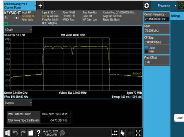
Plot 7-512. Conducted Average Output Power Plot (B66_5M+5M+5M+20M_4C_16QAM - Mid Channel, Port 3)
