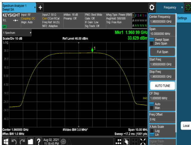
Plot 7-533. Peak Power Spectral Density Plot (B2_5M_1C_16QAM - Mid Channel, Port 0)
