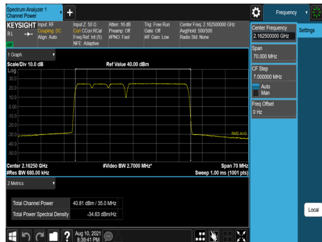
Plot 7-516. Conducted Average Output Power Plot (B66_5M+5M+5M+20M_4C_QPSK - High Channel, Port 3)
