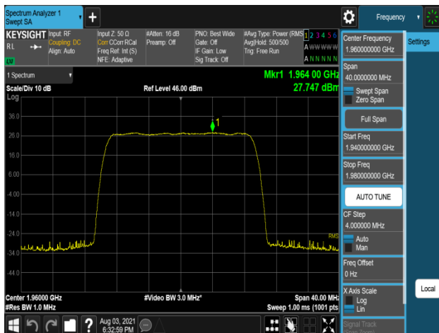
Plot 7-569. Peak Power Spectral Density Plot (B2_20M_1C_16QAM - Mid Channel, Port 0)
