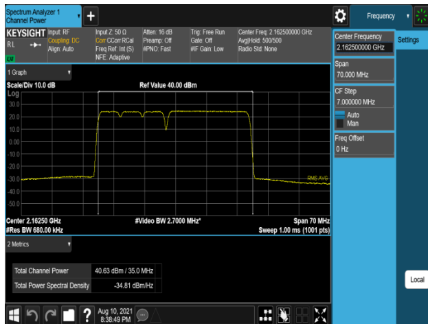
Plot 7-513. Conducted Average Output Power Plot (B66_5M+5M+5M+20M_4C_QPSK - High Channel, Port 0)
