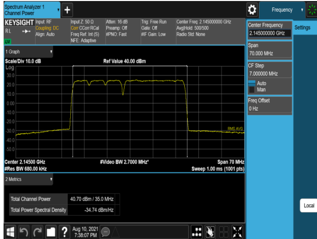
Plot 7-511. Conducted Average Output Power Plot (B66_5M+5M+5M+20M_4C_16QAM - Mid Channel, Port 2)
