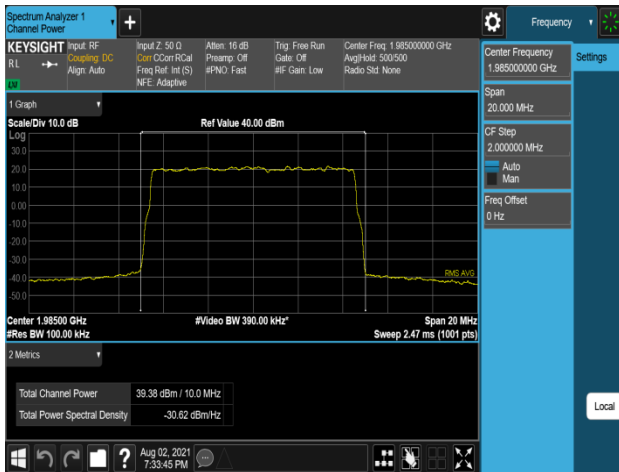
Plot 7-285. Conducted Average Output Power Plot (B2_10M_1C_16QAM – High Channel, Port 0)
