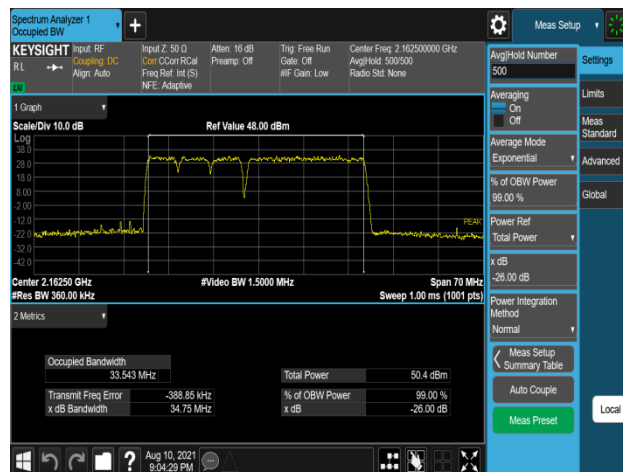
Plot 7-250. Occupied Bandwidth Plot (B66_5M+5M+5M+20M_4C_16QAM - High Channel, Port 2)
