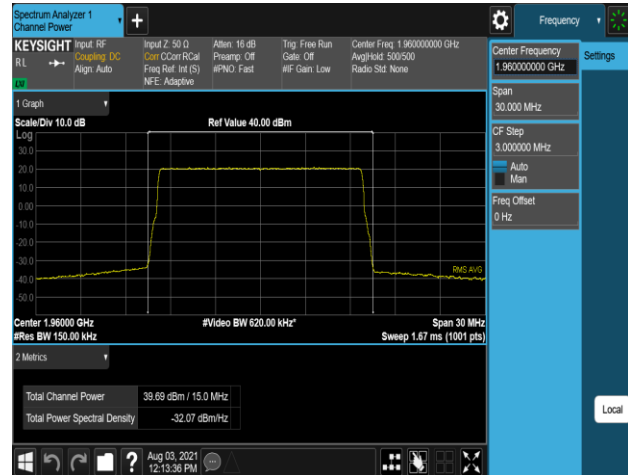
Plot 7-296. Conducted Average Output Power Plot (B2_15M_1C_64QAM - Mid Channel, Port 3)
