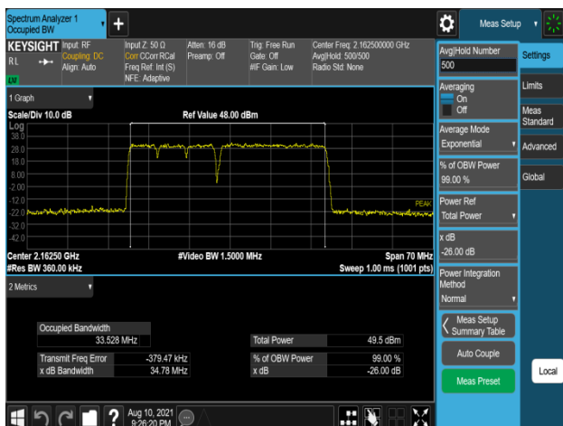
Plot 7-251. Occupied Bandwidth Plot (B66_5M+5M+5M+20M_4C_64QAM - High Channel, Port 2)
