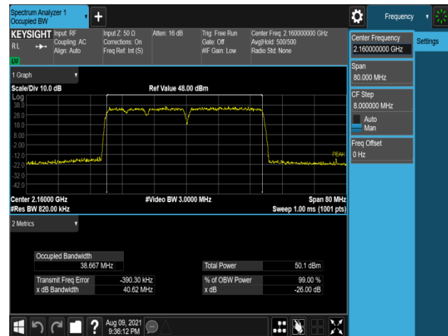
Plot 7-262. Occupied Bandwidth Plot (B66_5M+5M+10M+20M_4C_16QAM - High Channel, Port 1)
