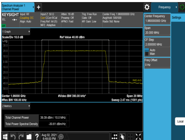
Plot 7-281. Conducted Average Output Power Plot (B2_10M_1C_256QAM - Mid Channel, Port 0)
