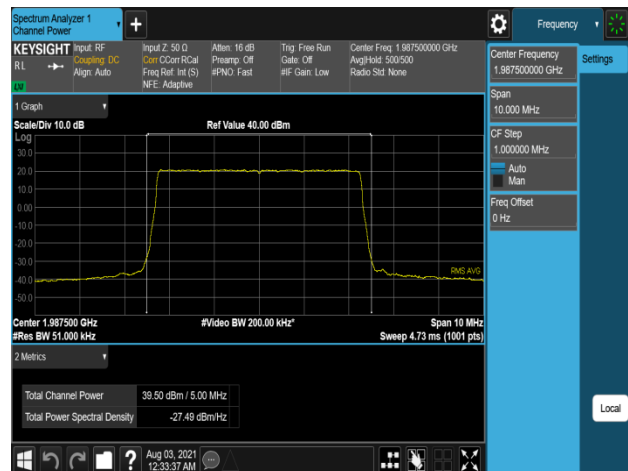
Plot 7-276. Conducted Average Output Power Plot (B2_5M_1C_256QAM - High Channel, Port 3)
