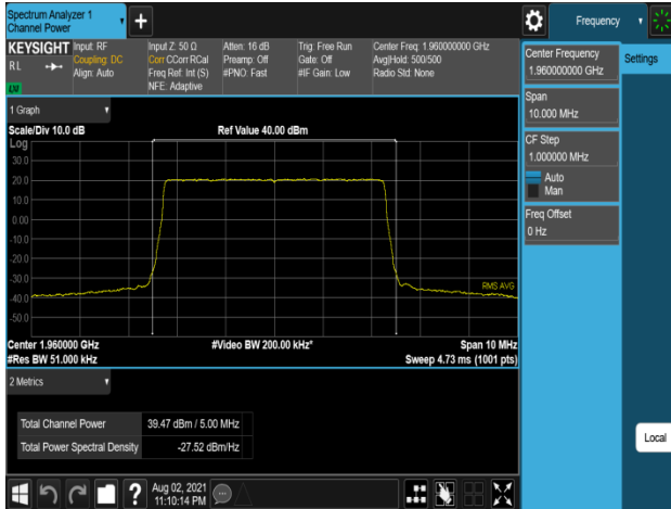
Plot 7-271. Conducted Average Output Power Plot (B2_5M_1C_QPSK - Mid Channel, Port 2)
