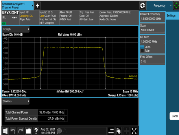
Plot 7-265. Conducted Average Output Power Plot (B2_5M_1C_64QAM - Low Channel, Port 0)
