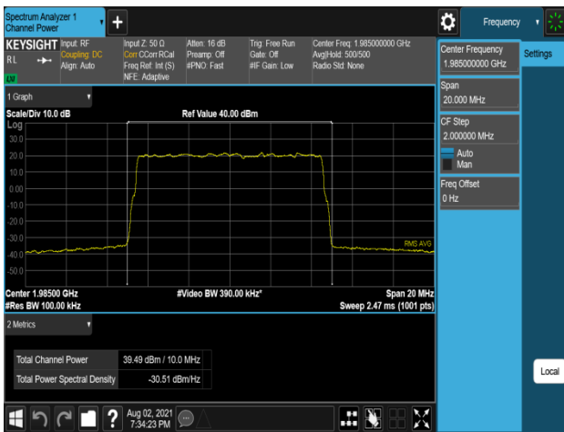
Plot 7-287. Conducted Average Output Power Plot (B2_10M_1C_16QAM – High Channel, Port 2)
