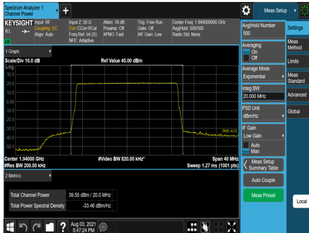
Plot 7-301. Conducted Average Output Power Plot (B2_20M_1C_256QAM - Low Channel, Port 0)
