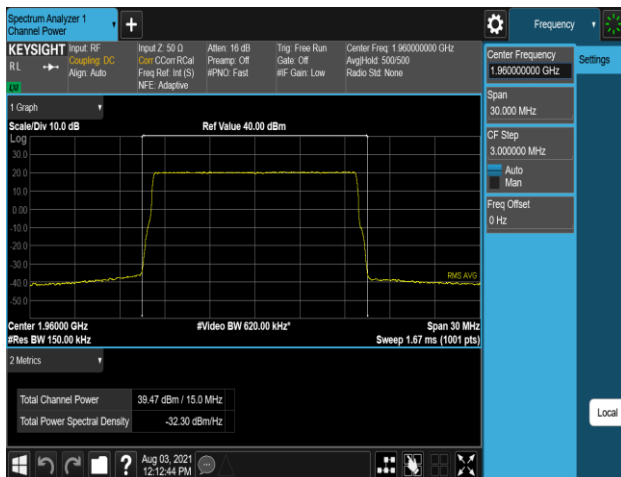
Plot 7-293. Conducted Average Output Power Plot (B2_15M_1C_64QAM - Mid Channel, Port 0)
