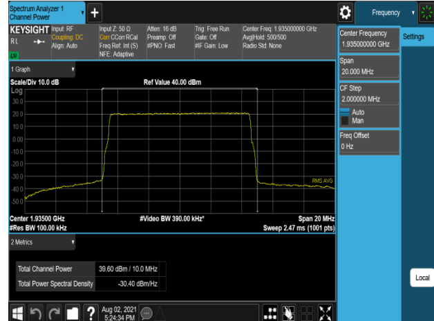
Plot 7-280. Conducted Average Output Power Plot (B2_10M_1C_256QAM - Low Channel, Port 3)
