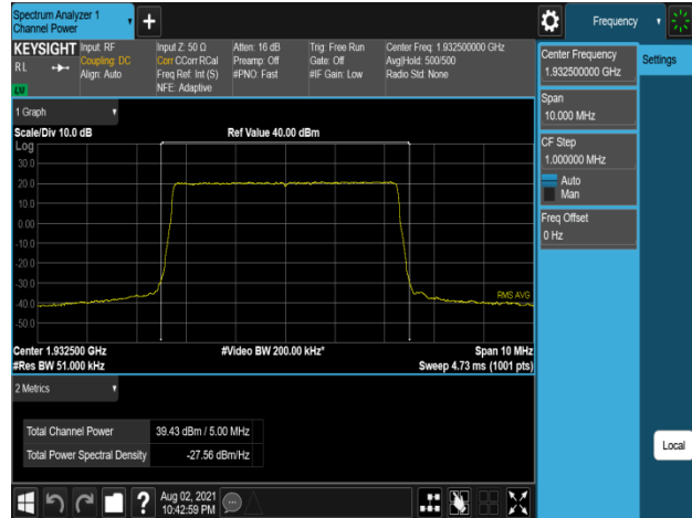
Plot 7-266. Conducted Average Output Power Plot (B2_5M_1C_64QAM - Low Channel, Port 1)
