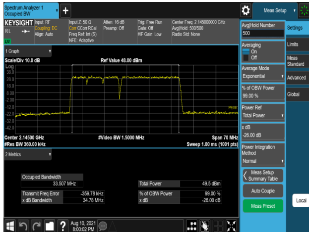
Plot 7-247. Occupied Bandwidth Plot (B66_5M+5M+5M+20M_4C_64QAM - Mid Channel, Port 0)
