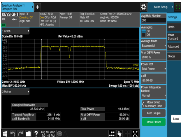
Plot 7-245. Occupied Bandwidth Plot (B66_5M+5M+5M+20M_4C_QPSK - Mid Channel, Port 0)
