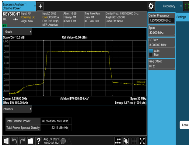
Plot 7-289. Conducted Average Output Power Plot (B2_15M_1C_QPSK - Low Channel, Port 0)
