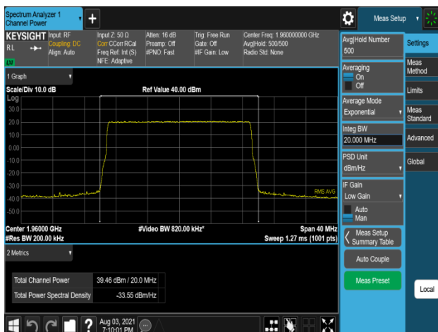
Plot 7-305. Conducted Average Output Power Plot (B2_20M_1C_256QAM - Mid Channel, Port 0)
