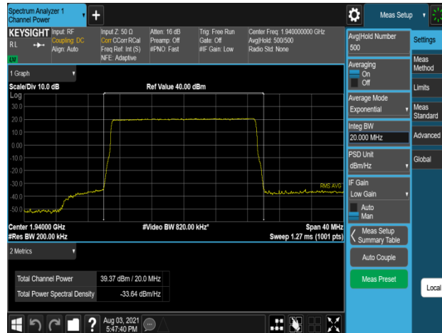
Plot 7-302. Conducted Average Output Power Plot (B2_20M_1C_256QAM - Low Channel, Port 1)
