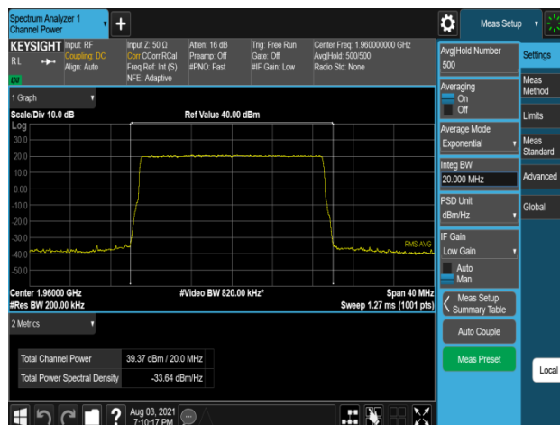
Plot 7-306. Conducted Average Output Power Plot (B2_20M_1C_256QAM - Mid Channel, Port 1)
