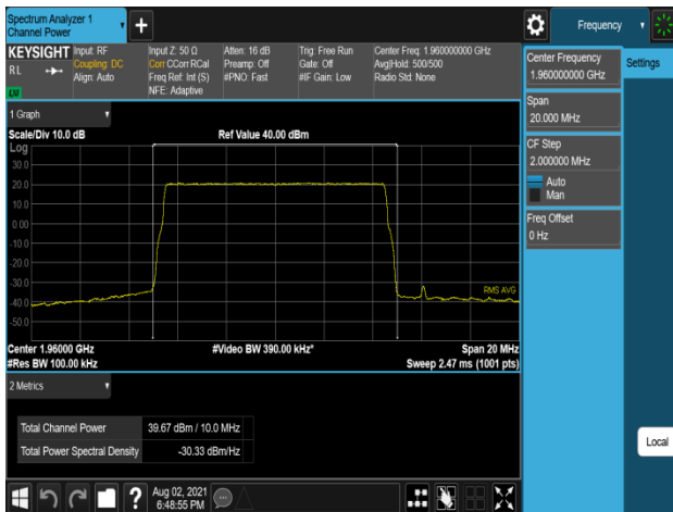
Plot 7-283. Conducted Average Output Power Plot (B2_10M_1C_256QAM – Mid Channel, Port 2)
