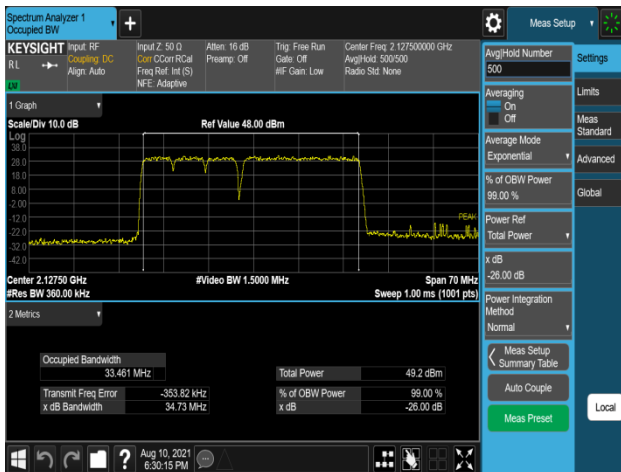
Plot 7-243. Occupied Bandwidth Plot (B66_5M+5M+5M+20M_4C_64QAM - Low Channel, Port 1)
