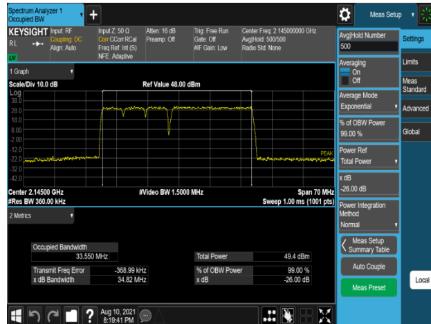
Plot 7-248. Occupied Bandwidth Plot (B66_5M+5M+5M+20M_4C_256QAM - Mid Channel, Port 2)
