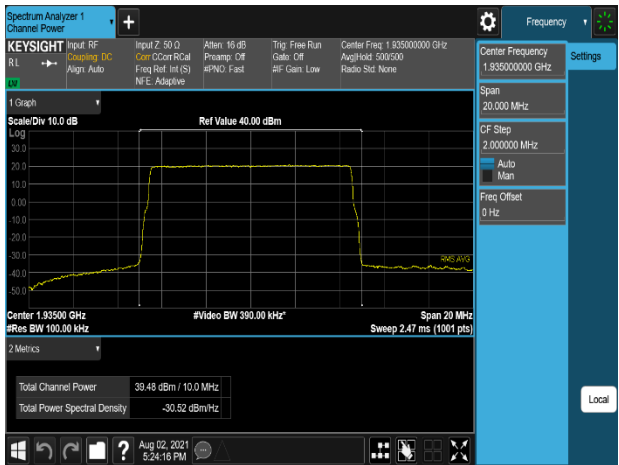
Plot 7-279. Conducted Average Output Power Plot (B2_10M_1C_256QAM - Low Channel, Port 2)
