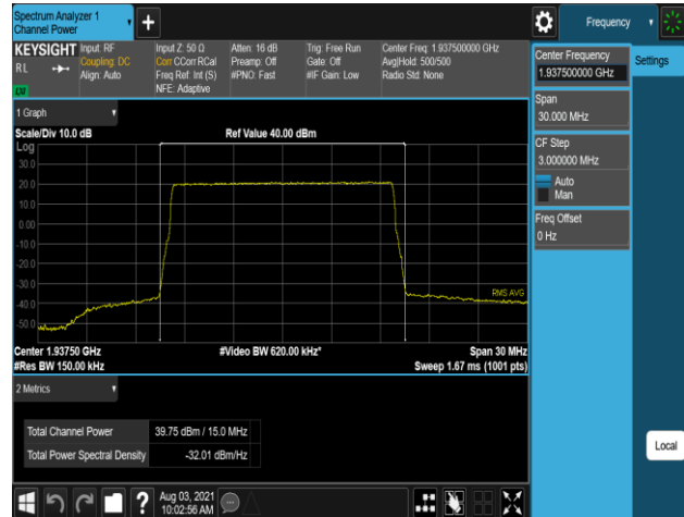
Plot 7-290. Conducted Average Output Power Plot (B2_15M_1C_QPSK - Low Channel, Port 1)
