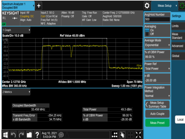
Plot 7-241. Occupied Bandwidth Plot (B66_5M+5M+5M+20M_4C_QPSK - Low Channel, Port 2)
