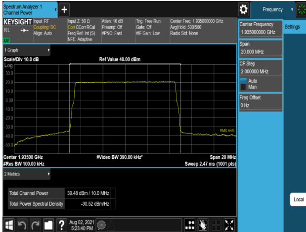
Plot 7-277. Conducted Average Output Power Plot (B2_10M_1C_256QAM - Low Channel, Port 0)
