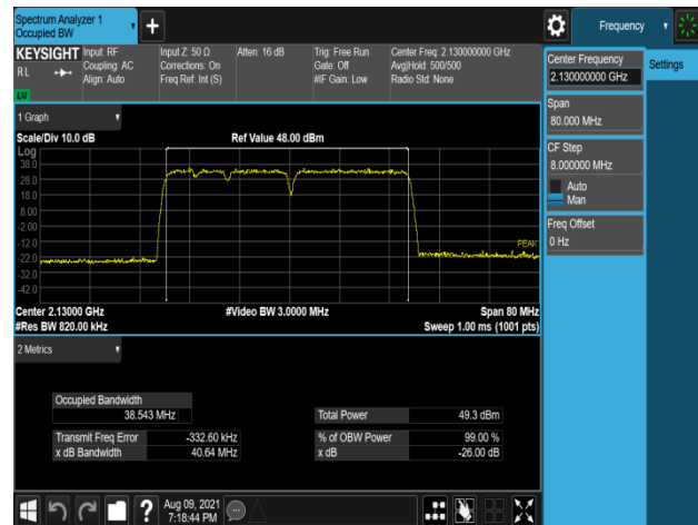
Plot 7-256. Occupied Bandwidth Plot (B66_5M+5M+10M+20M_4C_256QAM - Low Channel, Port 1)
