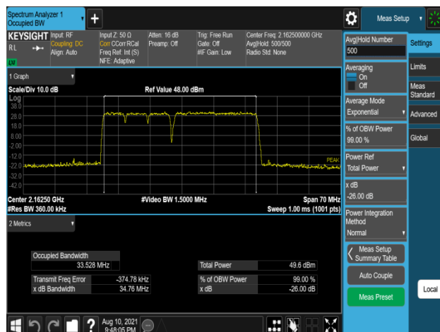
Plot 7-252. Occupied Bandwidth Plot (B66_5M+5M+5M+20M_4C_256QAM - High Channel, Port 2)
