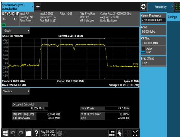
Plot 7-261. Occupied Bandwidth Plot (B66_5M+5M+10M+20M_4C_QPSK - High Channel, Port 0)
