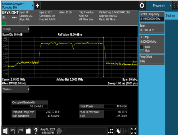
Plot 7-259. Occupied Bandwidth Plot (B66_5M+5M+10M+20M_4C_64QAM - Mid Channel, Port 0)
