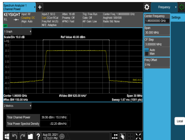
Plot 7-294. Conducted Average Output Power Plot (B2_15M_1C_64QAM - Mid Channel, Port 1)
