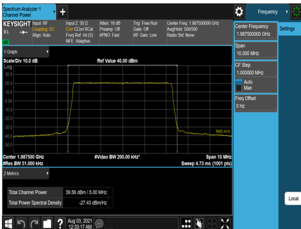
Plot 7-275. Conducted Average Output Power Plot (B2_5M_1C_256QAM - High Channel, Port 2)
