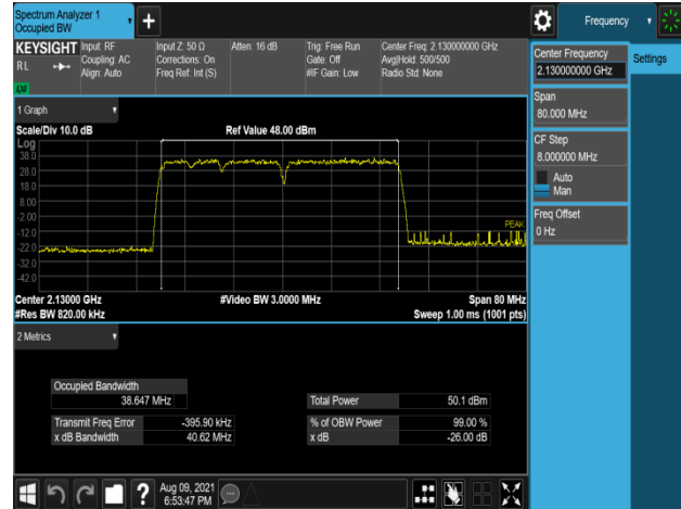
Plot 7-254. Occupied Bandwidth Plot (B66_5M+5M+10M+20M_4C_16QAM - Low Channel, Port 3)
