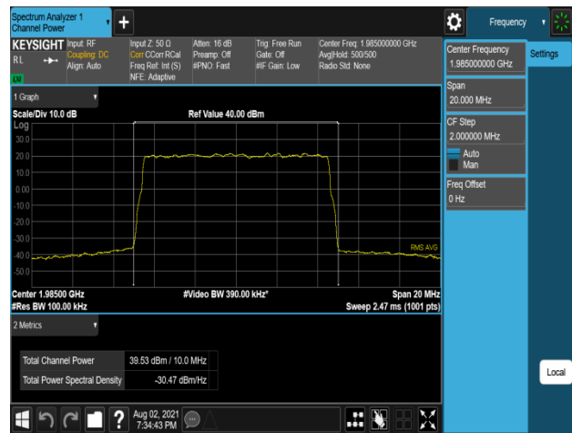
Plot 7-288. Conducted Average Output Power Plot (B2_10M_1C_16QAM – High Channel, Port 3)
