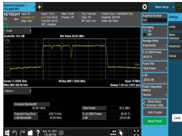
Plot 7-246. Occupied Bandwidth Plot (B66_5M+5M+5M+20M_4C_16QAM - Mid Channel, Port 0)
