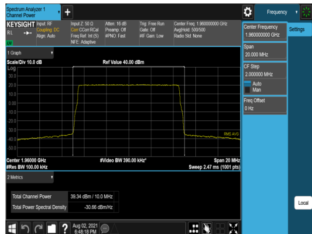
Plot 7-282. Conducted Average Output Power Plot (B2_10M_1C_256QAM - Mid Channel, Port 1)
