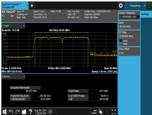
Plot 7-255. Occupied Bandwidth Plot (B66_5M+5M+10M+20M_4C_64QAM - Low Channel, Port 3)
