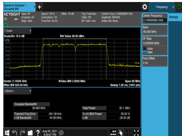
Plot 7-258. Occupied Bandwidth Plot (B66_5M+5M+10M+20M_4C_16QAM - Mid Channel, Port 3)
