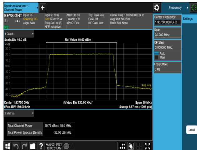
Plot 7-292. Conducted Average Output Power Plot (B2_15M_1C_QPSK - Low Channel, Port 3)
