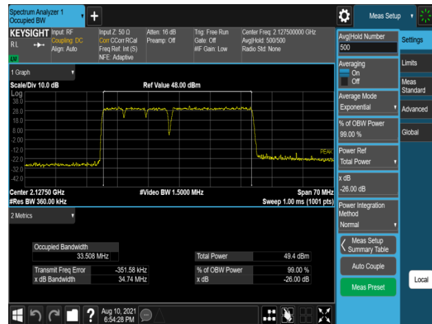
Plot 7-244. Occupied Bandwidth Plot (B66_5M+5M+5M+20M_4C_256QAM - Low Channel, Port 2)
