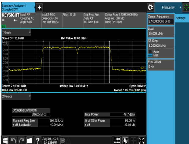
Plot 7-263. Occupied Bandwidth Plot (B66_5M+5M+10M+20M_4C_64QAM - High Channel, Port 3)
