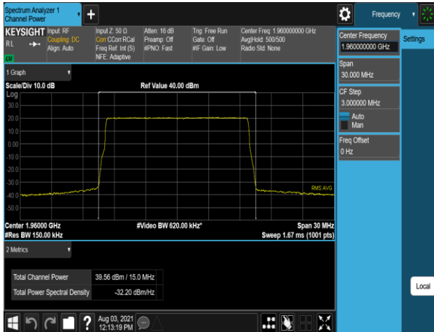
Plot 7-295. Conducted Average Output Power Plot (B2_15M_1C_64QAM - Mid Channel, Port 2)
