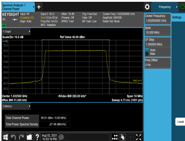
Plot 7-267. Conducted Average Output Power Plot (B2_5M_1C_64QAM - Low Channel, Port 2)
