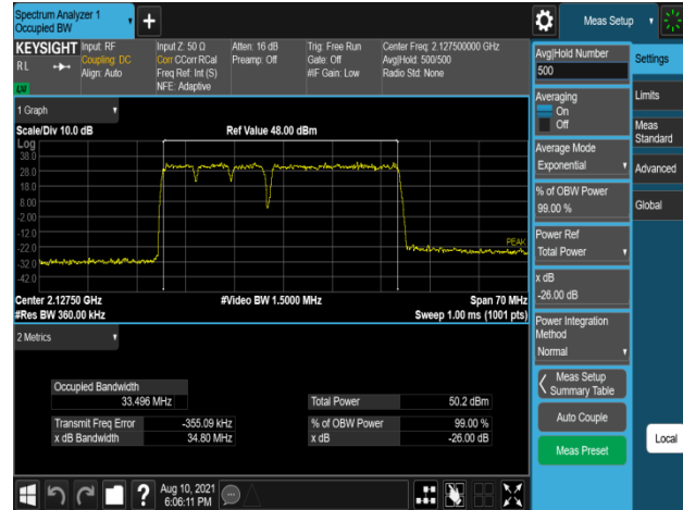
Plot 7-242. Occupied Bandwidth Plot (B66_5M+5M+5M+20M_4C_16QAM - Low Channel, Port 0)
