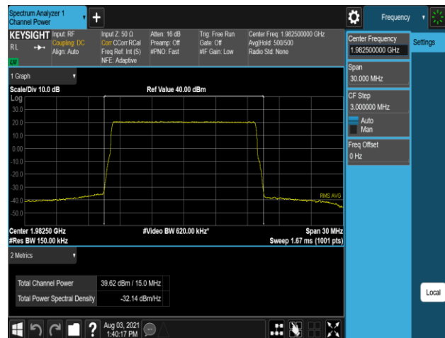
Plot 7-300. Conducted Average Output Power Plot (B2_15M_1C_64QAM - High Channel, Port 3)
