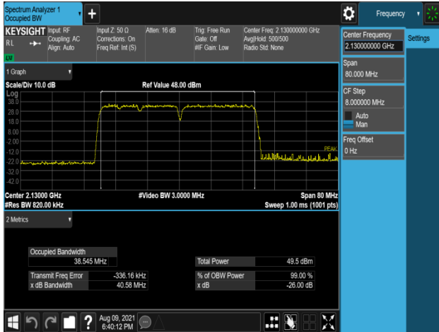
Plot 7-253. Occupied Bandwidth Plot (B66_5M+5M+10M+20M_4C_QPSK - Low Channel, Port 0)
