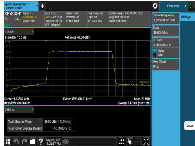
Plot 7-278. Conducted Average Output Power Plot (B2_10M_1C_256QAM - Low Channel, Port 1)
