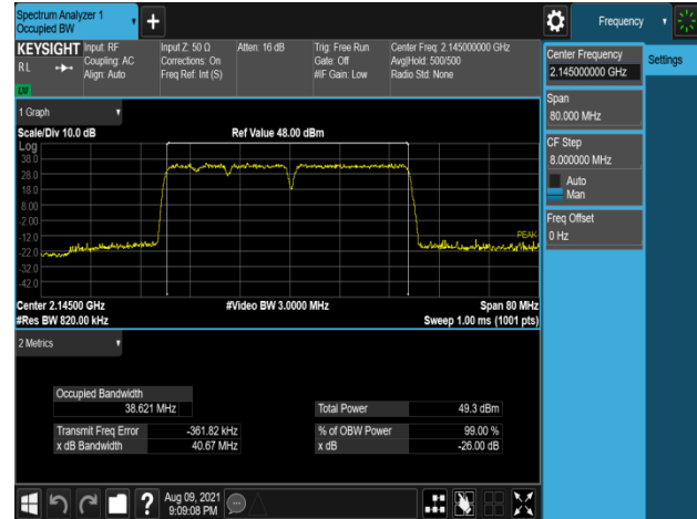
Plot 7-260. Occupied Bandwidth Plot (B66_5M+5M+10M+20M_4C_256QAM - Mid Channel, Port 1)
