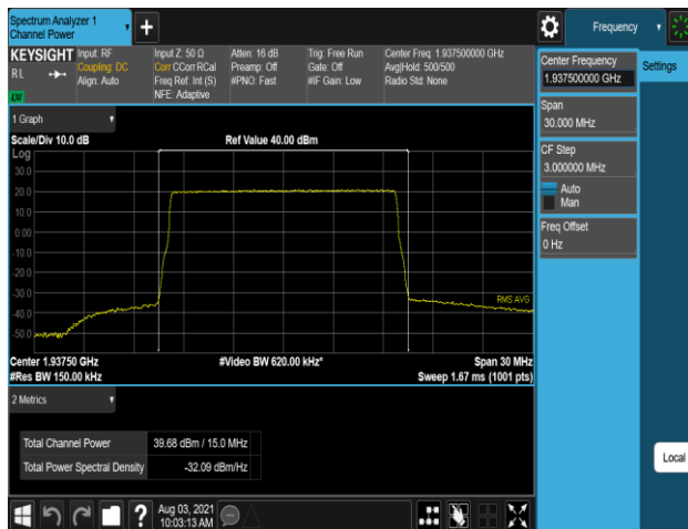
Plot 7-291. Conducted Average Output Power Plot (B2_15M_1C_QPSK - Low Channel, Port 2)
