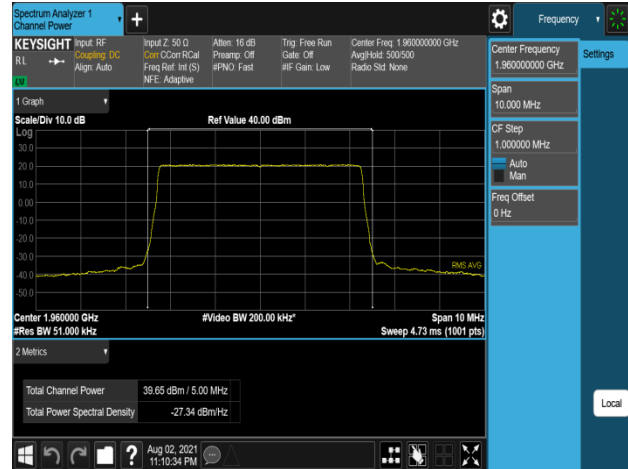
Plot 7-272. Conducted Average Output Power Plot (B2_5M_1C_QPSK - Mid Channel, Port 3)
