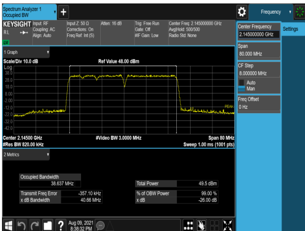
Plot 7-257. Occupied Bandwidth Plot (B66_5M+5M+10M+20M_4C_QPSK - Mid Channel, Port 2)
