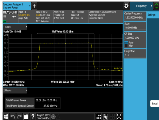
Plot 7-268. Conducted Average Output Power Plot (B2_5M_1C_64QAM - Low Channel, Port 3)
