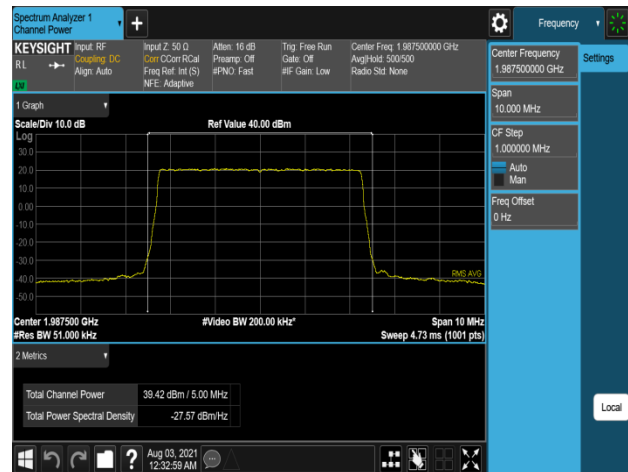
Plot 7-274. Conducted Average Output Power Plot (B2_5M_1C_256QAM - High Channel, Port 1)
