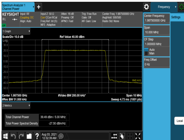
Plot 7-273. Conducted Average Output Power Plot (B2_5M_1C_256QAM - High Channel, Port 0)
