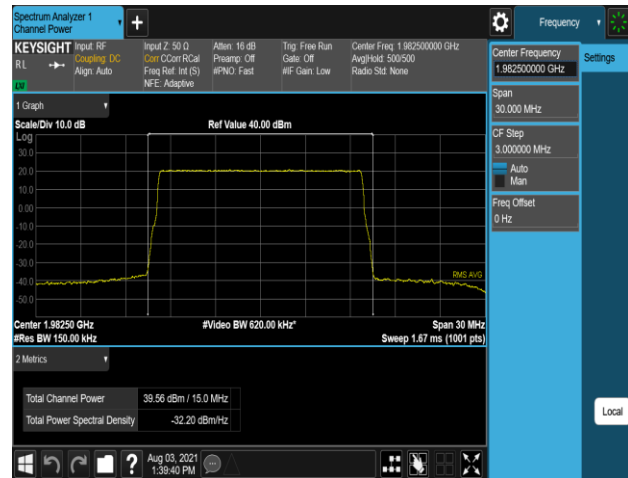
Plot 7-298. Conducted Average Output Power Plot (B2_15M_1C_64QAM - High Channel, Port 1)
