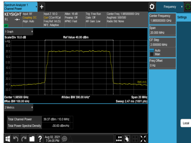
Plot 7-286. Conducted Average Output Power Plot (B2_10M_1C_16QAM – High Channel, Port 1)
