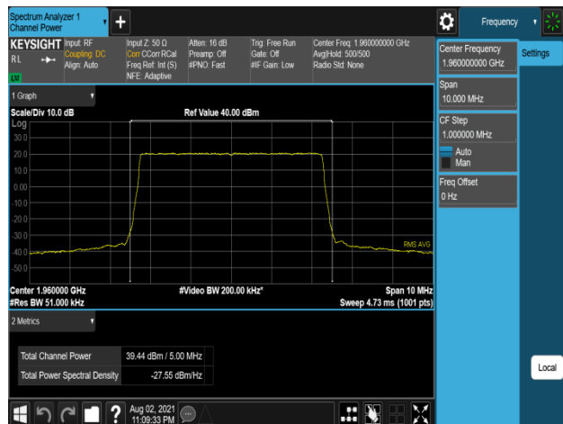
Plot 7-270. Conducted Average Output Power Plot (B2_5M_1C_QPSK - Mid Channel, Port 1)
