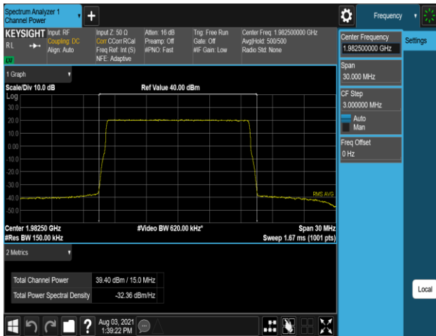
Plot 7-297. Conducted Average Output Power Plot (B2_15M_1C_64QAM - High Channel, Port 0)
