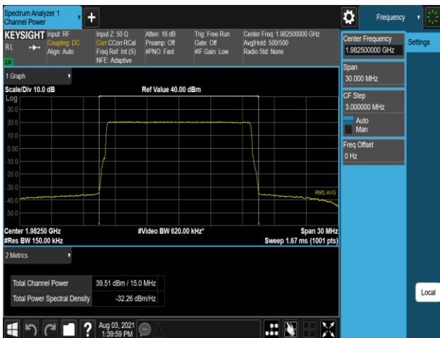
Plot 7-299. Conducted Average Output Power Plot (B2_15M_1C_64QAM - High Channel, Port 2)
