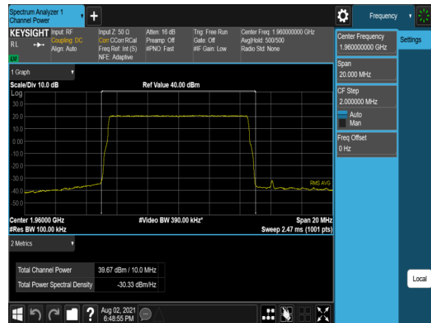
Plot 7-284. Conducted Average Output Power Plot (B2_10M_1C_256QAM – Mid Channel, Port 3)
