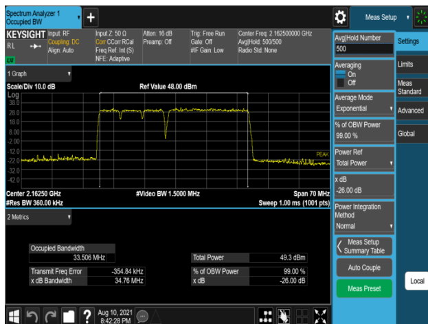
Plot 7-249. Occupied Bandwidth Plot (B66_5M+5M+5M+20M_4C_QPSK - High Channel, Port 1)
