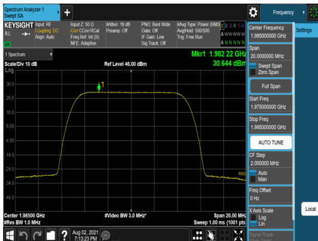
Plot 7-551. Peak Power Spectral Density Plot (B2_10M_1C_QPSK - High Channel, Port 2)
