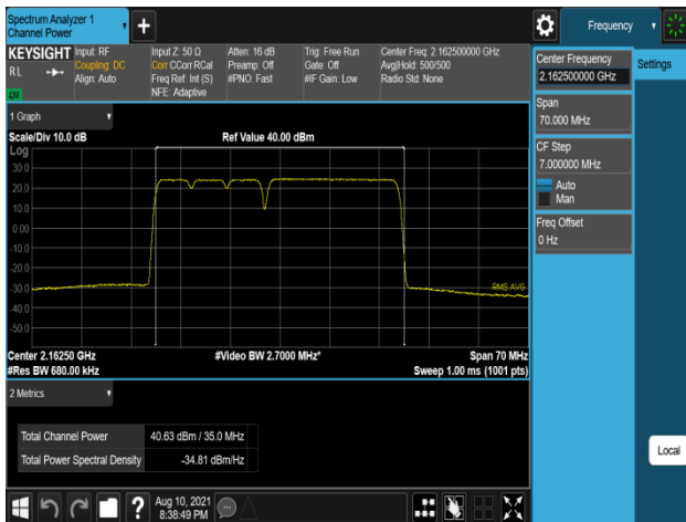
Plot 7-513. Conducted Average Output Power Plot (B66_5M+5M+5M+20M_4C_QPSK – High Channel, Port 0)
