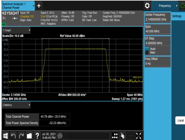
Plot 7-415. Conducted Average Output Power Plot (B66_20M_1C_64QAM - Mid Channel, Port 2)
