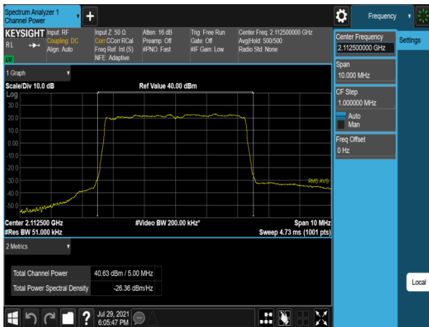
Plot 7-375. Conducted Average Output Power Plot (B66_5M_1C_16QAM - Low Channel, Port 2)
