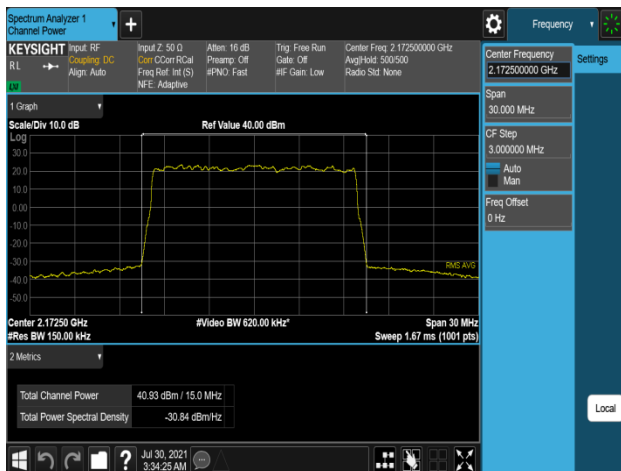
Plot 7-407. Conducted Average Output Power Plot (B66_15M_1C_16QAM – High Channel, Port 2)
