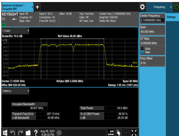
Plot 7-257. Occupied Bandwidth Plot (B66_5M+5M+10M+20M_4C_QPSK - Mid Channel, Port 2)
