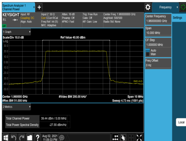
Plot 7-269. Conducted Average Output Power Plot (B2_5M_1C_QPSK - Mid Channel, Port 0)
