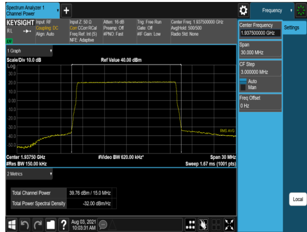
Plot 7-292. Conducted Average Output Power Plot (B2_15M_1C_QPSK - Low Channel, Port 3)
