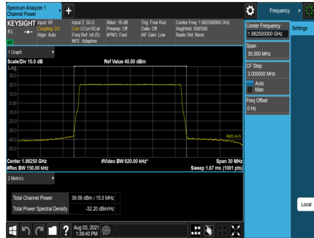
Plot 7-298. Conducted Average Output Power Plot (B2_15M_1C_64QAM - High Channel, Port 1)
