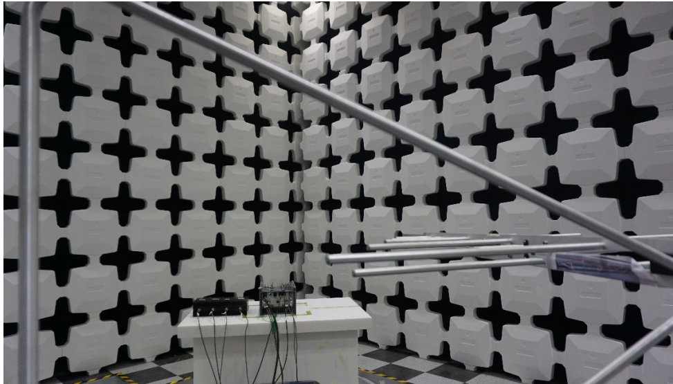
2. Radiated Measurement (Above 1GHz) Photo
